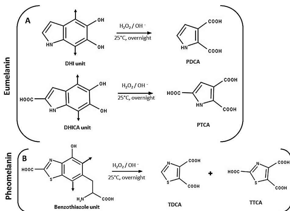
Figure 1. Eumelanin and pheomelanin markers obtained by alkaline peroxide oxidation. A) Peroxide oxidation of DHI and DHICA moieties of EM produces PDCA and PTCA markers respectively. B) Oxidation of the benzothiazole unit of PM yields TTCA and TDCA markers.
