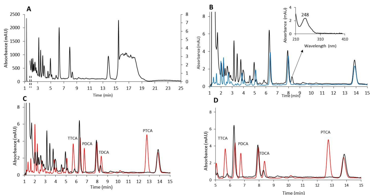
Figure 3. Chromatograms obtained by RP-HPLC-DAD (Column: Gemini C18, 150 x 3 mm, 3 \mu\text{m} particle size, 100 \text{\AA} pore size, Phenomenex) of A375 non-pigmented cells. A) crude sample before SPE method. A break was introduced in the x-axis and note the differences in y-axis scales. B) overlay of a crude sample before and after SPE. C) overlay of a crude sample before SPE and a spiked sample with a mixture of four markers (at a concentration of 1 \mu\text{g}/\text{mL} ) after SPE. D) zoom of chromatogram C that shows the zone of interest between 5 and 15 min of analysis.
