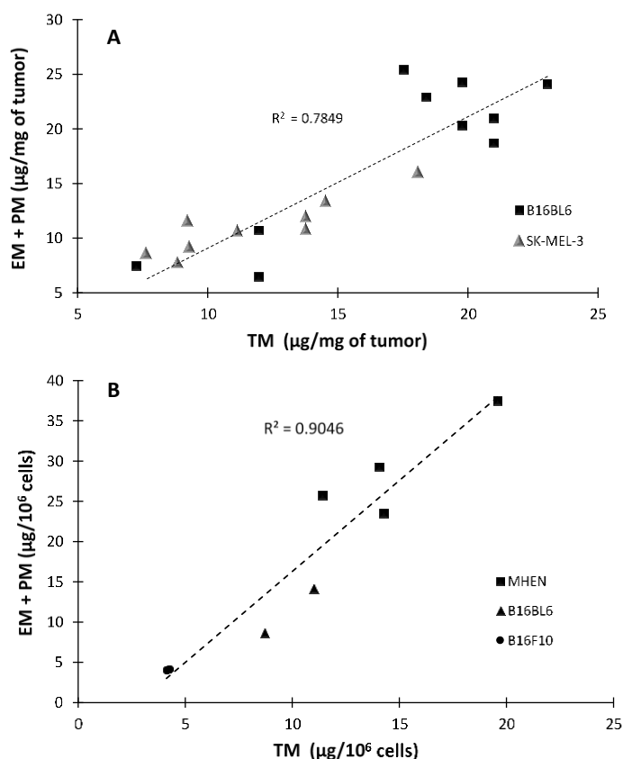
Figure 6. Correlation between total melanin obtained by chemical degradation method followed by SPE and HPLC analysis (eumelanin EM, and pheomelanin PM) versus total melanin (TM) content after potassium hydroxide solubilisation measured at 405nm. A) Melanoma tumors B16BL6 ( n=10 ) and human melanoma tumors SK-MEL-3 ( n=10 ); B) murine melanoma cells B16BL6 ( n=2 ), B16F10 ( n=2 ) and human melanocytes ( n=4 ). Correlation are significant at P < 0.0001 .
