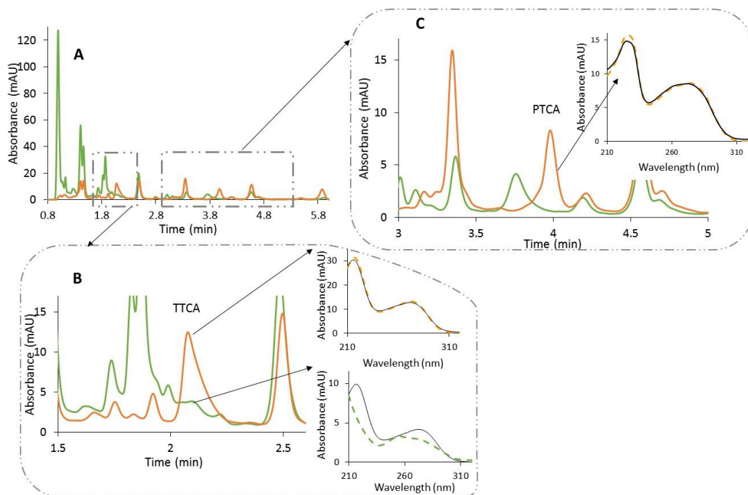
Figure 4. Chromatograms of SK-MEL-3 tumor obtained by RP-HPLC-DAD (column: Kinetex Evo C18, 150 x 3 mm, 2.6 \mu m particle size, 100 A pore size from Phenomenex ) after SPE: ___ fraction obtained during sample loading, ___ Elution-fraction, ___ UV spectrum of standards, ___ UV spectrum of the sample. A) Chromatograms between 0 and 6 min of analysis corresponding to maximum elution time of melanin markers B) Zoom between 1.5 and 3 min corresponding to the TTCA elution zone C) Zoom between 3 and 5 min of analysis corresponding to the PTCA elution zone.
