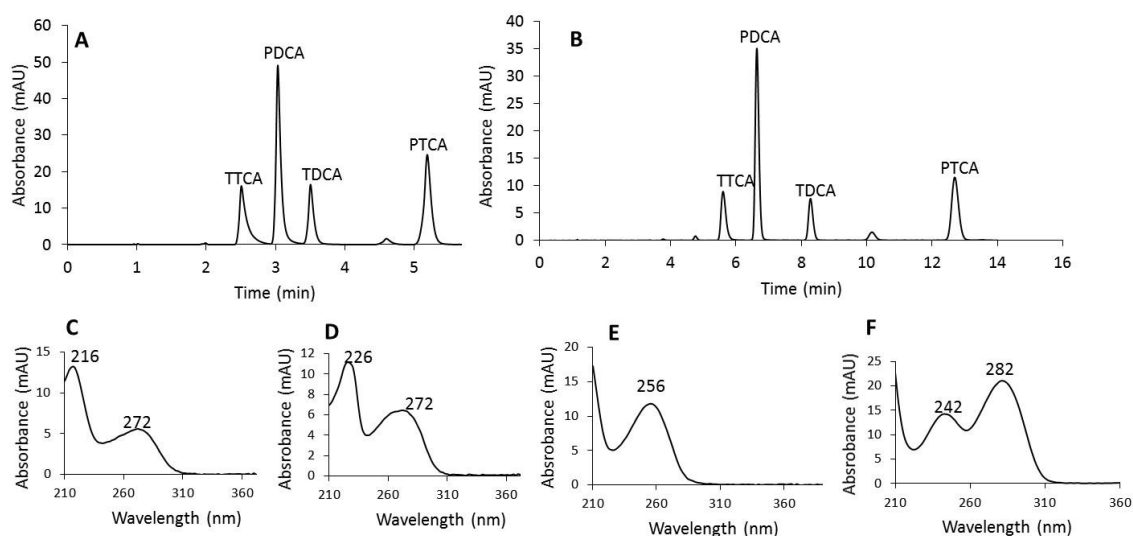
Figure 2. RP-HPLC-DAD chromatograms of a mixture of four melanin markers (10 \mu g/mL) obtained with 20mM phosphate pH 3.3 as mobile phase at 0.6 mL/min, 36°C, signal detected at 275nm and 5 \mu L injection volume. A) Column: Kinetex Evo C18, 150 x 3 mm, 2.6 \mu m particle size, 100 Å pore size from Phenomenex B) Column: Gemini C18, 150 x 3 mm, 3 \mu m particle size, 100 Å pore size, Phenomenex C) TTCA UV- spectrum D) PTCA UV- spectrum E) TDCA UV- spectrum and F) PDCA UV- spectrum
