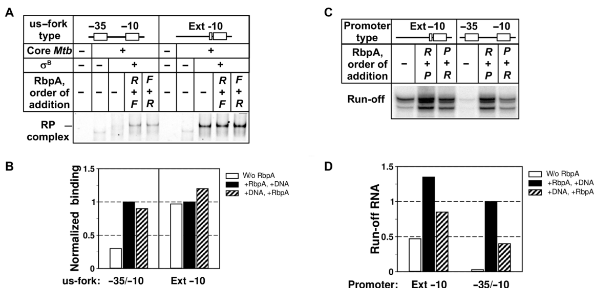
Fig. 4. Effect of promoter architecture on Mtb RNAP activity. (A) Native gel electrophoresis analysis of the Mtb RNAP complex formation with Cy3-labeled us-fork and us-fork harboring extended -10 element (Ext -10). RbpA was added either before (R + F) or after (F + R) the us-fork DNA. (B) Quantification of the gel shown in (A). Values were normalized to that obtained in the presence of RbpA for each template separately. (C) Run-off [ ^{32} P]RNA products synthesized in multiple-round transcription from the wild-type sigAP promoter and its derivative harboring extended -10 element. (D) Quantification of the RNA products shown in (C). Values were normalized to that obtained for the wild-type sigAP promoter in the presence of RbpA. RbpA was added either before (R + P) or after (P + R) the promoter DNA.
