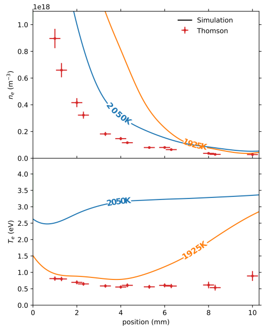
Figure 6. Comparison between electron properties obtained from the simulation (at two different emitter temperatures) and in scattering experiments, for a cathode discharge current of 8 A and flow rate of 0.8 mg/s.
