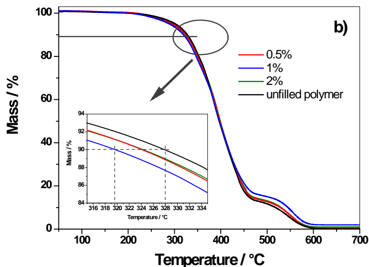
Figure 10: Thermal stability of different nanocomposites synthesized with 0.5, 1 and 2 % of PS sepiolite and dispersed by a) US or b) UT route. Insert: T_{10\%} zoom. An unfilled polymer is added for comparison.
