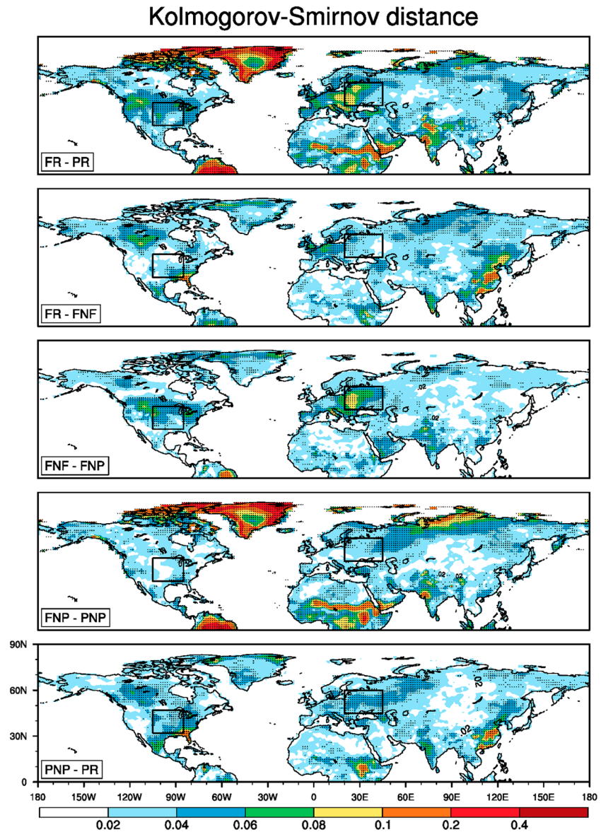
Figure 3. Northern Hemisphere distribution of the Kolmogorov-Smirnov (KS) statistics, which quantifies the distance between pairs of empirical distributions of daily summer T_{max} . Stippling denotes grid cells where the distance is statistically significant at the 95% level using a two-sided two-sample KS test. Note that all distributions have been centered (i.e., the summer mean T_{max} has been removed) in order to focus on the shape of the distribution.
