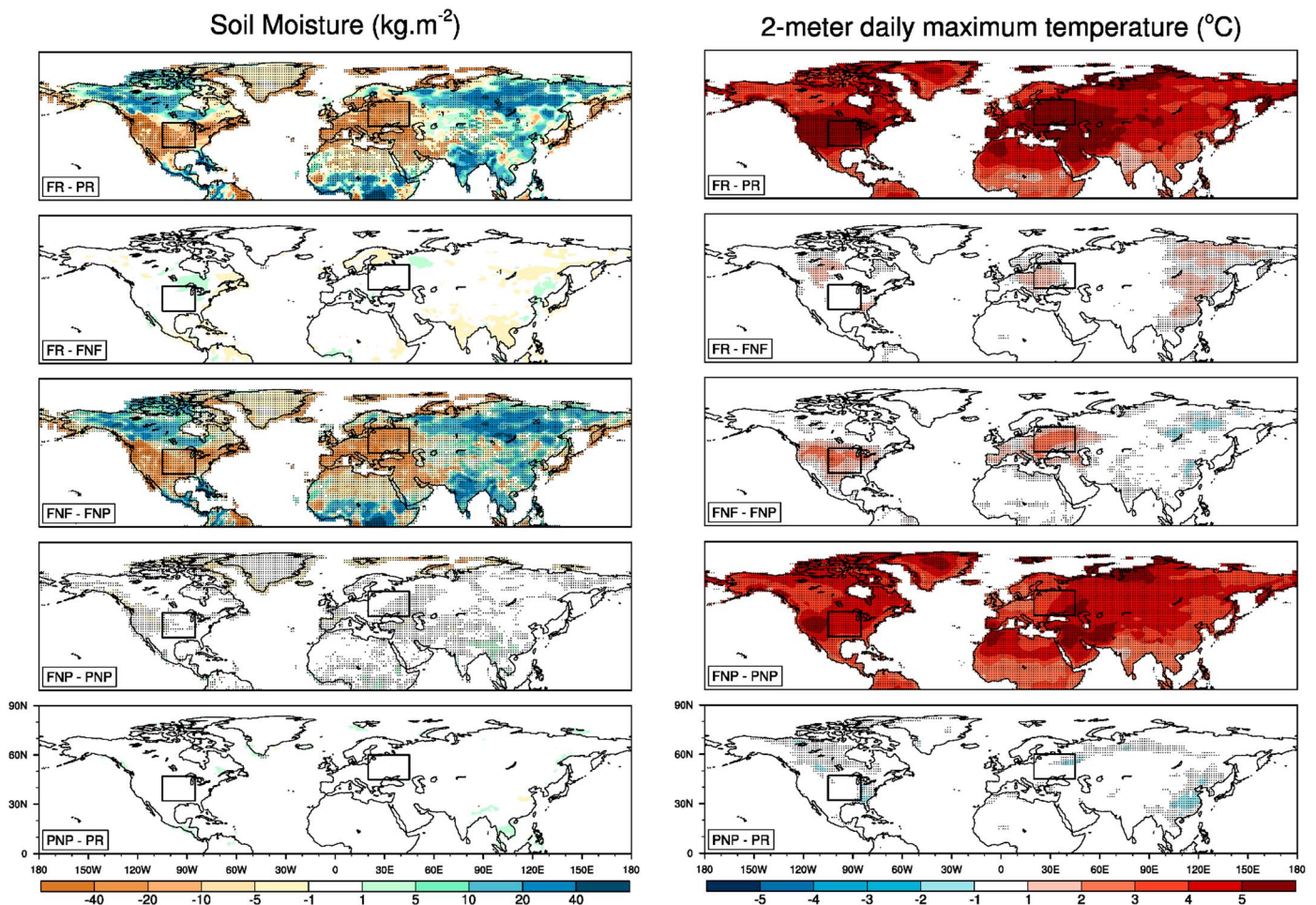
Figure 1. Northern Hemisphere breakdown of (left column) summer mean soil moisture ( \text{kg}\cdot\text{m}^{-2} ) and (right column) daily T_{\text{max}} (K) anomalies projected in the reference climate change experiments (FR-PR) into four contributions: nudging in future climate (FR-FNF), soil moisture feedback (FNF-FNP), climate change without soil moisture feedback (FNP-PNP), and nudging in present-day climate (PNP-PR). Stippling denotes grid cells where anomalies are statistically significant at the 95% level based on a two-sided t test. Black rectangles denote the central U.S. and eastern Europe domains selected for a regional analysis of the temperature distribution.
