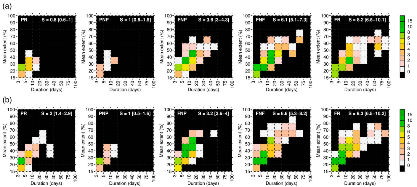
Figure 4. Joint pdfs of heat wave duration and mean extent for all 30 year simulations (PR, PNP, FNP, FNF, and FR from left to right) over (a) central U.S. and (b) eastern Europe. In each panel, S denotes the mean heat wave severity with the bootstrapped 5–95% confidence interval in brackets. All severity values have been normalized relative to the mean severity estimated in PNP.
