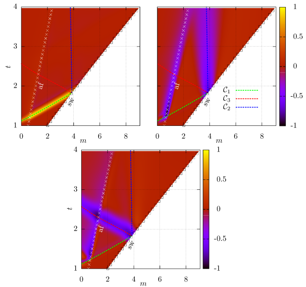
Figure 2: W_1 (left), W_2 (right) and W_3 (bottom).
