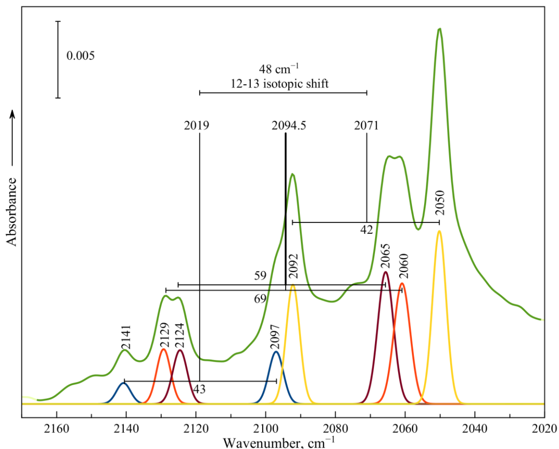
Figure 8. FTIR spectrum of 72% 13 CO+28% 12 CO mixture adsorbed on Ni10/H-USY after pumping for 15 min in the cooled cell with subsequent addition of 0.1 Torr of He at 77 K; and the result of its deconvolution.
