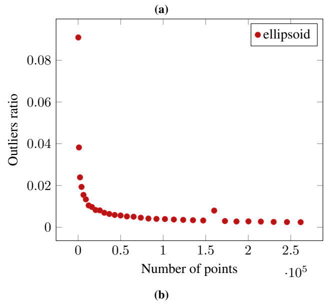
Figure 7: Percentage of outliers per total number of points. (7a) for the sphere and (7b) for the ellipsoid
