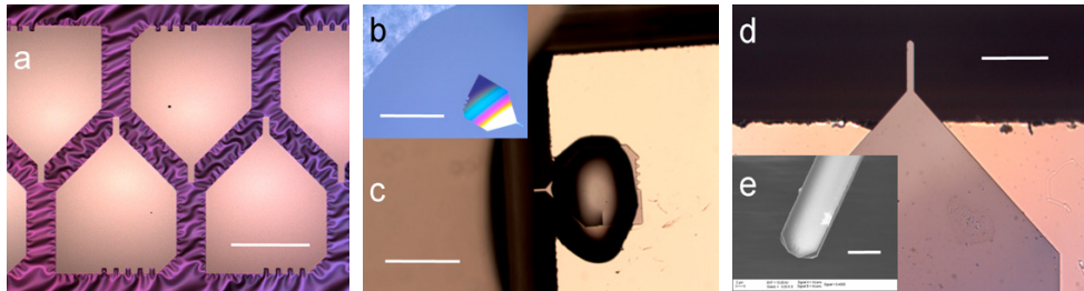
Fig. 1 Patch technology: (a) fabrication of 3 μm thick GaAs mesa "patches", scale bar = 300 μm (b) patch recuperation and storage in isopropanol, the optical microscope image shows an individual GaAs patch suspended in a water droplet, scale bar = 600 μm (c) fluidic assembling of a GaAs patch onto a pre-diced and metallized (Ti/Au/Pt/Ti/Pt) fused silica support wafer using capillary forces, scale bar = 400 μm (d) a GaAs microcantilever protruding over the edge of the fused silica support wafer (chip dimensions = 0.75×2×4 mm) following drying and ohmic contact formation (400°C/40s), scale bar = 100 μm and (e) a scanning electron microscopy image of the tip of the GaAs microcantilever showing the crystal planes and sharp corners exposed by the wet etching ( \text{NH}_4\text{OH}/\text{H}_2\text{O}_2/\text{H}_2\text{O} ) in (a), scale bar = 10 μm.
