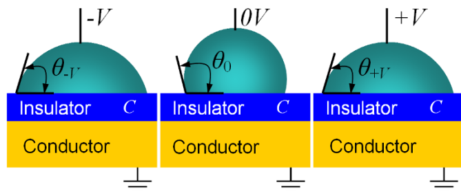
Figure 1 | Electrowetting behaviour for the liquid-insulator-conductor system. The variation of the contact angle of the droplet is symmetrical with the applied voltage polarity, \theta_{-V} = \theta_{+V} , and obeys the Young-Lippmann equation. The capacitance of the insulating layer is C \text{ Fm}^{-2} ; the conductor is considered to be perfect; the liquid is considered to be conducting.
