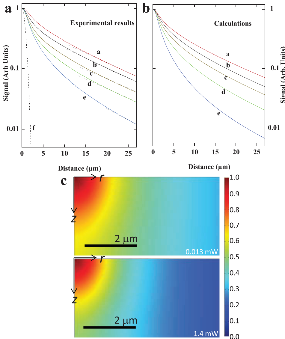
FIG. 2. (a) The normalized luminescence cross section for a light excitation power of 0.013 mW, 0.096 mW, 0.24 mW, 0.49 mW, and 1.4 mW (curves (a) to (e), respectively). Curve f is the laser profile. (b) Self consistent calculations under the same conditions. In both cases, the shape of the profile at low power and large r yields a diffusion length of 21.5 \mu\text{m} . The effect of an increase of light intensity is to decrease the diffusion length near r = 0 due to ambipolar diffusion, while the slope of the logarithmic plot remains practically unchanged at large r where u = n/N_A is small. (c) Calculated spatial dependence of the normalized electronic concentration. The top frame shows the low power case (curve a of the right panel), while the bottom frame shows the high power case (curve e of the right panel).
