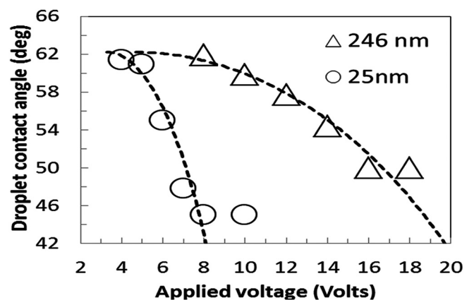
FIG. 4. Electrowetting of a droplet of the bubble solution on the Tefflon ® coated silicon surfaces (25 nm and 246 nm). The dashed lines are solutions of the Young-Lippmann equation. 2
