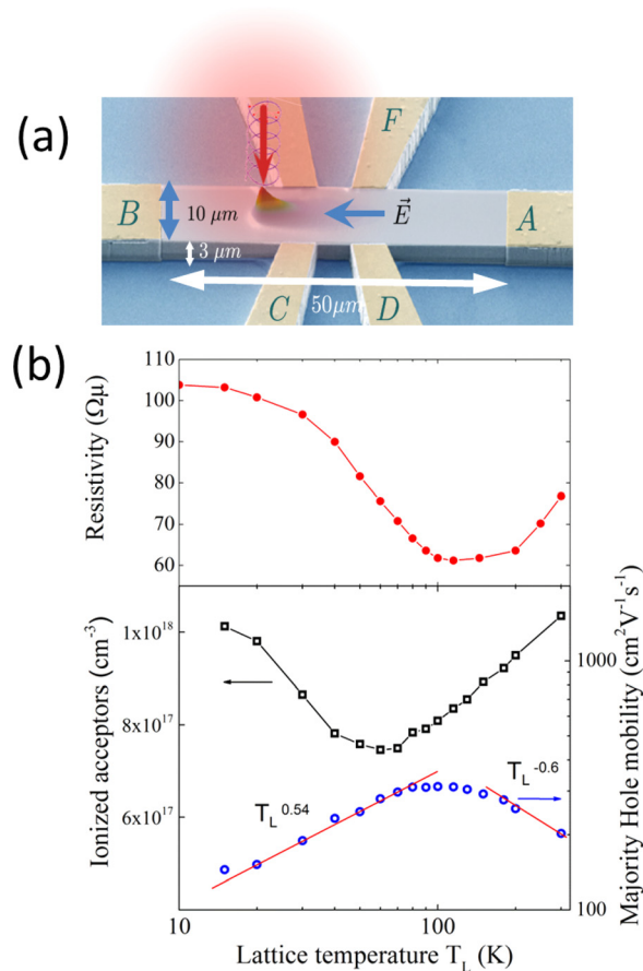
FIG. 1. (a) SEM image of the p -GaAs hall bar used to study both minority and majority carrier transport. Also shown is a 3D representation of a measured electron density profile when an electric field is applied. (b) Dependence as a function of lattice temperature of the resistivity (plain circles), the concentration of ionized acceptors (open squares), and their mobility (open circles).
