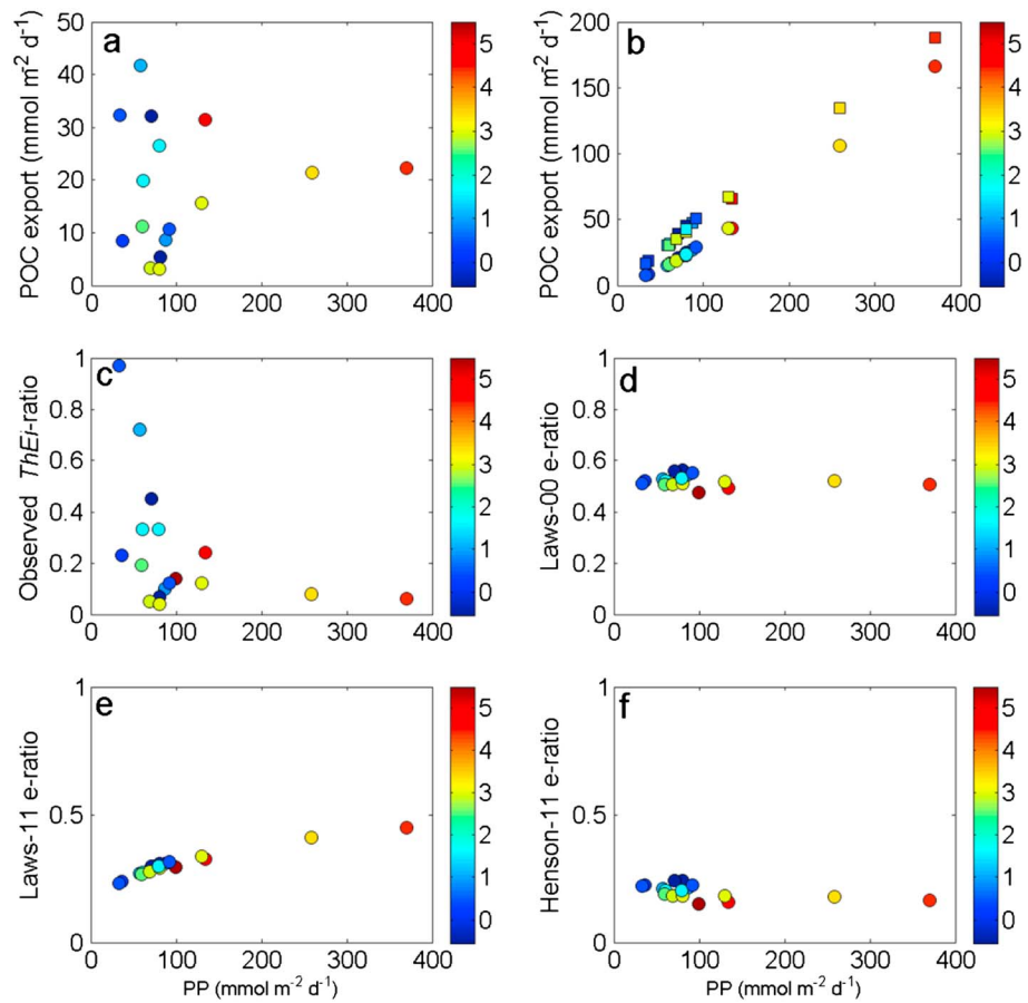
Figure 2. Scatterplot of POC export and primary production based on (a) our observations and (b) algorithms of Laws et al. [2000] (squares) and Laws [2011] (circles). Scatterplot of e ratio and primary production based on (c) observed ThE_i ratio and e ratio derived (d) from Laws et al. [2000] (Laws-00), (e) from Laws [2011] (Laws-11), and (f) from Henson et al. [2011] (Henson-11) algorithms. The color bar represents sea surface temperature ( ^{\circ}\text{C} ).
