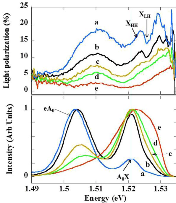
FIG. 4. The bottom panel shows the normalized local luminescence spectra at 15 K for an excitation power equal to 0.21 \mu W (a), 24 \mu W (b), 0.11 mW (c), 0.35 mW (d), and 2.18 mW (e) and reveals the cross-over between a low power regime where the eA_0 recombination is dominant to a high power one, where the BB emission prevails. The top panel shows the spectra of the luminescence degree of circular polarization in the same conditions and reveals a decrease of polarization in the high-power regime.
