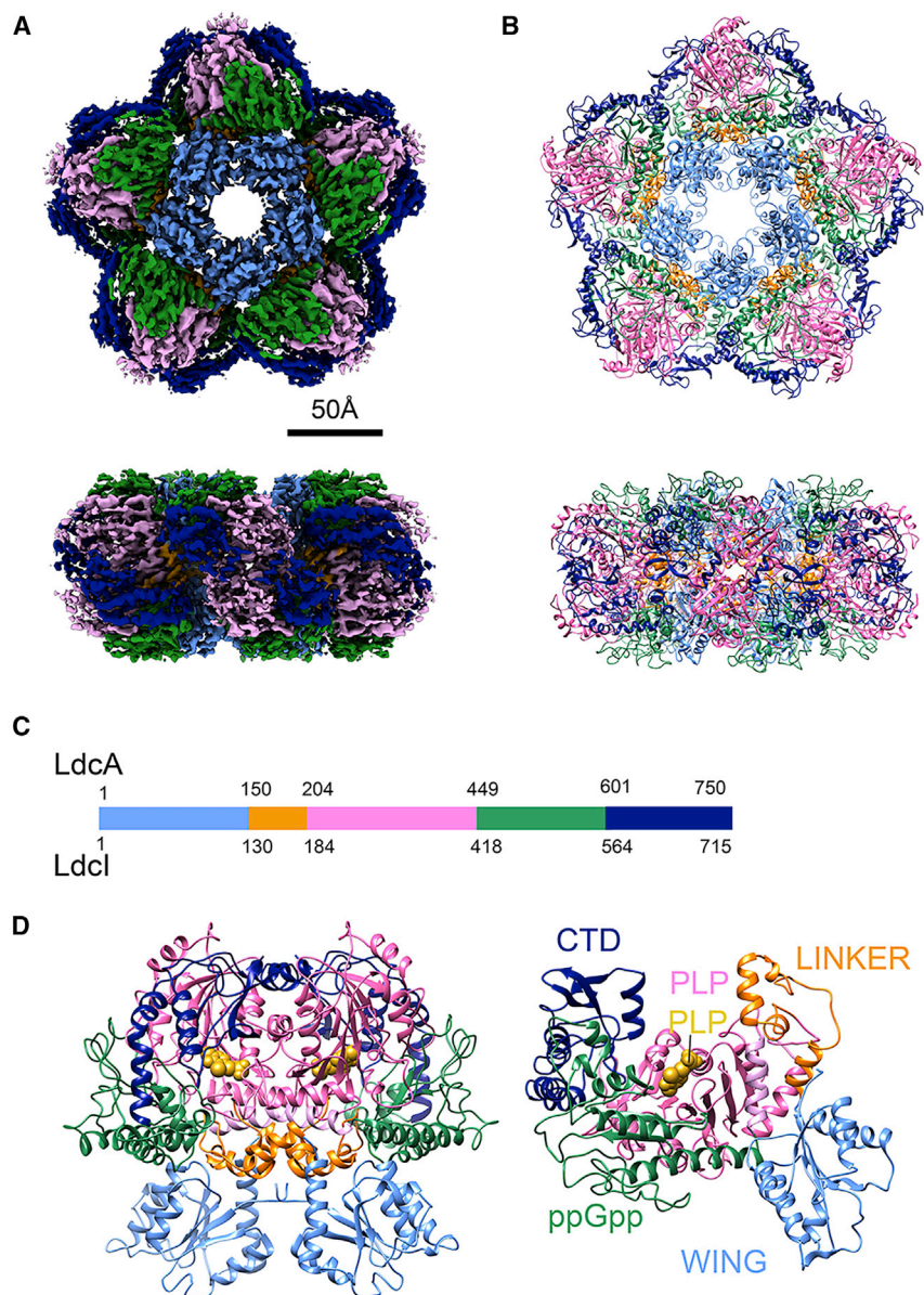
Figure 1. Cryo-EM Map and Near-Atomic Model of LdcA
