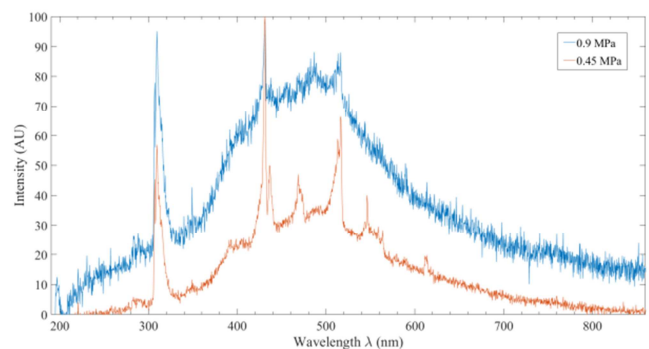
Fig. 3. Emission spectra of the LOX/CH 4 flame.
