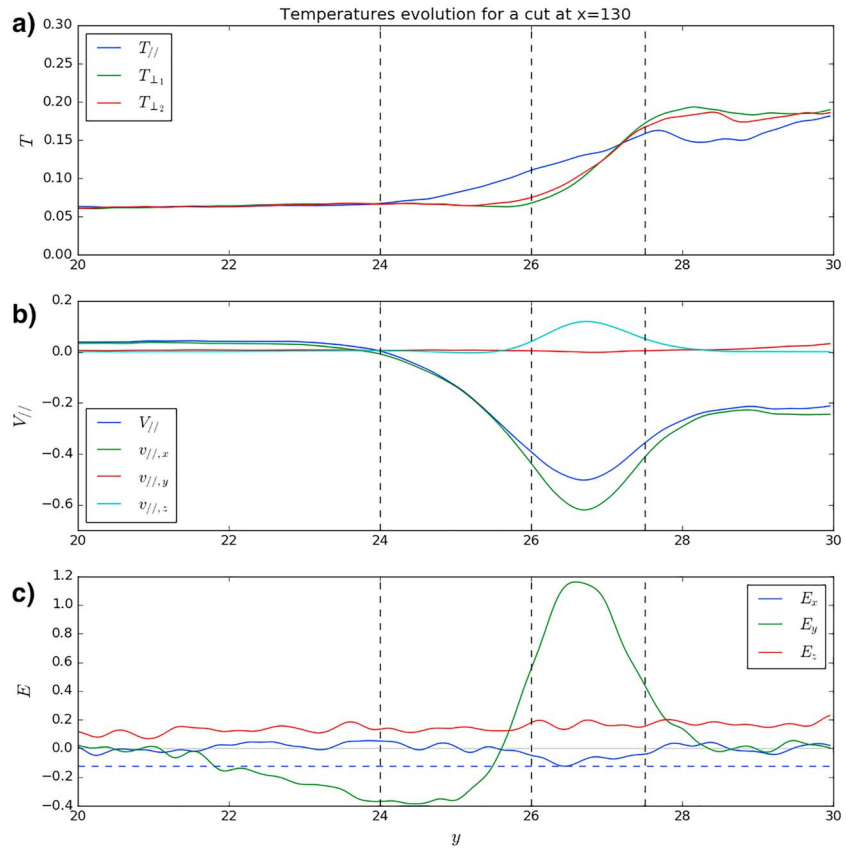
Figure 9. Components of the cold ion temperature, cold ion parallel velocity, and electric field for a cut at x = 130 and t = 120 . (a) Diagonal components of the temperature tensor in the ( // , \perp_1 , \perp_2 ) frame. (b) Mean velocity of cold ions in the direction parallel to the magnetic field and its projection upon x , y , and z directions. (c) Electric field components. A dashed blue line show the minimum value of E_x . Vertical dashed lines are plotted for y = 24 , 26 , and 27.5 in order to roughly show the area where the heating is only parallel (for 24 < y < 26 ) and the position of the Hall electric field peak (for 26 < y < 27.5 ).
