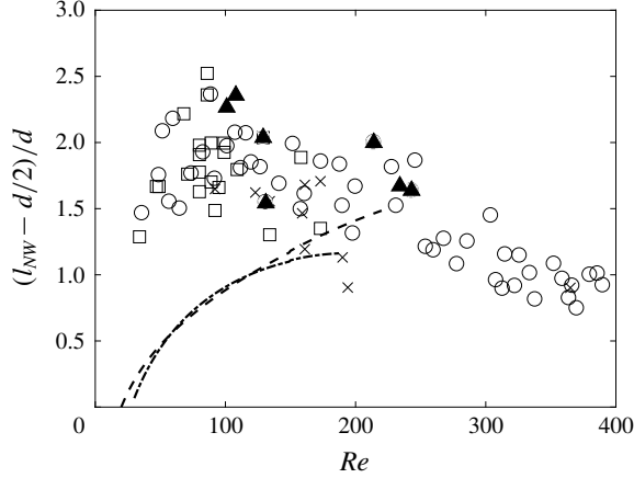
FIGURE 18. Non-dimensional near-wake chord length versus Re . Partially contaminated bubbles, \times , Ro < 6 ; \circ , 6 \leq Ro \leq 8.5 ; \square , Ro > 8.5 . Fully contaminated bubbles, \blacktriangle . Dashed line, Giacobello et al. (2009) and Tomboulides and Orszag (2000); dash-dotted line, Nakamura (1976).
