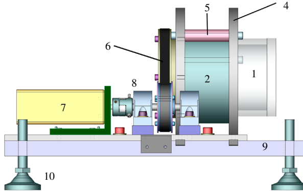
FIGURE 23. Lateral view of the device.
