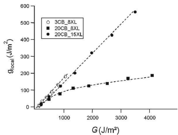
FIGURE 10 g_{\text{local}} as a function of G for the three studied elastomers. ■: 20CB_8XL; ○: 3CB_8XL; ●: 20CB_15XL.
