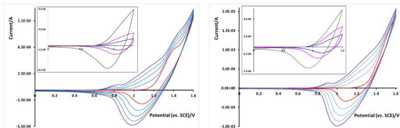
Figure 3. Electrochemical polymerization of TPM3 (left) and TPM4 (right) by cyclic voltammetry between 0 and 1.6 V/SCE in 1.5 \cdot 10^{-3} mol \text{L}^{-1} monomer + 0.1 mol \text{L}^{-1} ( n\text{-Bu}_4\text{N} ) [\text{PF}_6] \text{CH}_2\text{Cl}_2 solution onto ITO electrode. Scan rate = 0.1 \text{V} \cdot \text{s}^{-1} . Red = 1 st cycle, blue = 2 nd -4 th cycles, purple: 5 th cycle. Inserts = electroactivity in \text{CH}_2\text{Cl}_2 of the formed films at 50 (blue), 100 (red), 500 \text{mV/s} (green).
