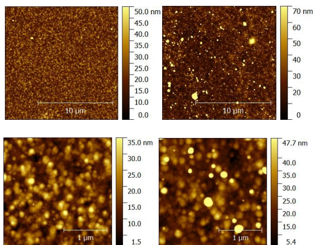
Figure 5. AFM surface topography of e-TTP3 (left) and e-TTP4 (right) thin films deposited by cyclic voltammetry on ITO/glass electrodes. Examined areas: 15 \times 15 \mu\text{m} (top), 2.5 \mu\text{m} (bottom).
