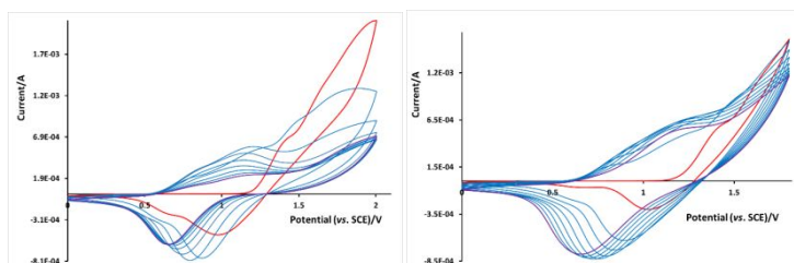
Figure 2. Electrosynthesis of e-TPP3 1.5 \cdot 10^{-3} \text{ mol L}^{-1} in \text{CH}_2\text{Cl}_2 + 0.1 \text{ mol L}^{-1} (n\text{-Bu}_4\text{N})[\text{PF}_6] using cyclic voltammetry between 0 and (left) 2.0 and (right) 1.8V/SCE on ITO electrode (10 cycles). Scan rate = 0.1 \text{ V.s}^{-1} . The first cycle is plotted in red, the intermediates in blue, and the 10 th in purple.
