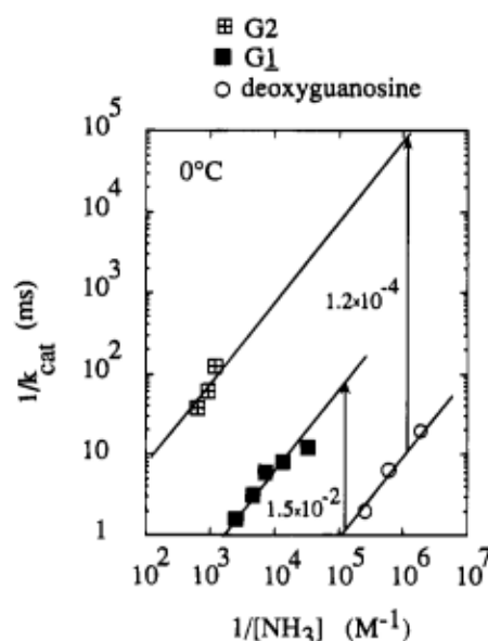
FIGURE 2: The contribution of ammonia to the exchange rate of the imino proton of G_1 and G_2 of the d(CGCGATCGCG) duplex and of deoxyguanosine. Conditions: NaCl, 200 mM; EDTA, 1 mM; 0^\circ C .
