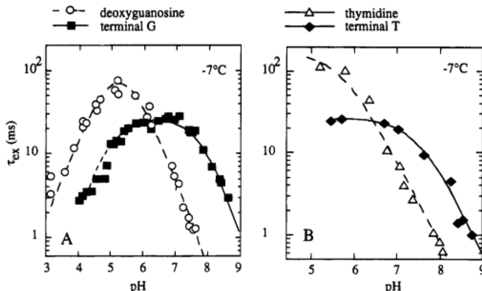
FIGURE 1: (A) Exchange time of the imino proton of the terminal G ( G_1 , opposite C_1 ) of the d(CGCGATCGCG) duplex and of deoxyguanosine vs pH. At high pH, when catalysis by OH^- dominates, the exchange time of the terminal pair is larger than that of deoxyguanosine. At lower pH, exchange is catalyzed by the intrinsic catalyst in the case of the terminal pair and by water in the case of deoxyguanosine. Conditions: NaCl, 200 mM; EDTA, 1 mM; -7^\circ C . The pH scale is inaccurate. (B) Exchange time of the imino proton of the terminal T of the d(TAGCGCTA) duplex and of thymidine vs pH. Same conditions as in (A) except NaCl, 100 mM.
