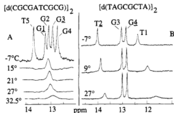
FIGURE 3: (A) Shift of the imino proton resonance of G1 of the d(CGCGATCGCG) 2 duplex vs temperature. The resonance is in a fast-exchange situation between the positions corresponding to closed and open pairs. Exchange with water produces broadening but no shift. In all spectra except for the -7^{\circ}\text{C} spectrum, all imino protons are saturated, except for the terminal one, which is therefore observable without interference, as described in Materials and Methods. The short acquisition time and Hamming filtering produce an instrumental broadening which is most simply determined by the line width of the methyl proton (not shown). The broadening assigned to exchange with water is 33, 40, 47, and 97 Hz at 15, 21, 27, and 32.5^{\circ}\text{C} , respectively. Conditions: NaCl, 200 mM; EDTA, 1 mM; chemical shift reference, NMe 4 Cl, 0.2 mM; pH 6.86 (measured at 20^{\circ}\text{C} ); 0^{\circ}\text{C} . (B) The imino proton spectrum of the d(TAGCGCTA) 2 duplex vs temperature, displaying the shift and broadening of the first and second thymidines. Conditions: NaCl, 100 mM; EDTA, 1 mM; chemical shift reference, NMe 4 Cl, 0.2 mM; pH 5.6 (measured at 20^{\circ}\text{C} ); 0^{\circ}\text{C} .
