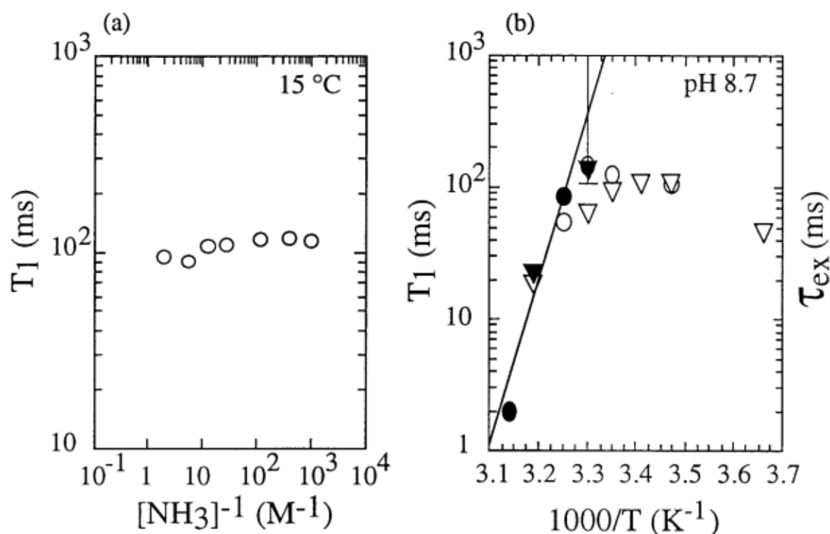
Figure 6. (a). The longitudinal relaxation time T_1 of the sugar 2'-OH proton of G34 as a function of the inverse of ammonia concentration in the AMP-RNA aptamer complex at 15^\circ\text{C} . The T_1 values are independent of the ammonia concentration up to 0.5 M. (b) The longitudinal relaxation times T_1 (open symbols) and exchange times (filled symbols) of the sugar 2'-OH proton of G34 as a function of temperature at pH 8.7 in the absence (triangles) and in the presence (circles) of 12 mM ammonia. The relaxation is governed by dipolar processes around 15^\circ\text{C} and by chemical exchange contributions at higher temperatures. At high temperature T_1 is equal to \tau_{\text{ex}} . An extrapolation of the exchange times measured at high temperature yields a \tau_{\text{ex}} of about 20 seconds at 15^\circ\text{C} and one second at 25^\circ\text{C} . The same result is obtained, based on the computation of \tau_{\text{ex}} from T_1 assuming a dipolar contribution of 120 ms between 15 and 20^\circ\text{C} .
