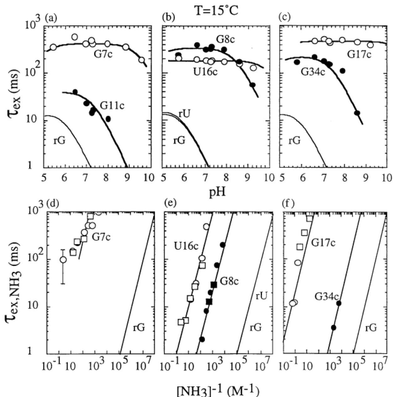
Figure 5. Exchange times of imino protons in the ATP-binding asymmetric internal loop in the AMP-RNA aptamer complex as a function of pH and ammonia at 15^\circ\text{C} . The corresponding curves describing exchange times in the ribonucleoside monomers under the same conditions are reported in the plots. The pH dependence of the exchange times of: (a) the G7 and G11 imino protons, (b) the G8 and U16 imino protons and (c) the G17 and G34 imino protons in the complex. Exchange times of all imino protons except G11 (for which the data are marginal to reach conclusions) display the pH-independent feature characteristic of intrinsic catalysis. The apparent dissociation constants of base-pairs involving the imino protons of G7, U16 and G17 are too low to be derived from the hydroxide catalysis data. The dependence on the inverse of the ammonia concentration of: (d) the G7 imino proton, (e) the G8 and U16 imino protons and (f) the G17 and G34 imino protons in the complex. Circles and squares relate to data collected with one and four equivalents of AMP bound per RNA aptamer, respectively. The same \alpha K_d(\text{NH}_3) values are observed for both ratios of AMP in the complex.
