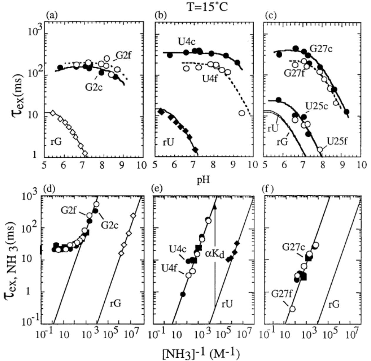
Figure 3. Exchange times of the imino protons in the stem (G2 and U4) and UUCG hairpin loop (G27 and U25) segments in the free RNA aptamer (designated by f) and the AMP–RNA aptamer complex (designated by c) as a function of pH and ammonia at 15°C. The corresponding exchange times in the ribonucleoside monomers under the same conditions are represented by diamonds. The pH dependence of the exchange times of: (a) the G2, (b) the U4 and (c) the G27 and U25 imino protons in the free RNA duplex and the complex. The exchange times are analyzed in term of three exchange processes: the hydroxyl catalysis \text{NOH}^- at high pH, the intrinsic catalysis from the neutral hydrogen bond acceptor at the pH-independent plateau and the intrinsic catalysis from the \text{N}^7 -protonated guanosine for G·C base-pairs under pH 6. The curves are fitted according to equation (11) with the \alpha K_d values listed in Tables 1 and 2, the \text{p}K values given in Theory and the following collision and pseudo-collision constants measured on the monomer using equations (3) and (4): for rU, q_{\text{OH}^-} = 6 \times 10^9 \text{ s}^{-1} \text{ M}^{-1} and q_{\text{H}_2\text{O}} = 1.5 \times 10^{11} \text{ s}^{-1} ; for rG, q_{\text{OH}^-} = 6.5 \times 10^9 \text{ s}^{-1} \text{ M}^{-1} and q_{\text{H}_2\text{O}} = 1.65 \times 10^{11} \text{ s}^{-1} . The lines of the base-pairs are displaced vertically from that of the monomer by a factor whose inverse gives the apparent dissociation constant \alpha K_d (\text{OH}^-) . The dependence on the inverse of the ammonia concentration of (d) the G2, (e) the U4 and (f) the G27 imino protons in the free RNA duplex and the complex. Filled circles and squares relate to data collected on the complex with one and four equivalents of AMP bound per RNA aptamer, respectively. The same \alpha K_d (\text{NH}_3) values are observed for both ratios of AMP in the complex. The lines of the base-pairs are displaced vertically from that of the monomer by a factor whose inverse gives the apparent dissociation constant \alpha K_d (\text{NH}_3) .
