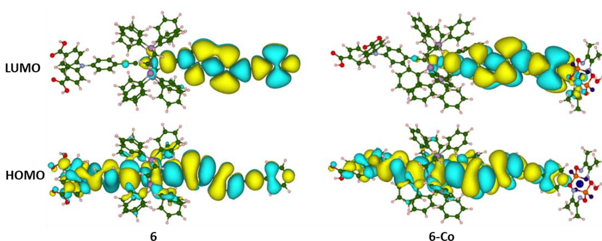
Figure 4. Isodensity surface plots of the HOMO and LUMO of 6 and 6-Co (contour value set to 0.005 a.u.). Color legend: C atom green, O atom red, N atom light blue, Ru atom magenta, H atom white, S atom yellow, P light purple; isodensity positive and negative values are depicted in yellow and cyan, respectively.
