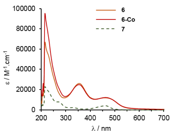
Figure 2. Absorption spectra of 6 , 6-Co and 7 in THF ( C \sim 1.10^{-5} M).
