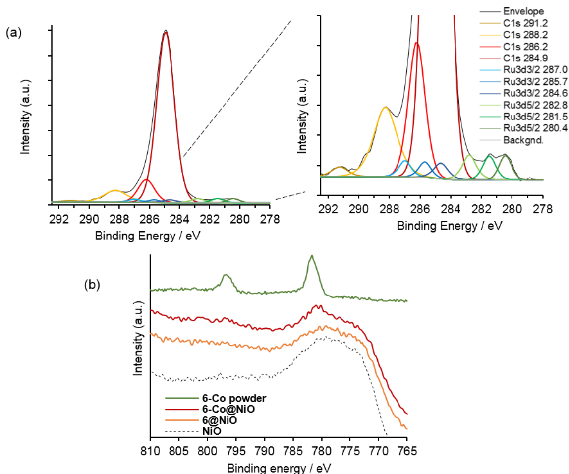
Figure 5. XPS core level spectra of 6-Co@NiO in the Ru 3d -C 1s (a) and Co 2p (b) core regions.
