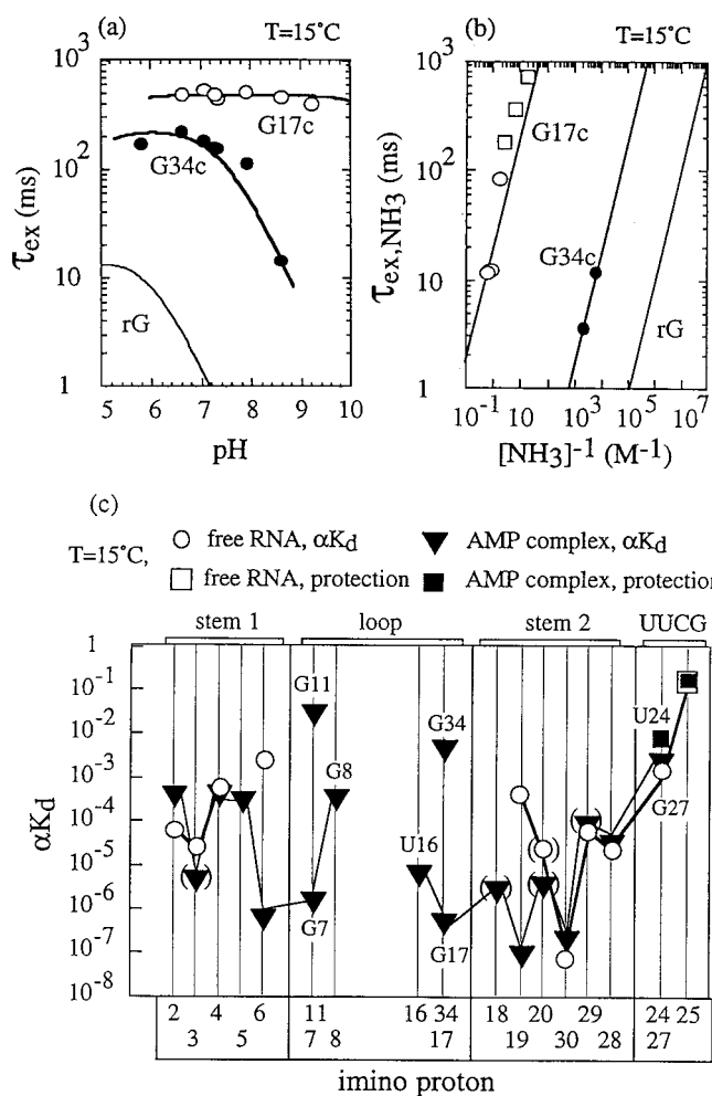
Figure 4. Exchange times of imino protons of G17 and G34 of the G17·G34 mismatch pair in the asymmetric internal loop of the AMP-RNA aptamer complex as a function of (a) pH and (b) the inverse of the ammonia concentration in H 2 O at 15°C. Also shown is the corresponding data for rG monomer under the same conditions. Circles and squares relate to data collected with one and four equivalents of AMP bound per RNA aptamer, respectively. (c) Plot of the apparent dissociation constant ( \alpha K_d ) values (circles and triangles) and the protection factors (squares) as a function of the base or base-pair position in the free RNA aptamer (open symbols) and in the AMP-RNA aptamer complex (filled symbols). \alpha K_d values derived from the measurement of exchange times from poorly resolved imino proton resonances are represented by bracketed symbols. The \alpha K_d values of internal stem Watson-Crick base-pairs exhibit values similar to those reported previously for B-DNA. The two base-pairs flanking either side of the AMP-binding asymmetric internal loop are stabilized on complex formation. The \alpha K_d values of imino protons involved in pairing within the mismatch pairs fall in the same range as the corresponding values of stem Watson-Crick pairs with the values of G7 and G17 amongst the most stable in the complex. (Reproduced from Nonin et al. (1997) with permission from the J. Mol. Biol. )
