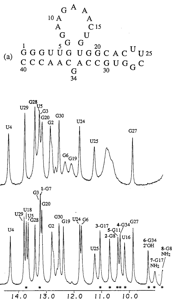
Figure 1. (a) Sequence and numbering system of the AMP-binding 40-mer RNA aptamer. Imino proton NMR spectra (8.8 to 14.8 ppm) of (b) the free RNA aptamer and (c) the AMP-RNA aptamer complex ( \approx 20\% excess AMP) in 10 mM sodium phosphate containing H 2 O solution at pH 6.7 and 0°C. The asterisks in (c) identify additional exchangeable resonances which appeared upon addition of AMP. The imino proton resonance assignments are indicated above the spectra. The additional guanine imino and amino proton resonances and a 2'-OH proton resonance of the asymmetric internal loop that appear on complex formation are designated by numbers in bold face. (Reproduced from Jiang et al. (1996b) with permission of Biochemistry .)
