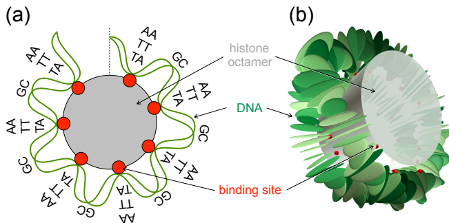
FIG. 3. (a) Nucleosome positioning rules [1]: Key dinucleotides are shown relative to one-half of the symmetric nucleosome. (b) A coarse grained computational model of the nucleosome as employed in Refs. [18–20].
