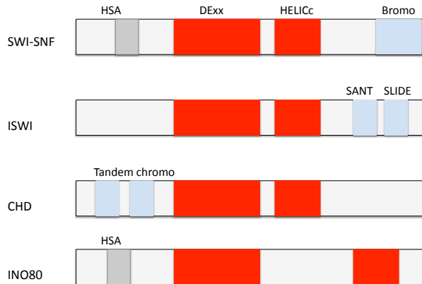
FIG. 1. Definition of the remodeler families according to [4]. DExx and HELICc (shown in red) are ATPase domains, Bromo , SANT and SLIDE, and Tandem chromo (shown in blue) are accessory domains that recognize specific histone tail modifications, or DNA. Adapted from [4].
