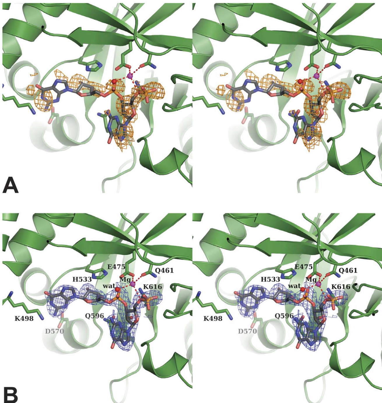
Figure 2. Stereo view of the active site of FimX-EAL domain. (A) The residual density F_o - F_c calculated after molecular replacement with no ligand in the model is contoured in orange at 3 \sigma level (A). The FimX backbone is represented as green cartoon. (B) Interpretation of the density as the bound 5'-pGpG, shown as black sticks. The magnesium ion is shown as a magenta sphere and the catalytic water involved in its coordination as a red sphere. Side-chains of residues involved in ligand binding are shown. The final electron density map 2F_o - F_c contoured at 1.2 \sigma level is traced around the ligand.
