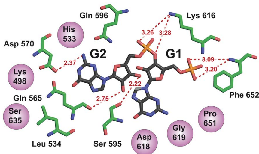
Figure 5. Schematic view of the interactions between FimX-EAL and 5'-pGpG. 5'-pGpG is shown as black sticks. Residues of FimX-EAL involved in polar contacts are shown in green sticks and residues involved in hydrophobic interactions are shown as purple spheres. Polar contacts are shown as red dotted lines. doi:10.1371/journal.pone.0052424.g005
