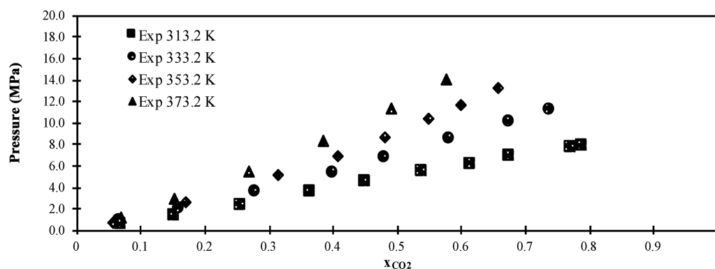
Figure 10. P - x_{\text{CO}_2} diagram for \text{CO}_2 + \gamma -valerolactone system at 313.2, 333.2, 353.2, and 373.2 K.
