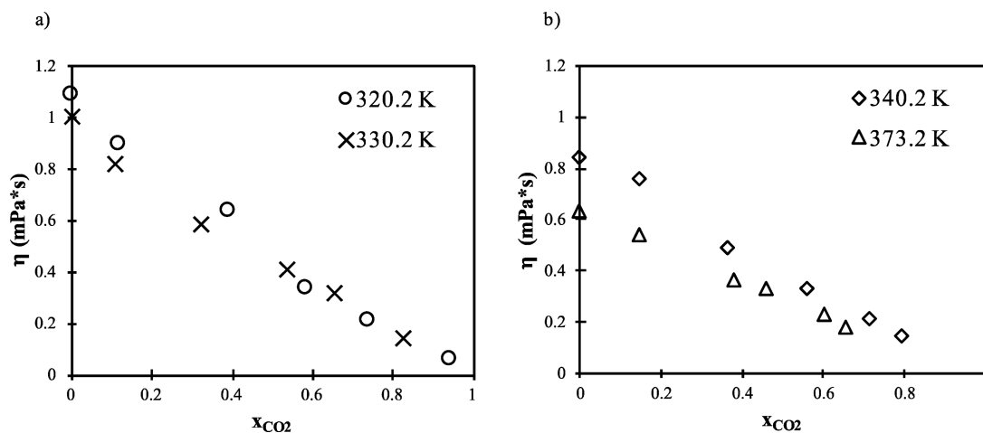
Figure 35. Viscosity vs molar fraction for \text{CO}_2 + diethyl carbonate system at (a) 320.2 and 330.2 K and (b) 340.2 and 373.2 K.
