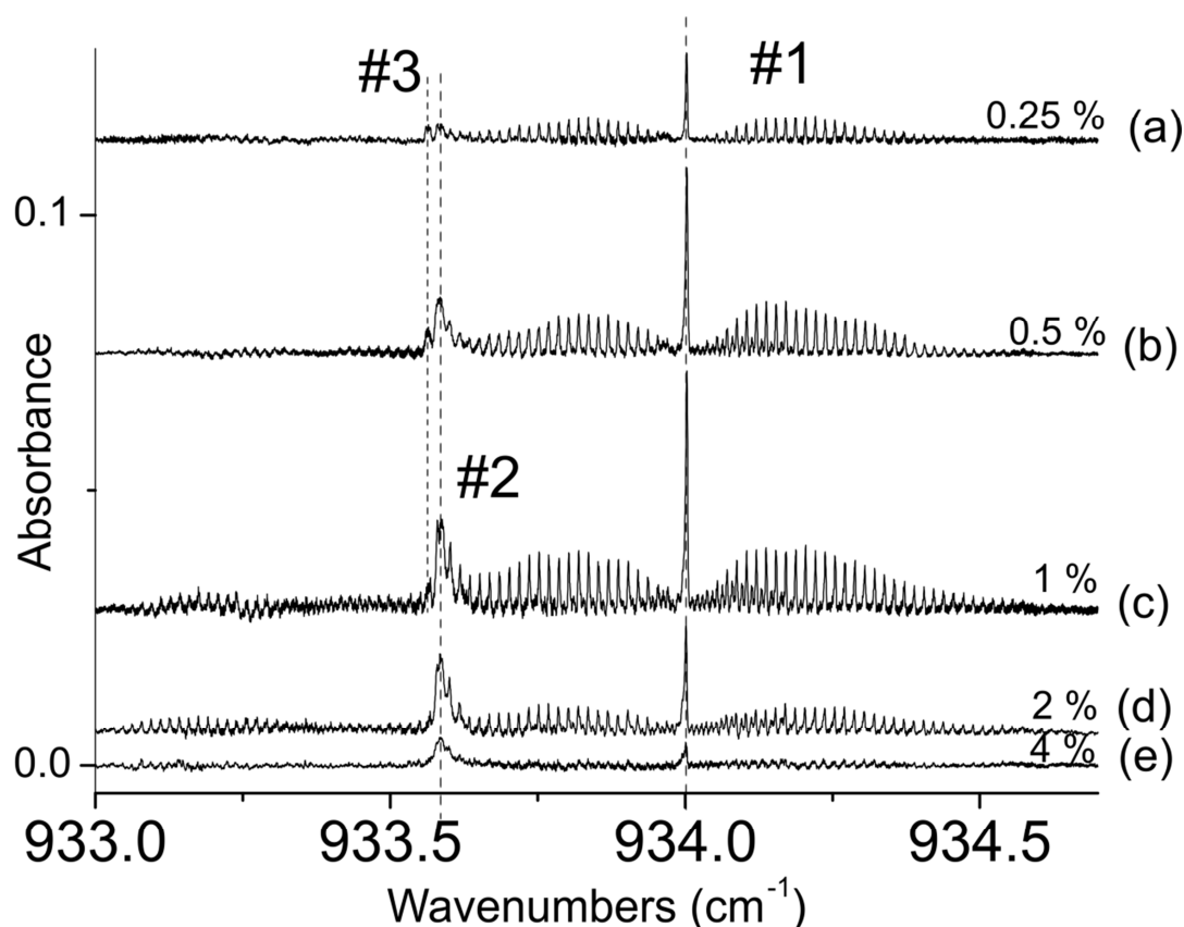
FIGURE 2. EC-QCL absorption spectra of the parallel band of \text{SF}_6 dimer or various concentrations: (a) 0.25%, (b) 0.5%, (c) 1%, (d) 2%, (e) 4% of \text{SF}_6 diluted in helium. The stagnation pressure is 6 bars and the axial distance from the nozzle 9 mm. Reproduced from Phys. Chem. Chem. Phys. 19 (26), 17224 (2017) with permission from the PCCP Owner Societies.
