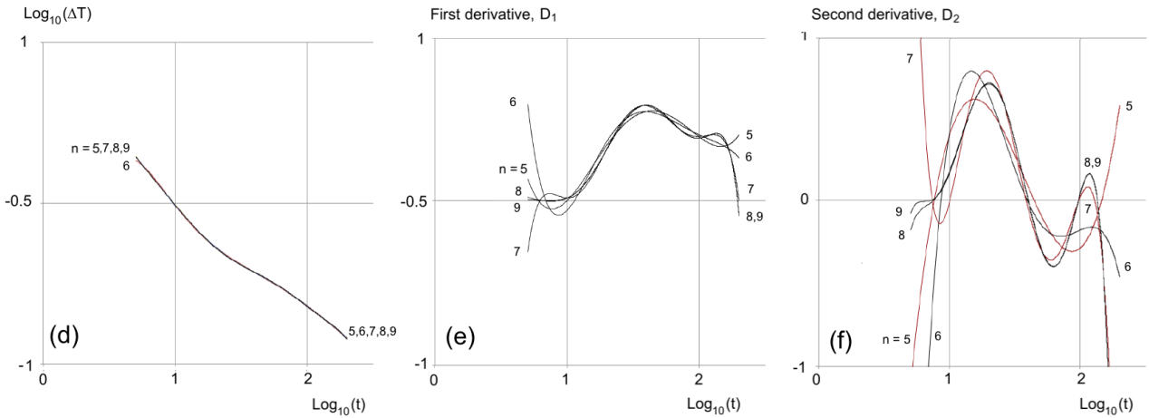
Fig. 9. Combined influence of the time-window ([1s-300s] and [5s-200s]) and of the polynomial degree ( n = 5 to 9 ) on: (a,d) the fitted thermograms \text{Log}_{10}(\Delta T) = f(\text{Log}_{10}(t)) , (b,e) their first derivatives ( D_1 ), (c,f) their second derivative ( D_2 ). The thermogram is normalized by its value at time t = 1 s. Test #1.
