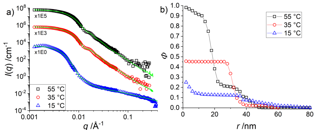
Figure 2: H-pNIPMAM core with H-pNNPAM shell with CCC = 10 mol% at different temperatures. (a) Intensity shifted experimental data of I(q) vs. q of SANS measurements in \text{D}_2\text{O} . The green lines indicate the multi-shell RMC fits. (b) Density profiles obtained with the RMC model.
