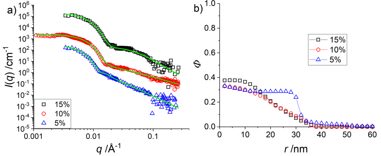
Figure 6: (a) I(q) vs. q from SANS measurements of three H-pNIPMAM-core D7-pNNPAM-shell microgels with different CCC as indicated in the legend at T = 55 °C, under matching conditions of the shell. (b) Density profiles of core monomers determined by multi-shell RMC model.
