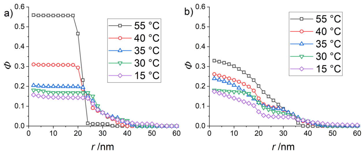
Figure 5: (a): Density profiles of the H-pNIPMAM-core with a CCC of 10 mol% in D 2 O (data adapted from Cors et al. 35 ) (b) Density profiles of the core monomers of the H-pNIPMAM-core D7-pNNPAM-shell system with the same core as in (a) and an index-matched shell (CCC = 1.9 mol%).
