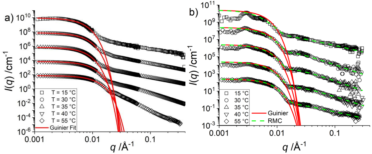
Figure 4: Temperature dependence of I(q) vs. q of SANS measurements at a concentration of 0.1 wt% and the respective Guinier fits (red continuous lines) of (a) A H-pNIPMAM core with a CCC of 10 mol% in D_2O (exp. data adapted from Cors et al. 35 and (b) The same core with a matched D7-pNNPAM shell (12 v% H_2O ), and the corresponding Guinier fits (red continuous lines), and the multi-shell RMC fits (green dashed lines).
