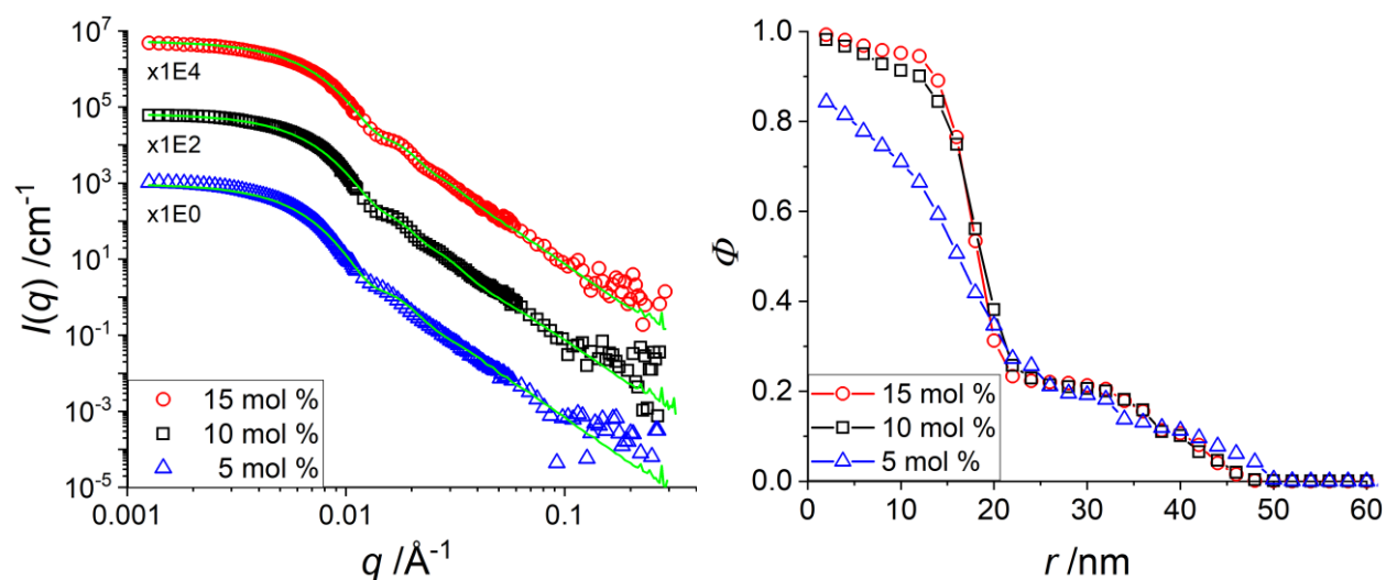
Figure 3: H-pNIPMAM core with H-pNNPAM shell with CCC = 5 mol% (blue triangles), CCC = 10 mol% (black squares) and CCC = 15 mol% (red circles) (a): I(q) vs. q of a SANS measurement at 55 °C in D 2 O (b): Corresponding density profiles obtained by multi-shell RMC model.
