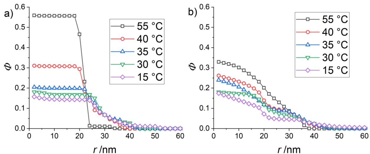
Figure 5: (a): Density profiles of the H-pNIPMAM-core with a CCC of 10 mol% in \text{D}_2\text{O} (data adapted from Cors et al. 35 ) (b) Density profiles of the core monomers of the H-pNIPMAM-core D7-pNNPAM-shell system with the same core as in (a) and an index-matched shell (CCC = 1.9 mol%).
