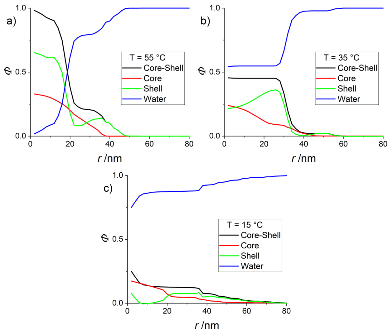
Figure 7: Density profiles of core and shell monomers, and water for H-pNIPAM/D7-pNNPAM core-shell microgels (CCC = 10 % mol) in H 2 O/D 2 O under matching conditions of the shell. (a) T = 55\text{ }^{\circ}\text{C} (b) T = 35\text{ }^{\circ}\text{C} (c) T = 15\text{ }^{\circ}\text{C} .
