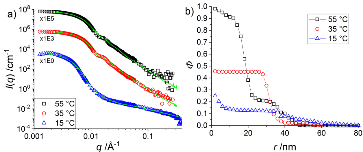
Figure 2: H-pNIPMAM core with H-pNNPAM shell with CCC = 10 mol% at different temperatures. (a) Intensity shifted experimental data of I(q) vs. q of SANS measurements in \text{D}_2\text{O} . The green lines indicate the multi-shell RMC fits. (b) Density profiles obtained with the RMC model.
