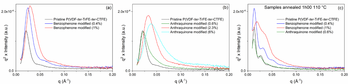
Figure 4. Evolution of the SAXS spectra for the fluorinated modified terpolymers for different contents of (a): benzophenone and (b): anthraquinone, (a,b): as cast and (c): after annealing at 110^{\circ}\text{C} for 1h00.
