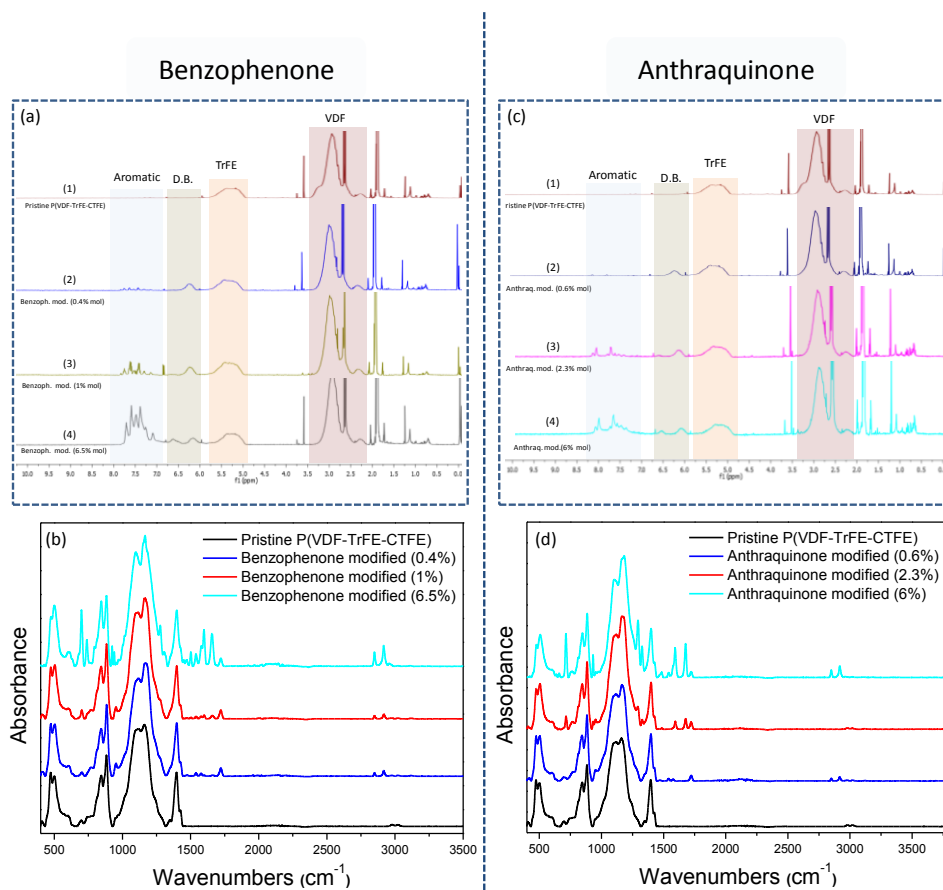
Figure 1. ^1\text{H} NMR (400MHz, acetone- d_6 ) (a,c) and ATR FT-IR (b,d) of P(VDF- ter -TrFE- ter -CTFE) grafted with different benzophenone (a,b) and anthraquinone (c,d) contents.
