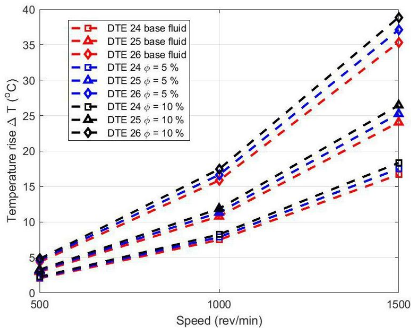
Figure 12. Variation in temperature rise with and without nanoparticles (TiO 2 ) in the lubricant.
