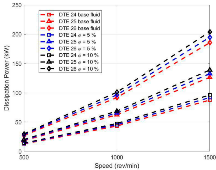
Figure 11. Variation in dissipation power in kW as a function of rotational speed for different nanoparticle (TiO 2 ) volume fraction percentage and lubricant types; the test-case is simulated under 7 kN specific load.
