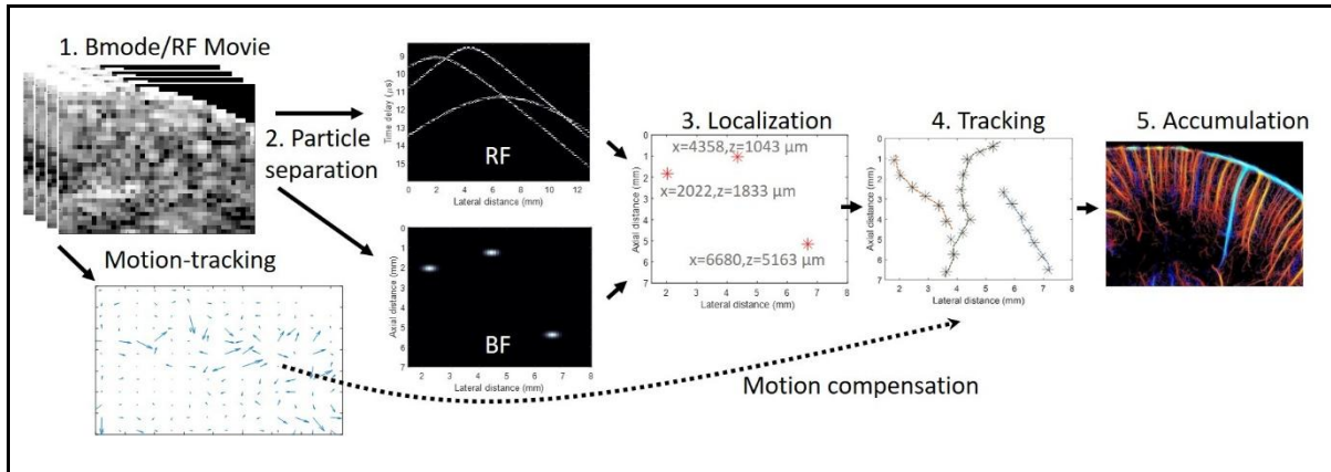
Figure 4: General steps for ultrasound localization microscopy. 1) 100's to 100,000's of images or radio-frequency channel matrices are acquired and stacked 2) Slow-time filtering or low concentration allow the separation of particles/microbubbles 3) The centroids of the hyperbolas or the focal spots created by the microbubble are localized. 4) The localization of microbubbles are assigned to tracks to determine the velocity vector 5) The resulting tracks through the movie are accumulated in one image. In parallel, motion is tracked in the cineloop and used to correct microbubble localization.
