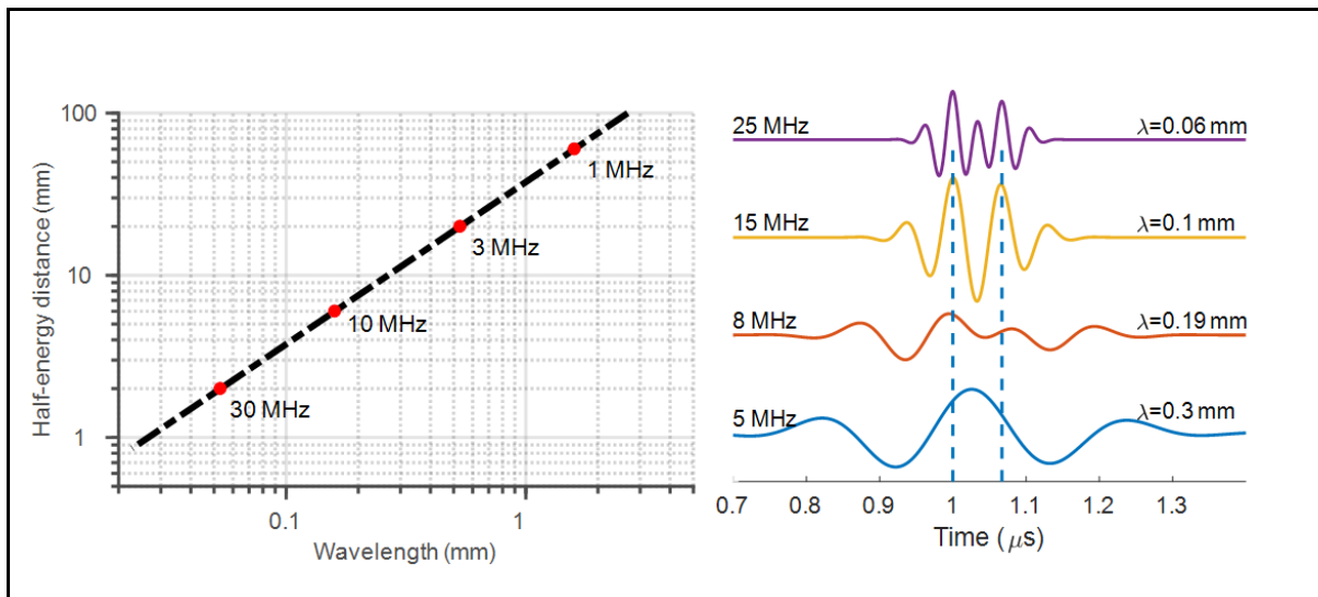
Figure 2: (Left) Compromise between resolution, defined by the wavelength, and ultrasound penetration. The half-energy distance correspond to a loss of 3dB in liver tissue (attenuation \approx 0.5 dB/cm/MHz, extrapolated linearly from [38]). (Right) Separability of two sources (dotted lines), 0.1 mm apart, using acoustic pulses emitted at various wavelengths (60% bandwidth). The sources are indistinguishable when they are closer than a half-wavelength.
