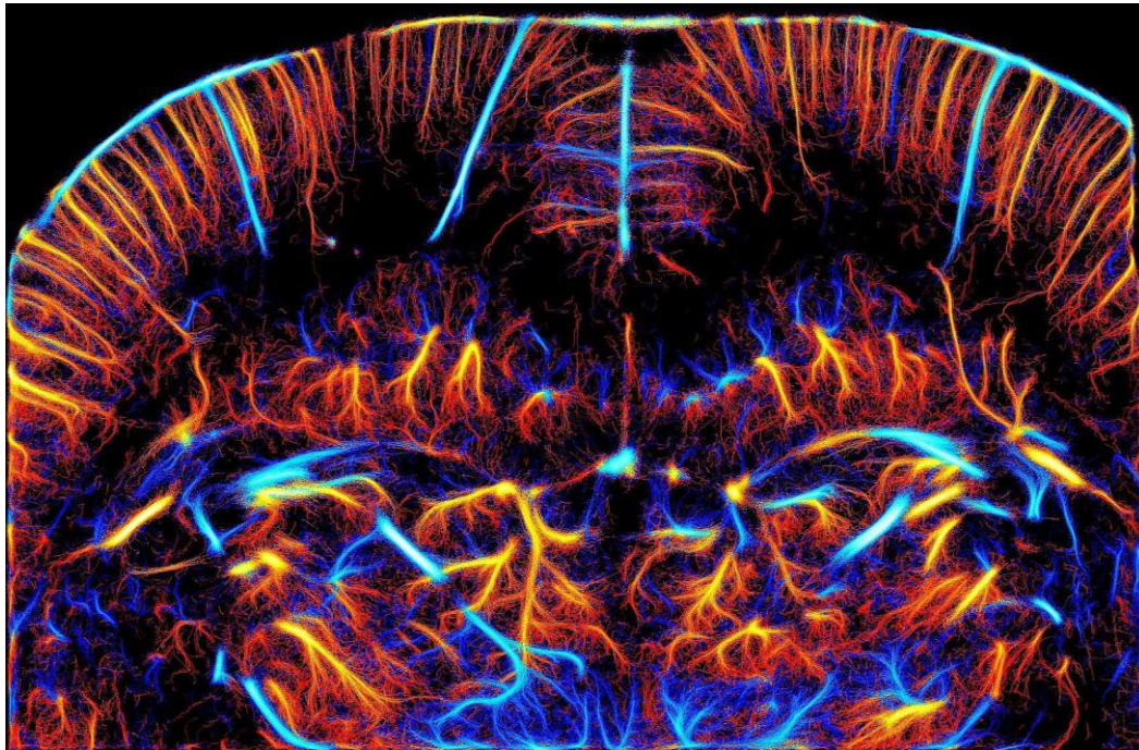
Figure 1: Ultrasound Localization Microscopy of the living rat brain (reconstructed from data in [1])
