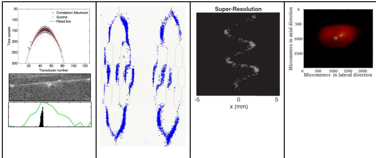
Figure 3: First examples of in-vitro ultrasound localization microscopy a) Ultrafast localization of microbubbles in a liquid and in a tube [© 2011 IEEE. Reprinted, with permission, from [83]] b) 3D ULM in microfluidics channels [Reproduced from [97]with the permission of AIP Publishing] c) 3D low-concentration microbubble localization in a tube [Reproduced from [96] by permissions of Wiley company, all rights reserved] d) Planar low-concentration nonlinear localization of microbubbles in two tubes [Reproduced from [95], © Institute of Physics and Engineering in Medicine. Reproduced by permission of IOP Publishing. All rights reserved]
