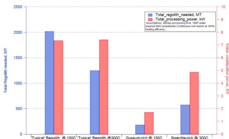
Figure 7.4: An engineering trade showing the processing temperature and quantity of regolith needed to extract water from potential Mars aqueous minerals as defined in the MWIP study (Abbud-Madrid et. al., 2016).
