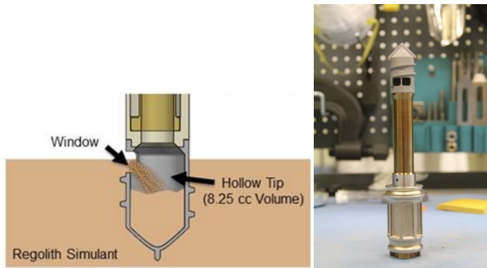
Figure A3.2: Left-Artist's rendition of the M-2020 regolith drill bit collecting granular material as it rotates just below the martian surface. Right-After collection the drill bit and attached sample tube are carefully reoriented to allow the sample to move from the drill bit into the sample tube.
