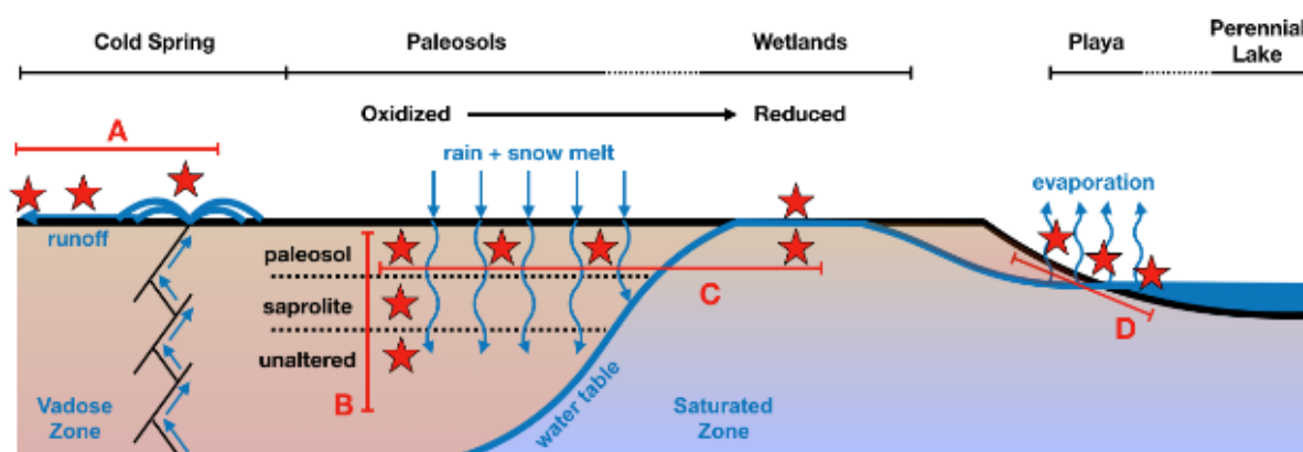
Figure 1.15: Possible relationships between spring deposits, soil horizons, and evaporite deposits. Stars indicate proposed sample locations. Sample suite (A) is of spring precipitate deposits at increasing distance from spring source along fluvial channels. Sample suite (B) are paleosol horizons at increasing depths from the paleosurface, from highly altered to unweathered parent material. Sample suite (C) are paleosols at variable redox states, including reduced wetland deposits. Sample suite (D) are playa evaporite deposits at increasing distance inward from highest lake level. Proposed samples not shown here include rock coatings and rinds.
