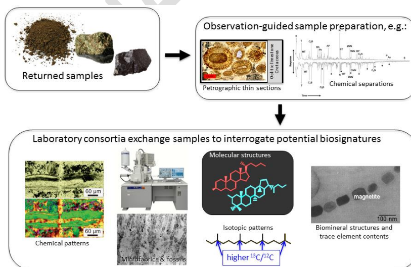
Figure 2.5: Potential biosignatures can be investigated thoroughly only by observation-guided sample preparation, followed by investigations by laboratory consortia that apply state-of-the-art techniques.
