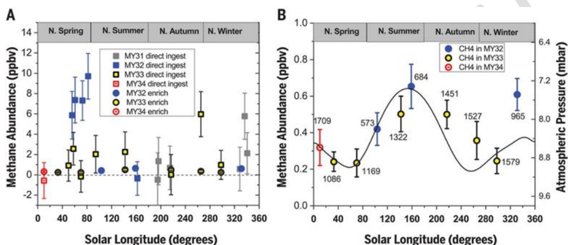
Figure 4.5: Temporal variations in methane abundance of the martian atmosphere at Gale Crater, as measured by the SAM Tunable Laser Spectrometer (TLS). Large excursions to several parts per billion by volume (ppbv) are seen in the full data set (A), as well as seasonal variations in the background levels measured with higher precision. (Webster et al., 2018)
