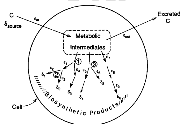
Figure 2.6: A schematic representation of the stable carbon isotopic fractionations associated with biological processes (Hayes 1993). Kinetic isotope effects are indicated by “ \epsilon ,” stable isotope ratio values are represented by “ \delta ” and branch points in carbon flow are indicated by numbers in circles.
