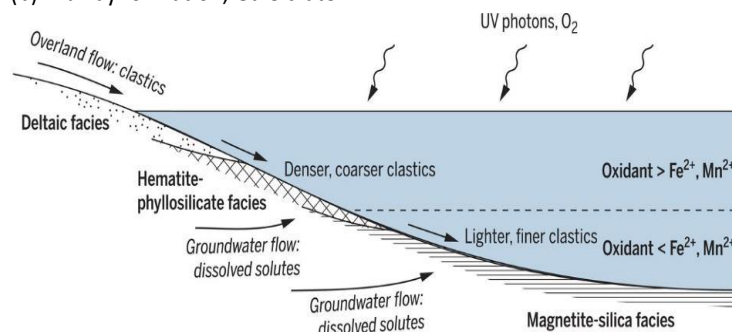
(b) Murray Formation, Gale Crater
