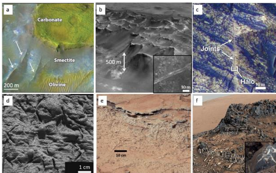
Figure 1.11: (a) groundwater-mineralized Fe/Mg phyllosilicate filled fractures in a > 300 m thick section (Saper and Mustard, 2013) beneath olivine-carbonate rich rocks formed in a shallow aquifer; (b) 500 m penetrative alteration of the NE Syrtis sedimentary sulfate deposits with isopachthus jarosite-bearing ridges (Quinn & Ehlmann, 2018); (c) haloes indicate groundwater flow through Valles Marineris sediments (Okubo et al., 2007); (d) microscopic imager data at Terra Meridiiani shows multiple generations of groundwater mineral precipitation and dissolution, indicated here by crystal vugs, (McLennan et al., 2005); (e) dark nodules and sulfate veins indicate multiple generations of groundwaters in rocks initially formed as Gale lake sediments (Siebach et al., 2014); (f) multiple generations of thick veins, including penetrative fractures indicate groundwaters in deeply buried rocks at Gale crater (Mastcam image from sol 938; Krontyak et al., 2017).
