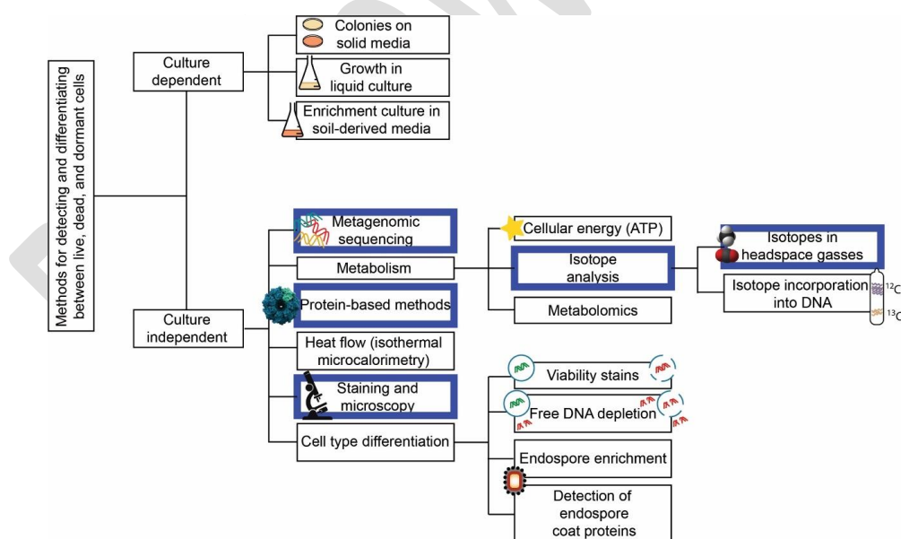
Figure 2.10: Common methods for detecting and differentiating between live, dead, and dormant cells in terrestrial samples. A subset of investigations recommended for initial investigations into Mars return samples are outlined in bold. Figure adapted from Emerson et al (2017).
