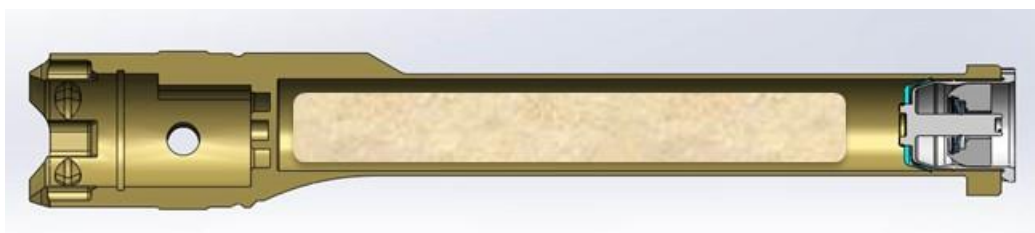
Figure A3. 1: A returnable Mars-2020 sample tube assembly with illustration of a collected core. On the left is the interface with the drill, on the right is the hermetic seal. Total length of the tube is ~15 cm. The sample cavity is ~13 mm x 100 mm.
