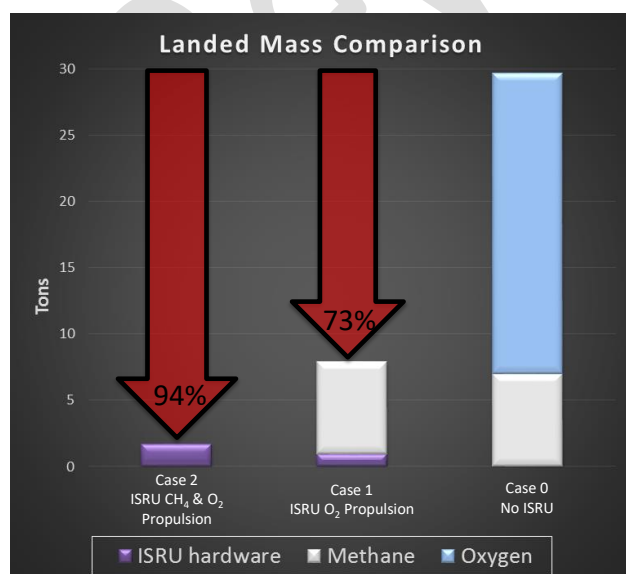
Figure 7.1: Results from an ISRU baseline study (Kleinhenz, 2017) conducted for the Evolvable Mars Campaign showing the benefits of ISRU propellant production. Case 0: the propellant mass needed for a Mars ascent vehicle (Polsgrove, 2015). Case 1: oxygen is produced from the Mars atmosphere and methane is transported from Earth. Case 2: methane and oxygen produced on Mars from the atmosphere and soil water.
