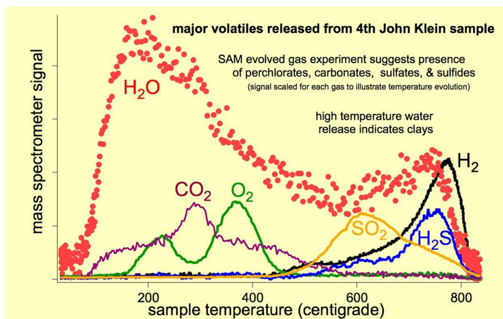
Figure 4.2: The Sample Analysis at Mars (SAM) system on Curiosity has measured a variety of volatiles released from solid samples. The volatiles released from this mudstone were incorporated at some unknown time in the past. With returned samples, it would be possible to provide a more detailed accounting of what volatiles are associated with specific lithologies and potentially to obtain chronologic information about the time of incorporation. Figure from NASA-JPL-CalTech, based on data in Ming et al., 2014.
