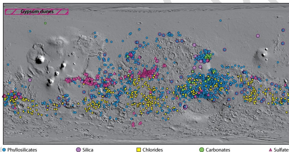
Figure 7.3: A map of aqueous mineral deposits from orbital data (Ehlmann & Edwards, 2014) as potential sources of water for ISRU purposes.
