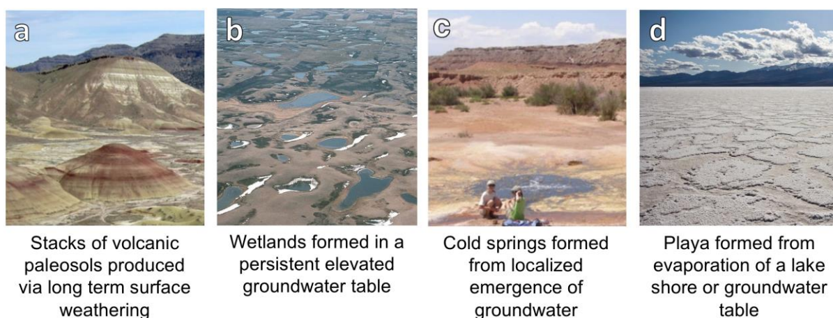
Figure 1.14: Images of subaerial environments, which are linked by their common interactions with the atmosphere and water at the near surface. (a) Paleosol sequence formed on volcanic material, John Day Fossil Beds National Monument, OR. (b) Wetlands in a post-glacial environment, Alberta, CA. (c) Circumneutral cold spring near Green River, Utah (photo: S. Potter-McIntyre). (d) Playa environment in Death Valley, CA.
