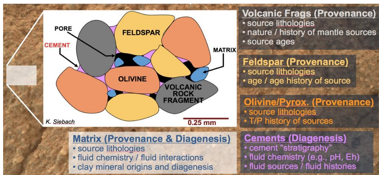
Figure 1.3: Schematic illustration of a microscopic view of a clastic sedimentary rock, illustrating types of information that can be obtained through study of various components (different grains, matrix material, different generations of cements) at a microscopic (sub-micron to millimeter) scale (adapted from http://slideplayer.com/slide/8858365/ ). Many of the analytical methods required to obtain the required mineralogical, textural, structural chemical and isotopic data, such as in situ high resolution microbeam techniques (e.g., ion microprobes, LA-MS) and other cutting-edge laboratory instruments (e.g., TIMS, GS-MS, AMS, STEM), must be carried out in Earth-based laboratories.
