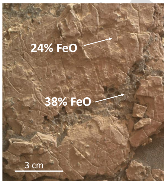
Figure 7.6: Example of anomalous iron detection. MAHLI image of the APXS targets “Morancy Stream” which has 38% FeO and “Morancy Stream Offset” (MSO) which has 24% FeO, acquired on Sol 1668 of the Curiosity rover mission. Image credit NASA/JPL/Caltech/MSSS
