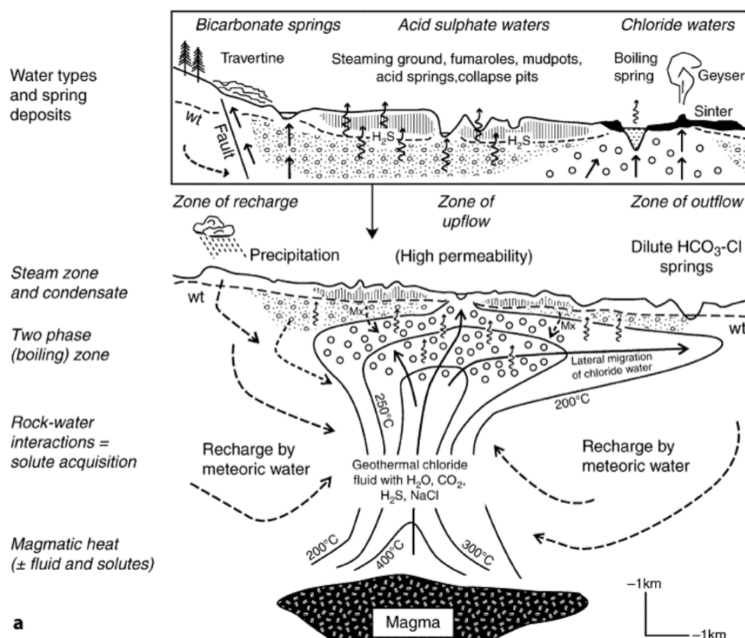
Figure 1.9: Continental terrestrial hot spring fluid types formed by magmatic heating and circulation of mainly meteoric waters that pick up solutes from water-rock interactions to form chloride reservoir-derived fluids (up to 400°C), with variable amounts of dissolved H 2 S and CO 2 , which may (1) rise directly to the surface in upflow zones to form near neutral alkali chloride geysers and hot springs; (2) undergo two-phase boiling during ascent and pressure release to form acidic steam condensate-fed mud pools and fumaroles; (3) feed bicarbonate springs with dissolved CO 2 at the margins of the geothermal field (from Renaut & Jones, 2011).
