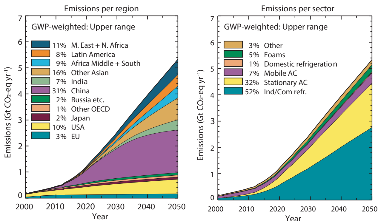
Figure 2-16. Regional and sectoral contributions to HFC GWP-weighted emissions for the upper-range baseline scenario of Velders et al. (2015), excluding HFC-23. The percentages refer to the global average relative contributions of each sector to the total GWP-weighted emissions in 2050. In the scenario, 10 HFCs are considered. The 11 regions are Europe, USA, Japan, other OECD countries, States of the former Soviet Republics and Yugoslavia (Russia), China, India, other Asian countries, Middle and Southern Africa, Latin America, and the Middle East plus Northern Africa. The six use sectors are (1) industrial, commercial (open compressor), commercial (hermetically sealed compressor), and transport refrigeration, (2) stationary AC, (3) mobile AC, (4) domestic refrigeration, (5) foams—extruded polystyrene, polyurethane, and open cell foams, and (6) other—aerosol products, fire extinguishing systems, and solvents. The emissions shown here are based on the GWPs used in Velders et al. (2015), which differ somewhat from those in Table 2-2 ; the difference in CO 2 -eq emissions is less than 1%.
