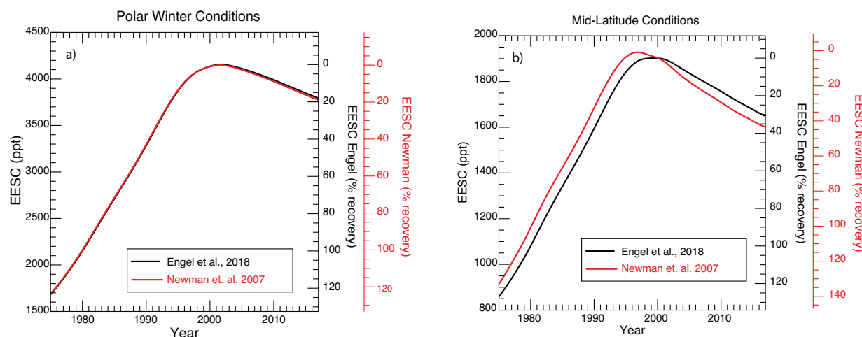
Figure 1-18. Level of EESC recovery towards 1980 benchmark values comparing the EESC calculation as used in the 2014 Assessment (Carpenter and Reimann et al., 2014; Newman et al., 2007) to the new method suggested by Engel et al. (2018). Plot (a) is for 3 years of mean age, representative of mid-latitude conditions, while plot (b) is for 5.5 years of mean age, representative of polar winter conditions. In all cases, the different age spectra (see Box 1-2 ) were parameterized as suggested by Newman et al. (2007) using half of the mean age as width of the age spectrum and an inverse Gaussian function as the shape of the age spectrum. The age spectrum has been integrated over a time period of 20 years. Fractional release factors were used as in the last Assessment report and in Velders and Daniel (2014) for the formulation according to Newman et al. (2007). In the calculation using the formulation suggested by Engel et al. (2018), the same fractional release factors were used, but these were modified to be consistent with the formulation of fractional release suggested by Ostermüller et al. (2017), as explained in Engel et al. (2018). The same tropospheric data were used as in Section 1.4.1.1 and Section 1.4.2.1 . VLSL contributions to EESC are not included in this calculation. In the calculation of EESC, the higher efficiency of bromine to destroy stratospheric ozone is taken into account. As in previous Assessments, we adopt a factor of 60 for mid-latitude conditions and a factor of 65 for polar winter conditions.
