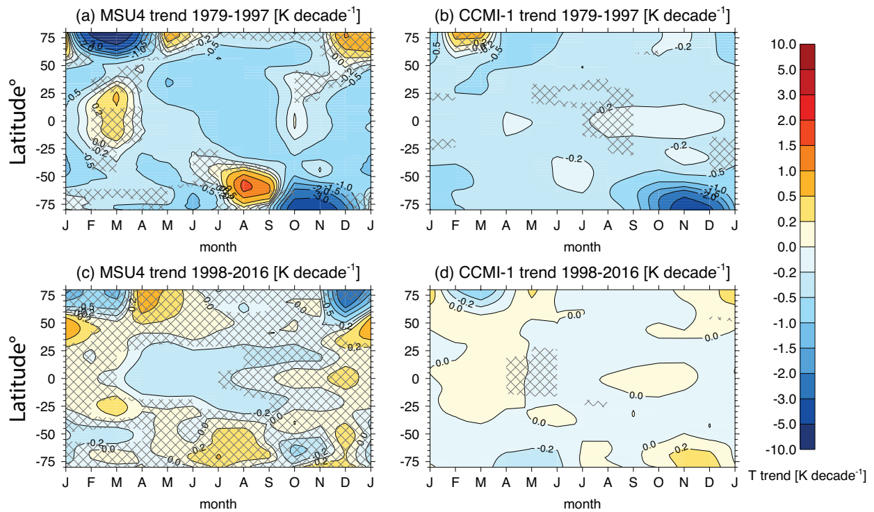
Figure 5-6. Lower-stratospheric temperature trends over the periods (a, b) 1979–1997 and (c, d) 1998–2016 in K per decade as a function of latitude and month from (a, c) satellite MSU/AMSU NOAA/STAR v4.0 (MSU4) and (b, d) multi-model mean MSU4 temperatures from 12 CCMI models for the REF-C2 simulation. The following years, which were influenced by volcanic eruptions, are treated as missing data in panels a and b: 1982, 1983, 1991, 1992, 1993. The hatching in panels a and c shows where the magnitude of the observed trend is within the 5–95% range of simulated internal variability, estimated from the spread in modeled trends, and is therefore estimated to be not statistically significant (at the 95% confidence level). Hatching in panels b and d shows where the observed MSU4 trends in panels a and c lie outside the 5–95% range of model trends, thus showing areas where the simulated and observed trends are inconsistent. Based on datasets described in Maycock et al. (2018).
