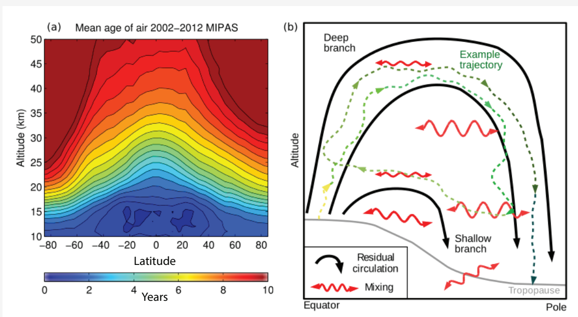
Box 5-2 Figure 1. (a) Climatology of annual mean age of air 2002–2012 from MIPAS \text{SF}_6 measurements and (b) schematic of the net stratospheric tracer transport circulation, including overturning circulation and mixing components. (a) Note that MIPAS mean age is overestimated at high latitudes due to an \text{SF}_6 mesospheric sink (Stiller et al., 2012). (a) Adapted from Haenel et al. (2015). (b) Adapted from Garny et al. (2014).
