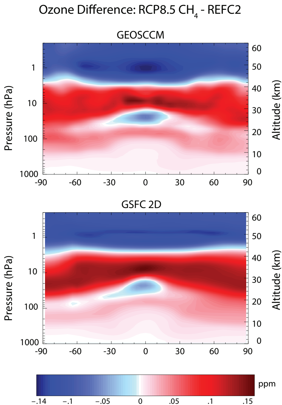
Figure 6B-3. Profile ozone sensitivity to CH 4 . This shows the ozone mixing ratio difference (ppm) between simulations using the RCP8.5 CH 4 (high) scenario and the baseline REF-C2 (RCP6.0 CH 4 ) from the GEOSCCM and GSFC 2-D model, averaged over the period 2070–2099 to minimize interannual variability in the GEOSCCM. Negative differences are indicated by the blue colors, positive differences by the red colors.
