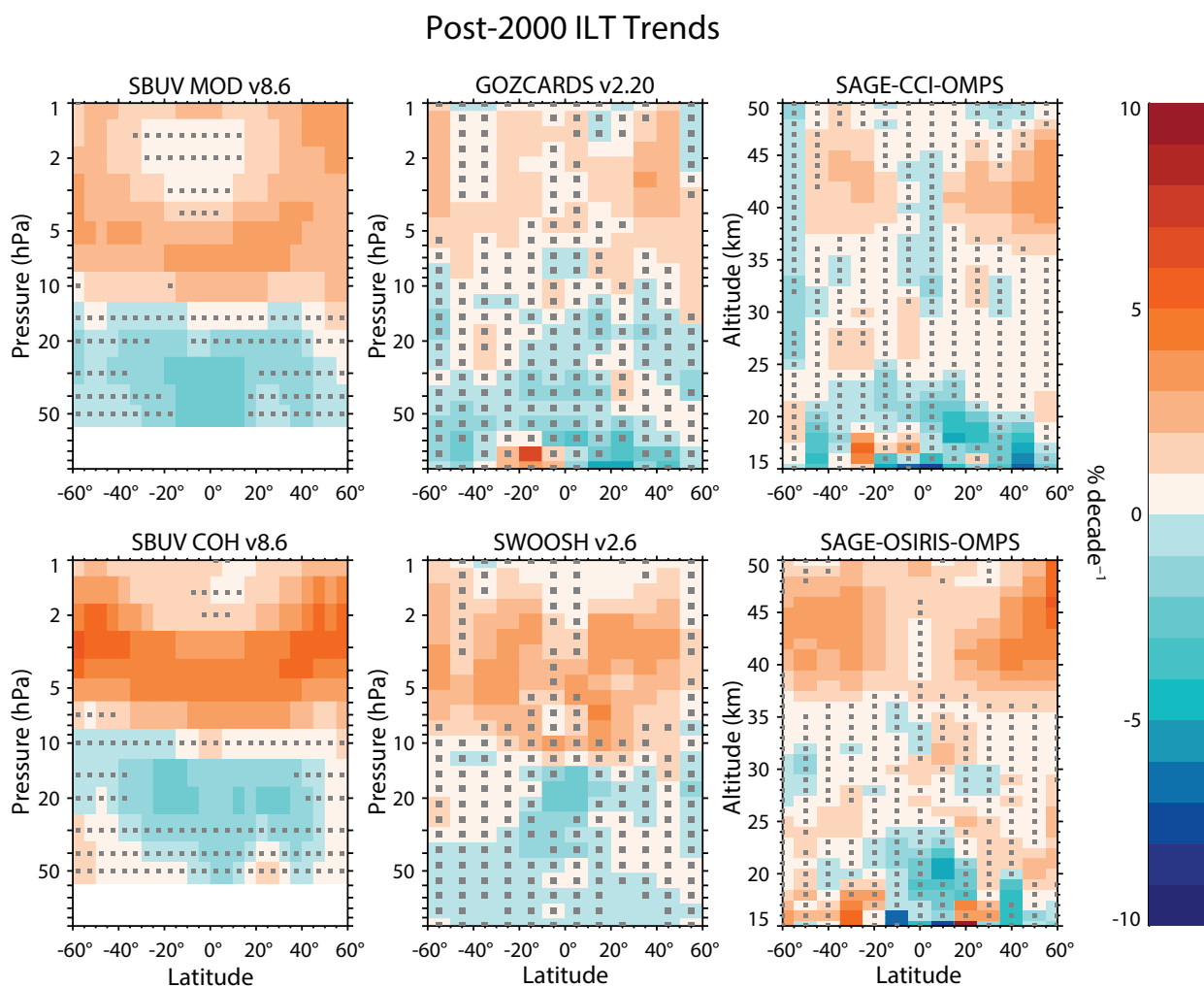
Figure 3-18. Ozone trends for the period 2000–2016 estimated from six satellite data records using the independent linear trend (ILT) model. Gray stippling denotes results that are not significant at the 2\sigma level. Data are presented on the latitudinal grid and vertical coordinates associated with each dataset. Adapted from LOTUS (2018).
