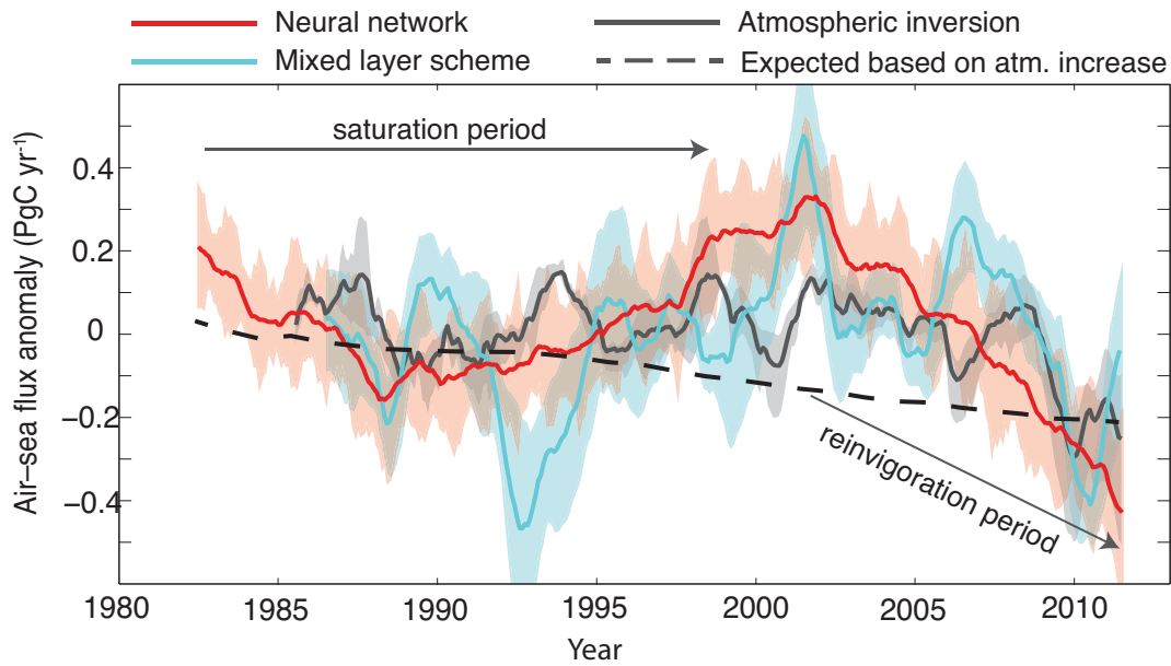
Figure 5-20. Evolution of the Southern Ocean carbon sink based on (red and blue lines and shading) two methods to interpolate surface ocean observations and (black solid line and gray shading) an atmospheric inversion method. The expected uptake based on the growth of atmospheric \text{CO}_2 alone is shown by the dashed black line. Negative values indicate anomalous uptake by the ocean. Adapted from Landschützer et al. (2015).
