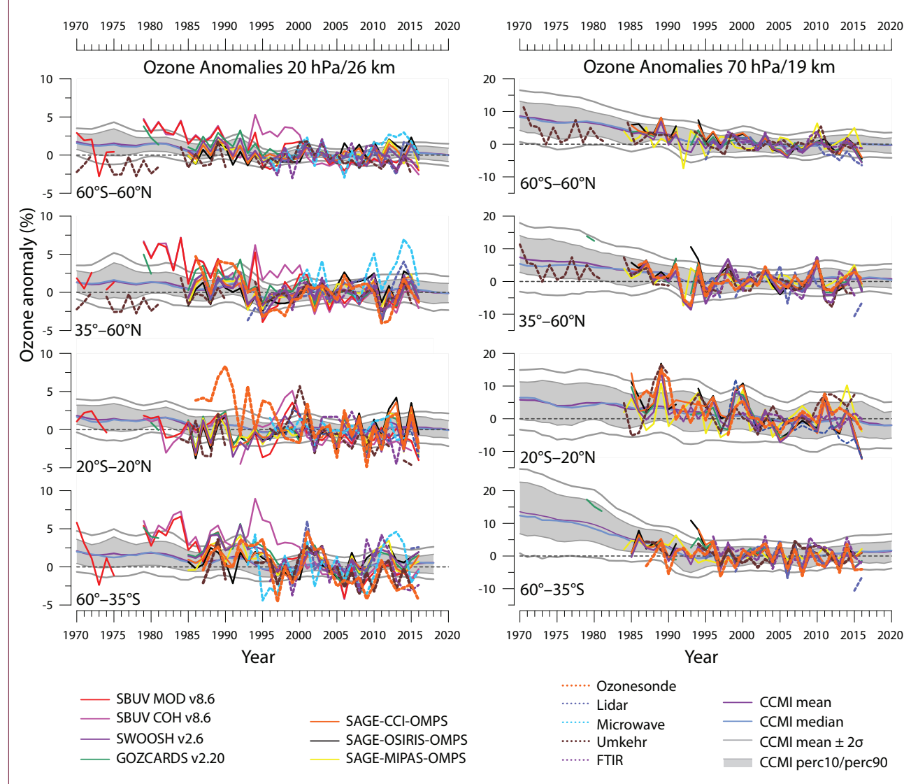
Figure 3-16. Same as Figure 3-15 but for levels 20 hPa/26 km (left) and 70 hPa/19 km (right). Adapted from LOTUS (2018).
