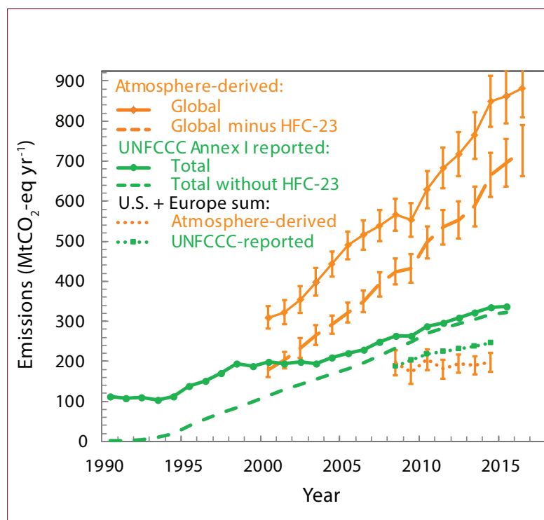
Figure 2-13. Summed HFC emissions, expressed as CO 2 -eq, reported to UNFCCC (UNFCCC 2017) and based on atmospheric measurements, for the global and for the sum of the U.S. and European regions. (Global emission values from Figure 2-1 ; measurement-based regional estimates for the U.S. and Europe are taken from Figure 2-4 and Figure 2-5 ). Sums including emissions of HFC-23 (solid lines) and without HFC-23 (dashed lines) are shown. Uncertainties on global estimates represent one standard deviation of estimates (see Figure 2-1 ); Uncertainties on regional estimates are approximate, based on the range and standard deviation quoted in the original sources (Graziosi et al., 2017 and Hu et al., 2017).
