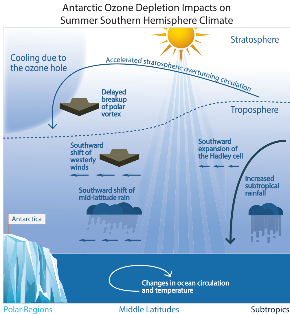
Figure 5-12. Schematic illustration of Southern Hemisphere climate impacts in austral summer associated with Antarctic ozone depletion. Ozone depletion has cooled the Antarctic stratosphere, leading to a delayed breakup of the stratospheric polar vortex and an accelerated Brewer–Dobson circulation. Impacts extended into the troposphere: A region of strong westerly winds and associated rainfall shifted southward, affecting the ocean circulation. The subtropical edge of the tropical circulation also expanded poleward, leading to reduced precipitation in mid-latitudes and enhanced precipitation in the subtropics. Update to Figure 4-22 in Arblaster and Gillett et al. (2014).
