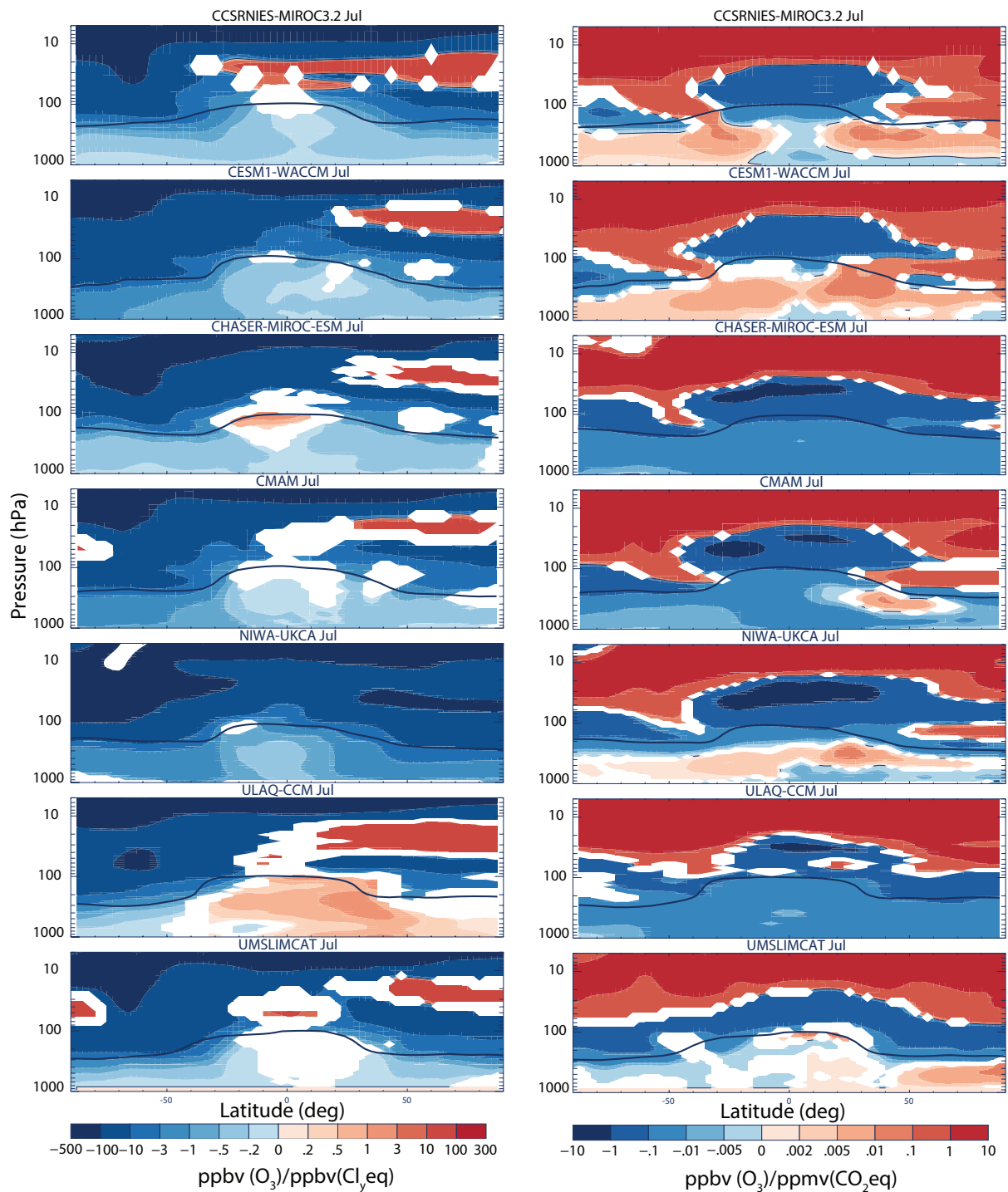
Figure 3-32. Ratio of zonal mean ozone volume mixing ratio (VMR) changes to VMR in (left column) equivalent Cl (Newman et al., 2007) and (right column) equivalent CO 2 (sum of CO 2 , HFCs, PFCs, and SF 6 ) for seven CCMI-1 models for July. The solid black lines indicate 150 ppbv of ozone. Adapted from Morgenstern et al. (2018).
