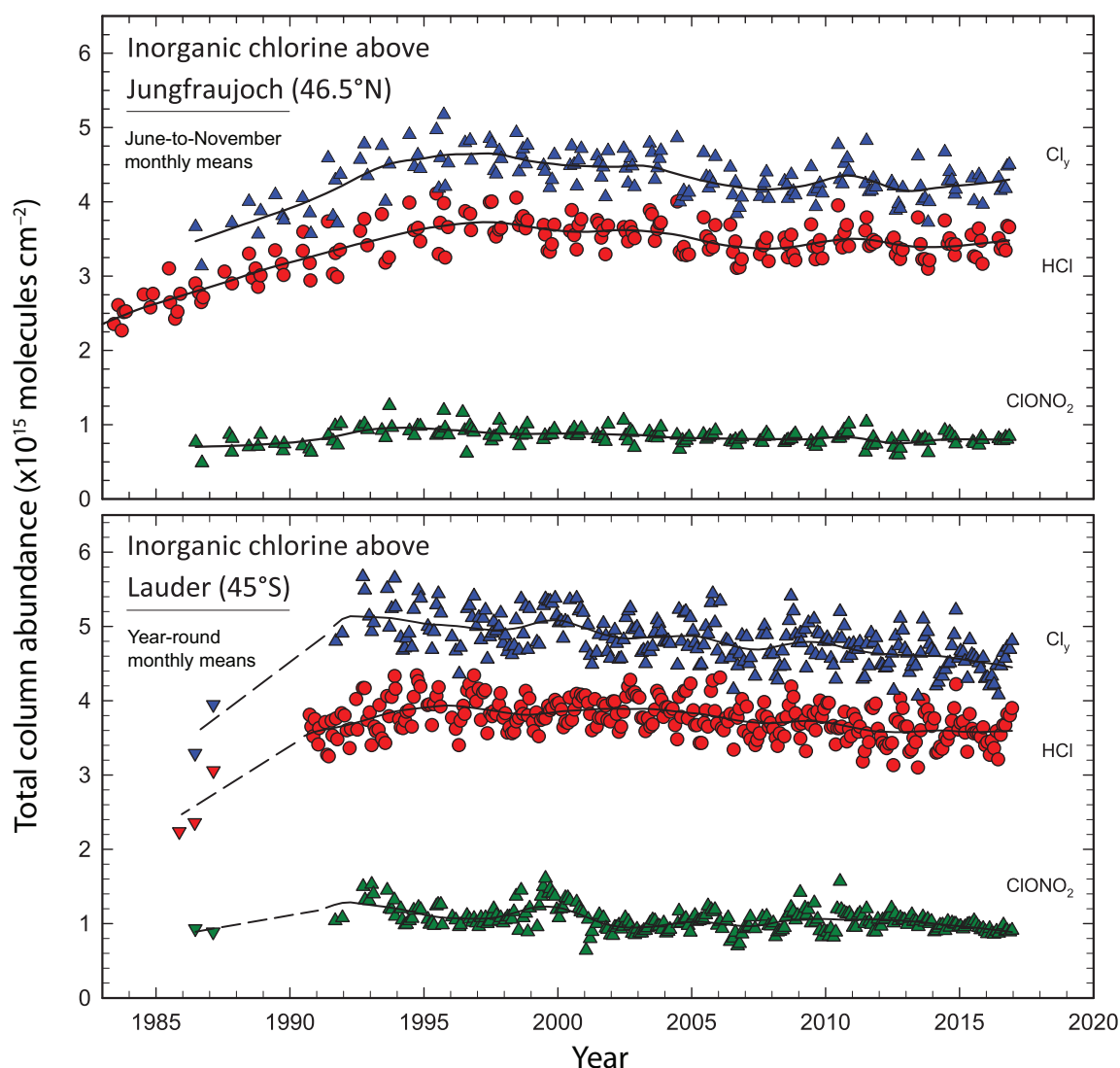
Figure 1-13. Multi-decadal monthly mean total column time series of the two main chlorine reservoirs, \text{HCl} and \text{ClONO}_2 , and their summation, as monitored at the Jungfraujoch station (Swiss Alps, 46.5°N, 3,580 m altitude) and the Lauder station (New Zealand, 45.0°S, 370 m altitude), in the framework of the NDACC network. For the Jungfraujoch, in contrast to the data shown in Figure 1-2, the datasets are restricted to the June to November months in an effort to limit the variability caused by atmospheric transport and subsidence during winter and spring. The continuous lines come from non-parametric least-squares fits involving an integration time of about 3 years and help to visualize the non-monotonic and non-linear changes in stratospheric chlorine after the peak from 1996 to 1997.
