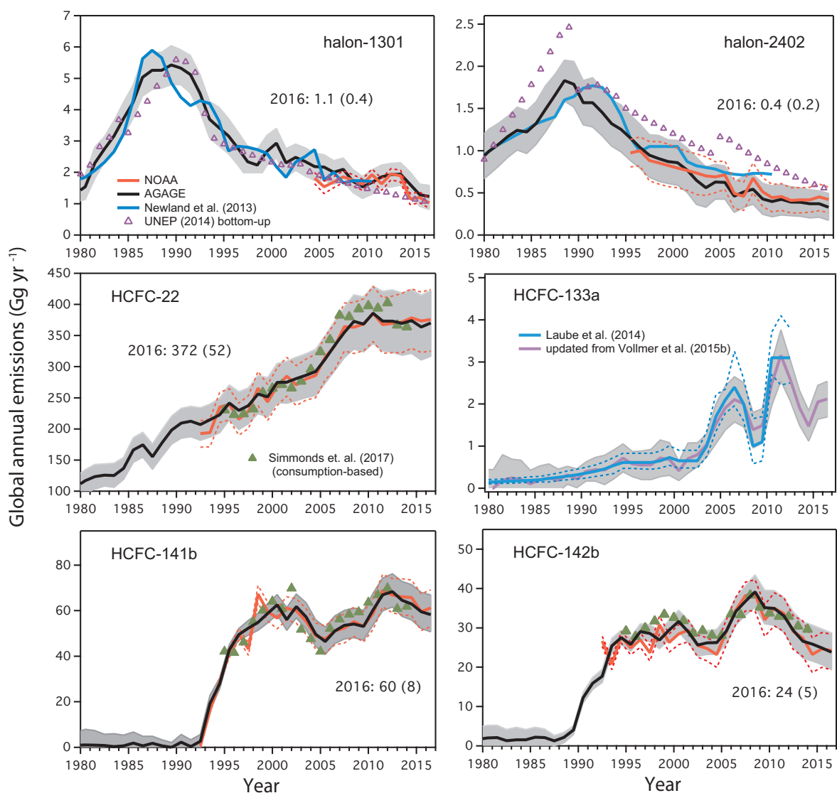
Figure 1-4. Top-down and bottom-up global emission rate estimates (Gg yr -1 ) for ozone-depleting substances. Top-down emissions rates from AGAGE (black) and NOAA (red) atmospheric data were calculated using a global 12-box model (Box 1-1; Cunnold et al., 1983; Rigby et al., 2013). For the CFCs, stratospheric lifetimes were assumed to be equal to the total lifetimes from Table A-1 (no other losses were assumed). For the halons, lifetimes are summarized in Vollmer et al. (2016). A lifetime of 32 years was used, derived from stratospheric, ocean, and soil lifetimes of CCl 4 (Butler et al., 2016; Rhew and Happell, 2016; SPARC, 2013). For the other species, stratospheric lifetimes from Table A-1 were imposed, with OH rate constants from Burkholder et al. (2015). Global steady-state lifetimes for each species were: CFC-11 (52 years), CFC-12 (101 years), CFC-13 (640 years), CFC-113 (93 years), combined CFC-114/CFC-114a (189 years), CFC-115 (540 years), halon-1211 (16 years), halon-1301 (72 years), halon-2402 (28 years), HCFC-22 (11.6 years), HCFC-141b (9.2 years), HCFC-142b (17.6 years), and HCFC-133a (4.6 years). For some of these species, small differences can be seen between these global steady-state lifetimes calculated using the 12-box model and those in Appendix Table A-1, due to differences in assumed OH and model transport. Emissions were estimated using a Bayesian inverse method, in which the emissions growth rates from bottom-up inventories were used as a priori constraints (Rigby et al., 2011; Rigby et al., 2014) with minor update in Vollmer et al. (2018). Descriptions of bottom-up datasets are given in Rigby et al. (2014); Rigby et al. (2013); Simmonds et al. (2017); Vollmer et al. (2016); and
