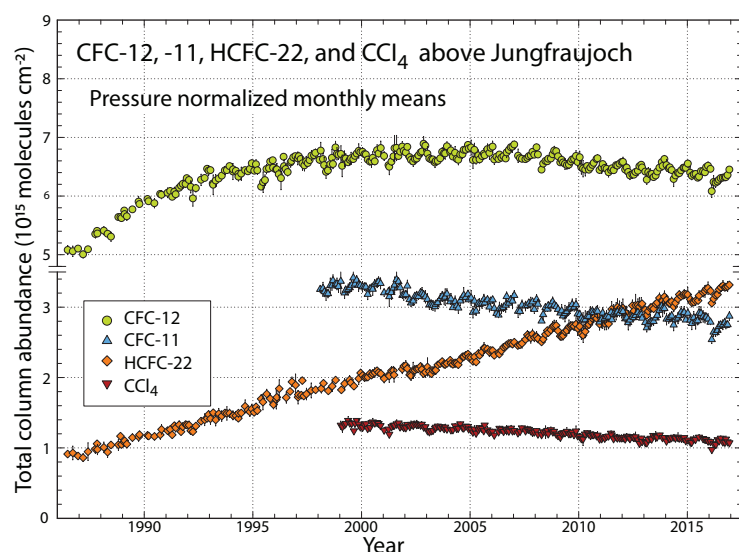
Figure 1-2. Monthly mean total vertical column abundances (in molecules per square centimeter) for CFC-12, CFC-11, CCl 4 , and HCFC-22 above Jungfraujoch station, Switzerland, from 1986 to 2016 (updated from Zander et al., 2008 and Rinsland et al., 2012). The bootstrap resampling tool described by Gardiner et al. (2008) and Rinsland et al. (2012) was used for the trend evaluations (see Table 1-2 ). Note the discontinuity in the vertical scale.
