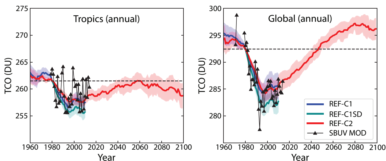
Figure 3-26. Adjusted and smoothed multi-model mean time series of annual mean tropical ( left ) and global ( right ) total column ozone (TCO) from CCMI models (colored lines) and from observations (solid black lines and symbols). Note that the multi-model mean uses a 1\sigma threshold (MMM1S) for filtering (for method see Dhomse et al., 2018, Figure 2, bottom). The dashed black lines represent 1980 values of TCO.
