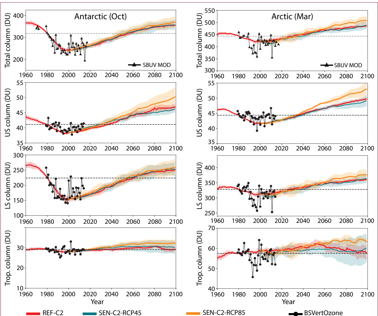
Figure 4-20. (top) Evolution of total column ozone (in Dobson Units, DU) MMM1S for the CCMI REF-C2 simulation (red lines) and the CCMI RCP scenario simulations SEN-C2-RCP45 (blue-green lines) and SEN-C2-RCP85 (orange lines). The REF-C2 simulation uses the RCP-6.0 scenario. Also shown are the partial ozone columns for the upper stratosphere (second row), the lower stratosphere (third row) and the troposphere (bottom). For comparison the respective total and partial ozone columns are shown. The black dashed lines denote the 1980 reference values for each region and layer. Adapted from Dhomse et al. (2018).
