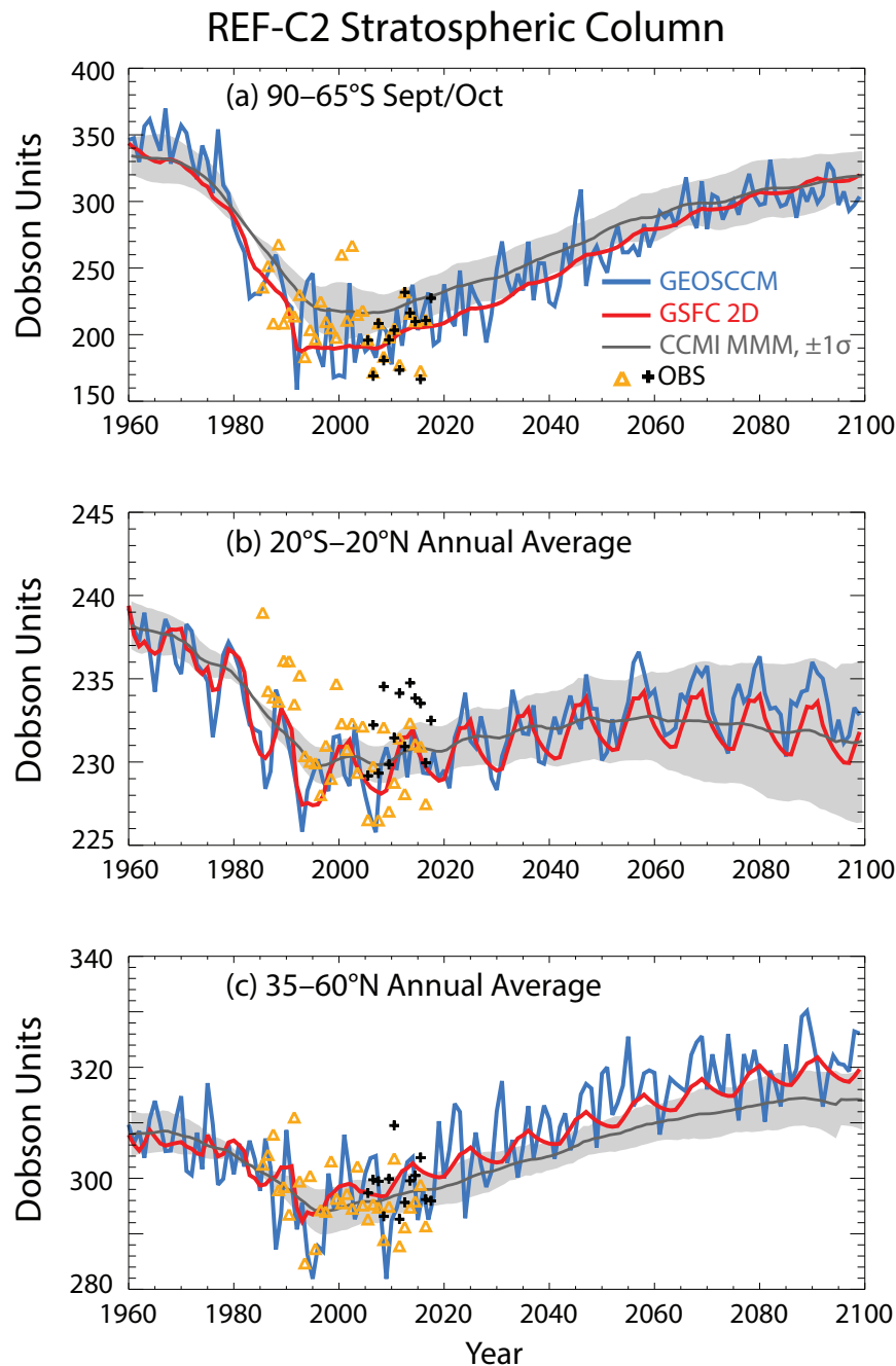
Figure 6B-2. Comparison of past and future stratospheric column ozone in select latitude bands from the baseline REF-C2 simulations and observations. This shows the ozone column above the tropopause (seasonally- and latitude-dependent) from the GSFC 2-D model (red line) and GEOSCCM 3-D model (blue line) for 1960–2100. Also shown are the CCMI multi-model mean (MMM, dark gray line) with \pm 1\sigma (gray shading) (see Sections 3.4 and 4.5 of this Assessment, and Dhomse et al., 2018 for details). The observations are stratospheric column ozone from: Aura/MLS version 4.2 for 2005–2017 (black +), and Global Ozone Chemistry And Related trace gas Data records for the Stratosphere (GOZCARDS) version 2.20 for 1985–2016, updated from Froidevaux et al., 2015 and time-interpolated to fill in missing data (orange \Delta ). To facilitate visual comparison and minimize the model biases in the 1960s, the following offsets were applied: (a) MMM: +15 DU; (b) MMM: –16 DU, GOZCARDS: +2 DU; (c) GEOSCCM: –5 DU, GOZCARDS: +2 DU.
