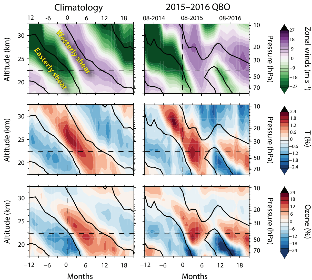
Figure 3-5. Impact of the 2015–2016 QBO disruption on stratospheric variables. The rows show (top) the MERRA-2 zonal-mean zonal wind component (in \text{m s}^{-1} ), (middle) deseasonalized MLS temperature anomalies (in %), and (bottom) ozone anomalies (in %) as a function of time and pressure (relative to the long-term monthly averages), averaged over 5^{\circ}\text{S} – 5^{\circ}\text{N} . The left column shows the composite of the easterly-to-westerly shear transitions based on 4 shear transitions at 40 hPa. The right column shows the 2015–2016 QBO cycle, which includes the data from April 2014 to September 2016, with month 0 (vertical dashed lines) being May 2016. The thick black contours denote the zero wind shear. The horizontal dashed lines indicate the 40 hPa level. Adapted from Tweedy et al. (2017).
