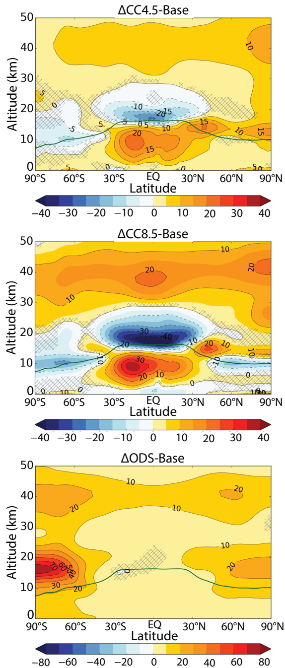
Figure 3-28. Modeled percent changes in annual mean ozone between 2000 and 2100 due to GHG changes according to RCP-4.5 ( top ) and RCP-8.5 ( middle ) and due to ODS changes ( bottom ). Shown are differences between a year-2000 baseline simulation with single forcing changes for year-2100 conditions: RCP-4.5 and RCP-8.5 assume year-2100 SST, sea-ice, and GHG concentrations with year-2000 ODS and ozone precursor emissions. From Banerjee et al. (2016).
