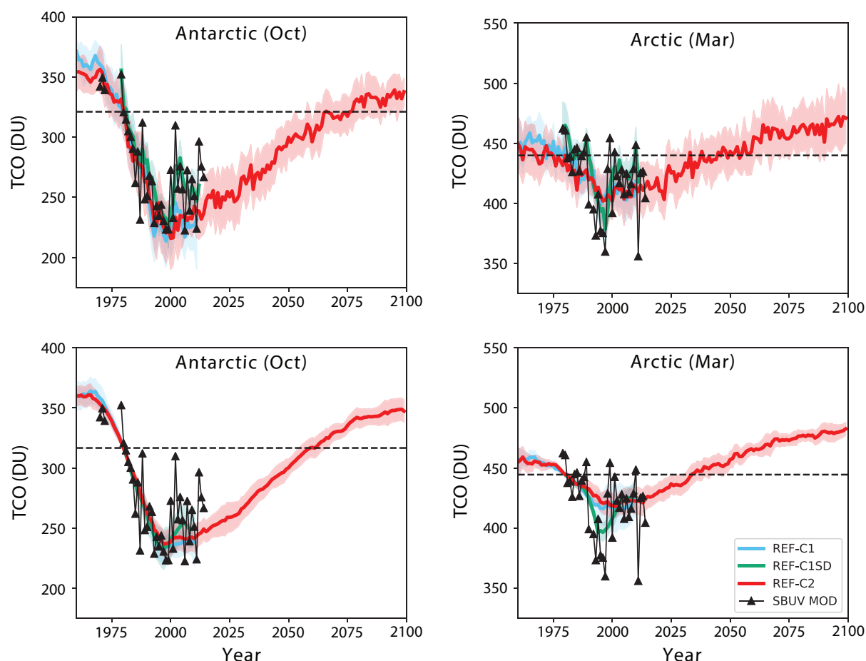
Figure 4-18. Multi-model mean (MMM15) total column ozone time series (in Dobson Units, DU) from CCMI REF-C1 (light blue), REF-C1SD (green) and REF-C2 (red) simulations for the (left) SH polar (October) and (right) NH polar (March) regions. The dashed black lines show the 1980 reference value for each latitude band. The top row shows the unadjusted modeled values and the bottom row shows the time series adjusted with respect to mean 1980–1984 observations. Also shown are the merged SBUV observations. From Dhomse et al. (2018).
