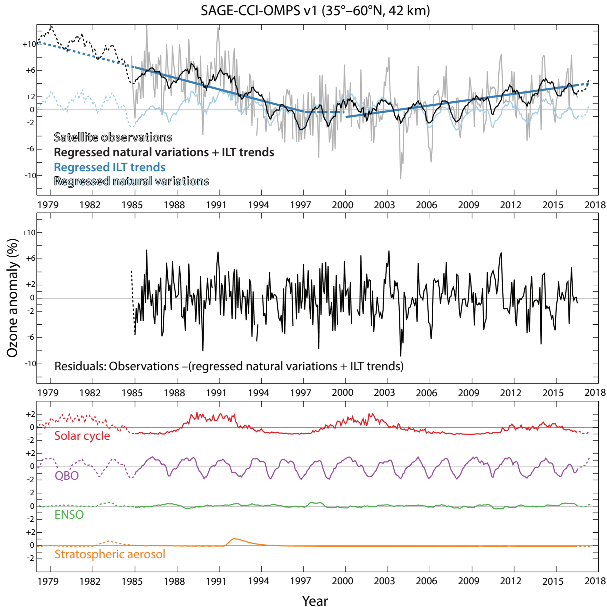
Figure 3-7. Terms in the regression of monthly deseasonalized ozone anomalies from SAGE-CCI-OMPS at 42 km in the 35°–60°N zonal band. The top panel shows observed monthly mean anomalies (in %; gray line) relative to the annual cycle of ozone. The black line is the result of the regression model including the independent linear trends (ILTs; thick blue lines). The light blue line shows the sum of the terms of the regression model without the ILTs included. The middle panel shows the residual in the observed ozone when the long-term trend and regressed natural variations are subtracted. The bottom panel shows the relative contributions of (from top to bottom ) the solar flux, QBO, ENSO, and aerosols to the reconstructed time series (light blue line) in the top panel. The same vertical scale is used for all time series. Dashed lines fall outside the period used by the MLR. Observations and regression model are those used by LOTUS (2018).
