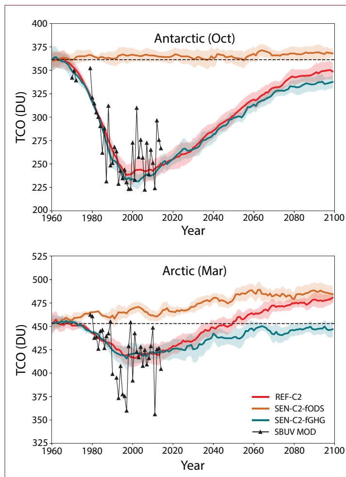
Figure 4-19. Temporal evolution of multi-model means (MMM1S) of total column ozone (in Dobson Units, DU) derived from REF-C2 (red), SEN-C2-fODS (brown), and SEN-C2-fGHG (green) CCMI scenario calculations for Antarctic spring (October, top panel) and Arctic spring (March, bottom panel). SEN-C2-fODS simulations use fixed ODS levels of the year 1960, while SEN-C2-fGHG simulations use fixed GHG levels of the year 1960. Black triangles indicate observations derived from SBUV MOD data. The black dashed lines denote the 1960 reference values for each region. Adapted from Dhomse et al. (2018).
