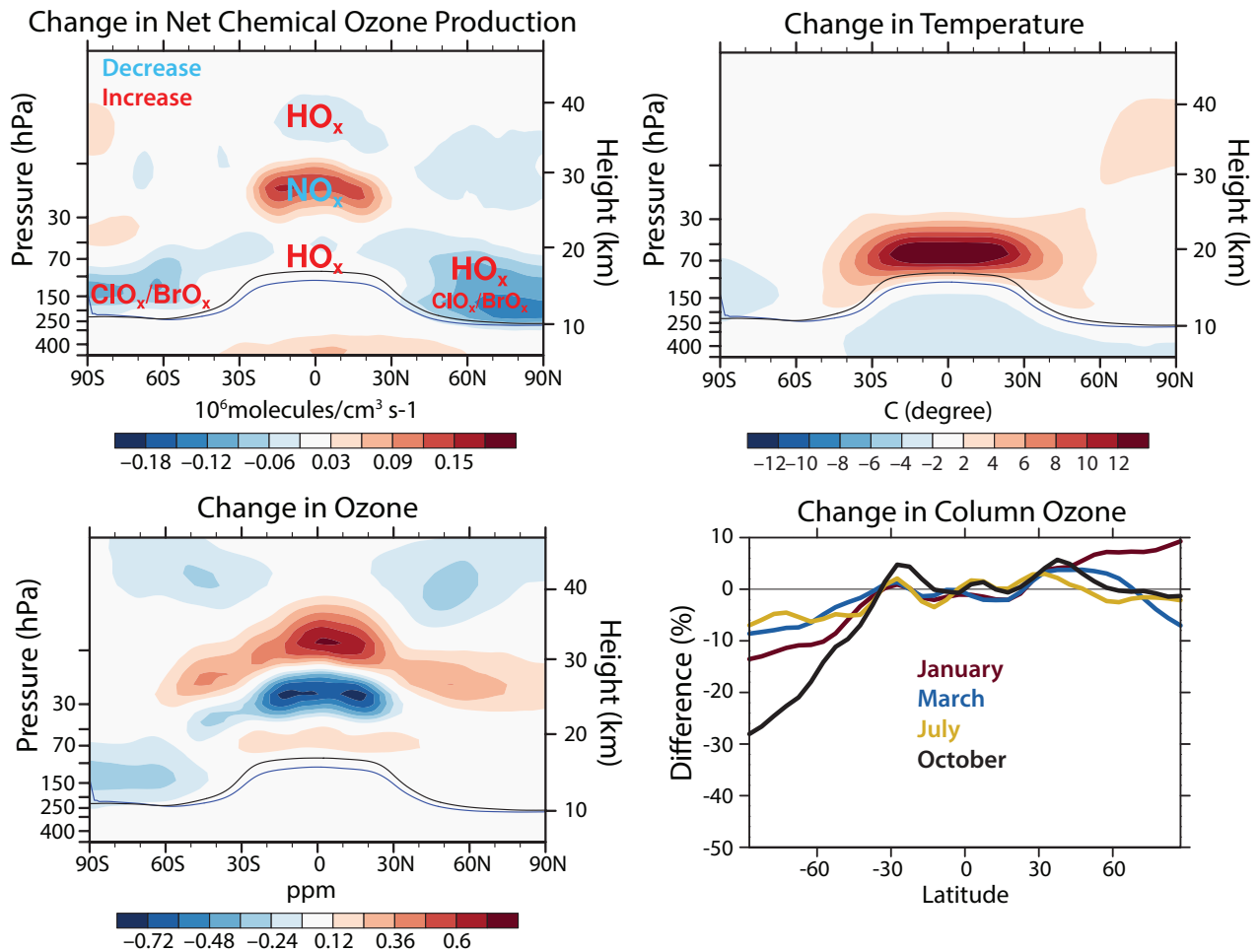
Figure 6A-1. Processes impacting stratospheric ozone in 2042–2049 following RCP8.5 for 16 Tg S yr -1 injections at 15°N/15°S. Impact of enhanced sulfate aerosols on zonal and annual averaged net rate of chemical production of ozone ( top left ), temperature ( top right ), and ozone concentration ( bottom left ). Changes in the dominant ozone loss cycles are shown in blue if decreasing (net chemical production is increasing) and in red if increasing (net chemical production decreasing) ( top left ). The example is based on a RCP8.5 control simulation between 2042 and 2049 and a geoengineering simulation with injection of 16 Tg S yr -1 evenly distributed between two single injection locations at 15°N and 15°S latitude, 180° longitude, and at 70 hPa (about 19 km) to counteract surface warming of about 2°C, using a fully interactive model, CESM1 (WACCM) (Richter et al., 2018; Tilmes et al., 2018). The tropopauses in the control and geoengineering simulations are shown by the black and blue lines, respectively. Changes in ozone concentration with geoengineering are driven mainly by dynamical changes, especially in the tropics and the Northern Hemisphere; changes in ozone concentration in polar regions mainly reflect enhanced chemical loss. Differences in column ozone (%) between the geoengineering and the control simulation in 2042–2049 are illustrated for different months ( bottom right ).
