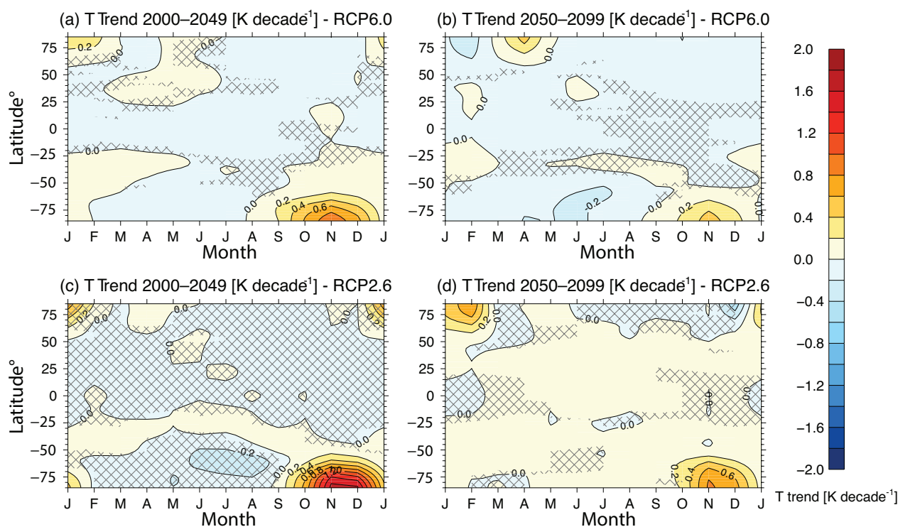
Figure 5-8. CCMI multi-model mean zonal-mean MSU4 channel (~13–22 km) temperature trends (K per decade) over the periods (a, c) 2000–2049 and (b, d) 2050–2099 under (a, b) the medium-to-high greenhouse gas (GHG) scenario (RCP-6.0; 12 models) and (c, d) the low GHG scenario (RCP-2.6; 4 models). Regions where less than two-thirds of the models agree on the sign of the trend are hatched. Based on model simulations described in Morgenstern et al. (2017) and Maycock et al. (2018).
