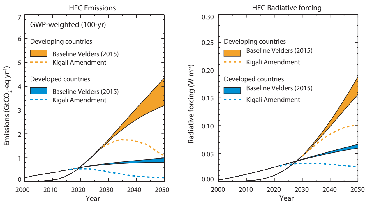
Figure 2-19. Response of HFC emissions ( \text{GtCO}_2\text{-eq yr}^{-1} ) and radiative forcing in the baseline scenario (Velders et al., 2015) for developed and developing countries to implementation of the Kigali Amendment to the Montreal Protocol (excluding HFC-23). Extending the scenarios beyond 2050 under the same assumptions gives a radiative forcing for the baseline scenario of 0.07\text{--}0.12 \text{ W m}^{-2} and 0.40\text{--}0.65 \text{ W m}^{-2} in 2100 for the developed and developing countries, respectively. The 2100 radiative forcing under the Kigali Amendment is 0.01 \text{ W m}^{-2} and 0.06\text{--}0.07 \text{ W m}^{-2} for the developed and developing countries, respectively. The emissions and radiative forcing shown here are based on the GWPs and radiative efficiencies used in Velders et al. (2015), which differ somewhat from those in Table 2-2.
