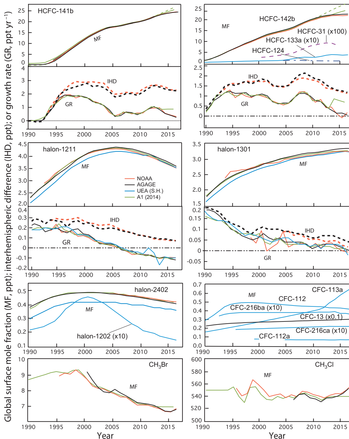
Figure 1-1. Annual mean global surface mole fractions (MF; expressed as dry air mole fractions in parts per trillion or ppt) of ozone-depleting substances from independent sampling networks and from scenario A1 of the previous Ozone Assessments over the past 26 years (1990–2016) (Daniel and Velders, 2011; Harris and Wuebbles et al., 2014). The baseline scenarios from previous Assessments (A1-2010, A1-2014) are projections from 2009 and 2013, respectively. Only A1-2014 data are shown for some species. Shown are measured global surface annual means from the NOAA network (red) and AGAGE network (black). Southern Hemispheric data obtained by the University of East Anglia (UEA) (blue) are shown for some species. NOAA and AGAGE CFC-113 data likely represent some combination of CFC-113 and CFC-113a (although the influence of CFC-113a on NOAA and AGAGE measurements of CFC-113 is likely small), whereas UEA measures CFC-113 and CFC-113a separately (Adcock et al., 2018). UEA CFC-113 data (annual Southern Hemispheric means from Adcock et al., 2018) were adjusted downward by 2% to be consistent with the NOAA scale determined by gas chromatography-mass spectrometry (GC-MS) as opposed to gas chromatography-electron capture detection (GC-ECD). HCFC-124 data were taken from Simmonds et al. (2017). HCFC-31 data were taken from Schoenenberger et al. (2015). For some gases, we also show growth rates (GR) and interhemispheric differences (IHD; NH mean minus SH mean) in a second panel, using the same color scheme as in the corresponding upper panel.
