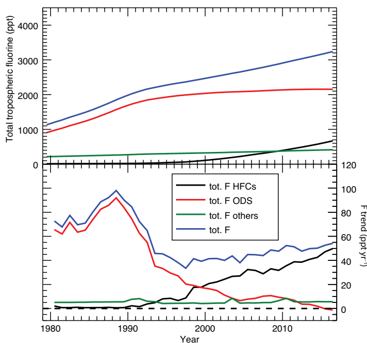
Figure 1-19. Tropospheric total fluorine time series and annual changes from long-lived gases, separated by contributions due to ODS, HFCs (see Chapter 2 ), and other fluorinated gases (such as SF 6 , NF 3 , and CF 4 ). ODS mole fractions were derived from a merged dataset based on NOAA, AGAGE, and UEA data. HFC mole fractions were derived from AGAGE and NOAA data. HFC records prior to regular global measurements were supplemented with estimates from Miller et al. (2010); Mühle et al. (2010); O'Doherty et al. (2009); Oram et al. (1996); Simmonds et al. (1998); Vollmer et al. (2011); and Weiss et al. (2008).
