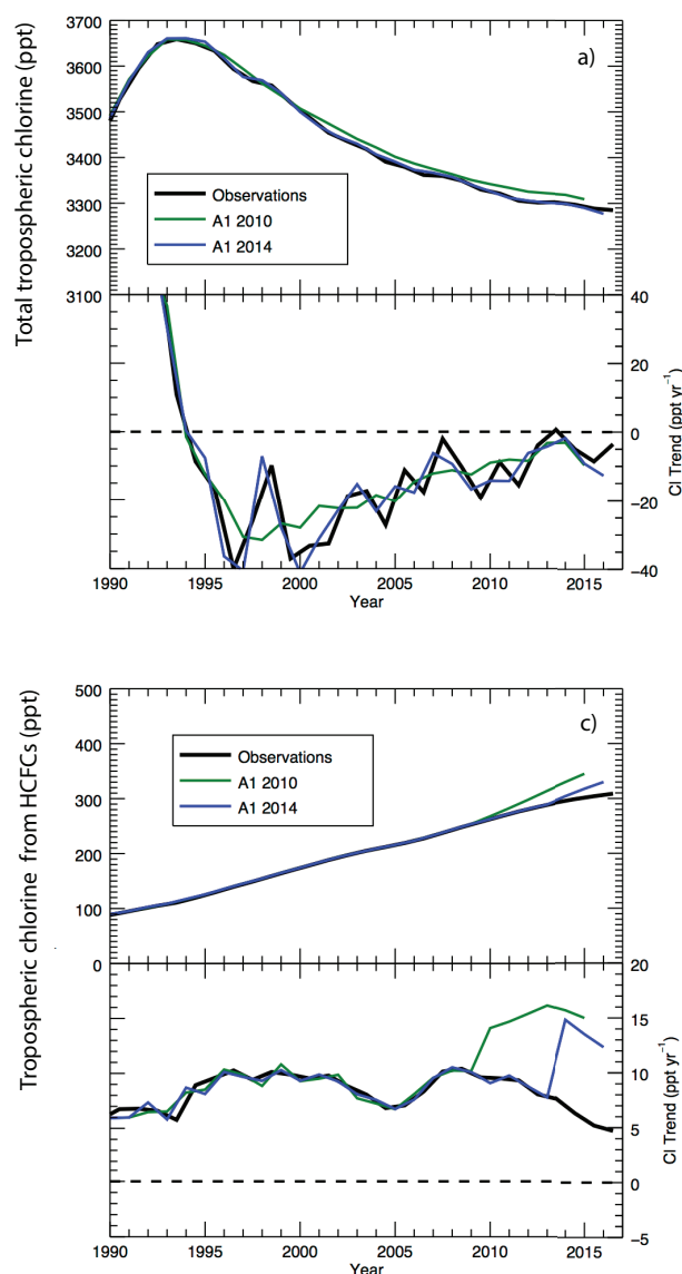
Figure 1-12. (a) Total tropospheric organic chlorine from the combined global measurement networks, based mainly on NOAA and AGAGE data (black line) in comparison to the A1 scenarios from the 2010 (green line) and 2014 (blue line) Assessments. Quantities are based on global mean mole fractions of CFC-11, CFC-12, CFC-113, CH 3 CCl 3 , CCl 4 , CH 3 Cl, HCFC-22, HCFC-141b, HCFC-142b, and halon-1211 determined by the respective networks. CFC-114, CFC-115, CFC-112, CFC-13, and CFC-113a are estimated from measurements of Cape Grim archive air samples (Laube et al., 2014; Newland et al., 2013). Organic chlorine also includes contributions from VSL SG, in particular CHCl 3 , CH 2 Cl 2 , and C 2 Cl 4 (see also Table 1-6). Observations of these gases are only available back to the mid-1990s. Before that, constant mixing ratios are
