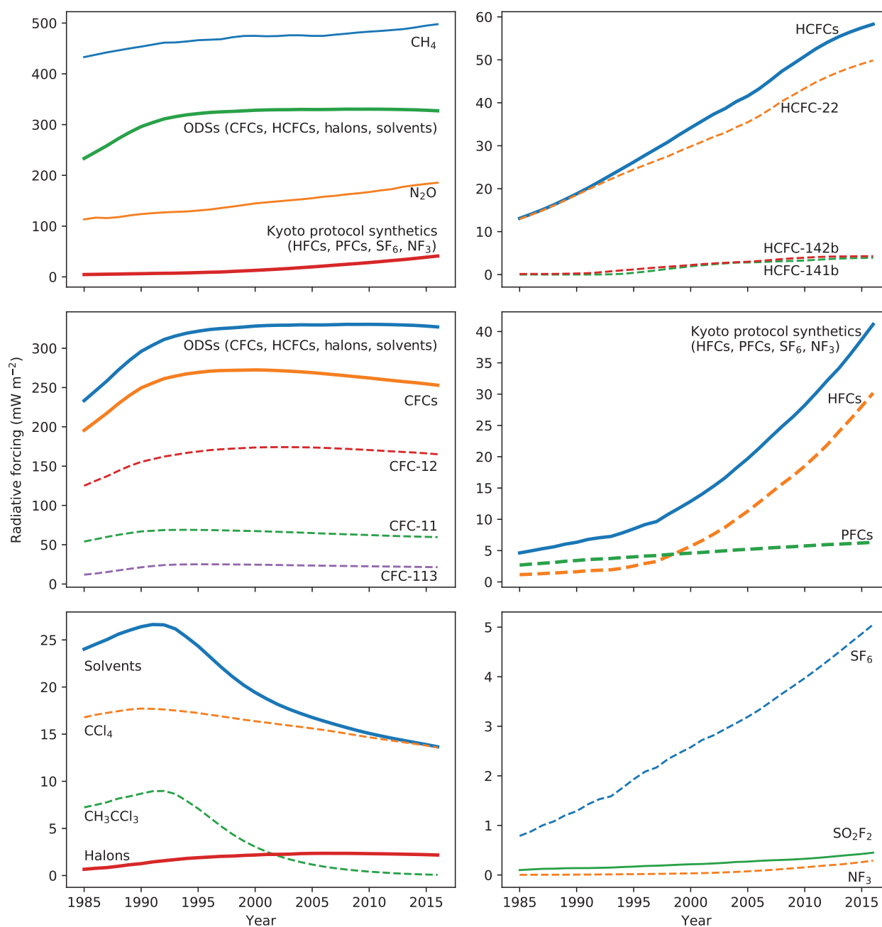
Figure 1-3. Direct radiative forcing due to ODSs, HFCs, \text{CH}_4 , \text{N}_2\text{O} , and other greenhouse gases. Selected groupings of gases are shown in bold and selected compounds or collections of compounds that fall within these groupings are shown as dashed lines. The ODS group here refers to combined CFCs, HCFCs, halons, and solvents ( \text{CCl}_4 and \text{CH}_3\text{CCl}_3 ). Kyoto protocol synthetics are defined as HFCs (see Chapter 2 ), perfluorocarbons (PFCs, which include \text{CF}_4 and \text{C}_2\text{F}_6 ), \text{SF}_6 , and \text{NF}_3 ( Section 1.5 ). Lower tropospheric annual mean mole fractions were taken from AGAGE data ( Table 1-1 , Figure 1-1 ). Radiative forcing was calculated using the expressions in Ramaswamy et al. (2001), with radiative efficiencies as summarized in Table A-1 and preindustrial global surface mean mole fractions of 722 ppb, 270 ppb, and 36 ppt for \text{CH}_4 , \text{N}_2\text{O} , and \text{CF}_4 , respectively. For comparison, the radiative forcing due to \text{CO}_2 was approximately 2 \text{ W m}^{-2} in 2016.
