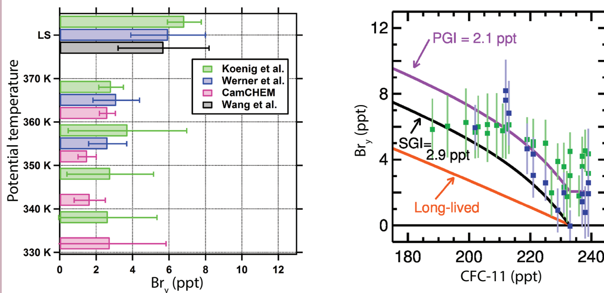
Figure 1-11. Left panel: Vertical variation of inferred inorganic bromine ( Br_y ) from VSLs within the TTL during the CONTRAST and ATTREX missions (adapted from Koenig et al., 2017). Right panel: SGI and PGI inferred from the correlation between stratospheric VSLs and CFC-11 measured in the Tropical Western Pacific. Inferred Br_y from DOAS (green) and CIMS (blue) instruments are shown, together with the tracer-tracer correlation for VSL SGs (black line) and the SGI + PGI best estimation (purple line). Modified from Wales et al. (2018).
