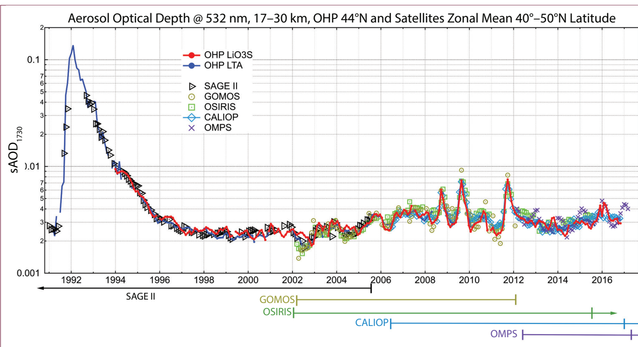
Figure 3-6. Time series of monthly mean stratospheric aerosol optical depth between 17- and 30-km altitude ( sAOD_{1730} ) from OHP lidars and monthly and zonal mean sAOD_{1730} within 40–50°N from satellite sounders. From Khaykin et al. (2017).
