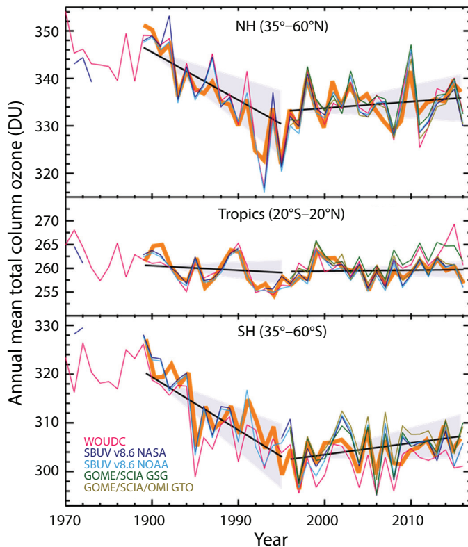
Figure 3-11. Annual mean total ozone time series of five bias-corrected, merged datasets in the 35°–60°S, 35°–60°N and 20°S–20°N latitude bands. The thick orange lines are the result from applying a multiple linear regression (MLR) model. The solid black lines indicate the linear trends before and after the ODS peak in 1997, respectively. The shaded areas show the 2\sigma uncertainty of the MLR trend estimates. Adapted from Weber et al. (2018).
