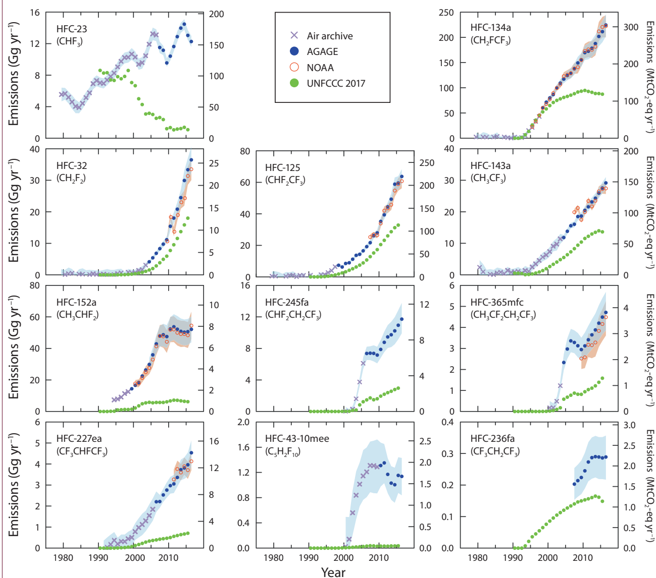
Figure 2-1. Total global emissions estimated from a budget analysis of atmosphere measurements at remote sites (those in Figure 2-2 ) compared to total emissions reported to UNFCCC (2017). Atmospheric measurement-based emissions are derived with a 12-box model and the lifetimes in Table 2-2 ; the methods and model used here are discussed by Rigby et al. (2014). Emissions are presented in units of Gg compound yr -1 on the left-hand axis, and the right-hand axis has been scaled by chemical-specific 100-yr GWPs ( Table 2-2 ) to indicate emission magnitudes in MtCO 2 -eq yr -1 (1 Mt = 10 12 g). Shaded regions represent 1 standard deviation in global emissions derived from measured mole fractions and a 12-box model (Rigby et al., 2014). Uncertainties in mole fractions and their model representation are propagated through to the posterior emissions estimates using a Bayesian framework. These uncertainties are augmented by lifetime and calibration scale uncertainties following Rigby et al. (2014). The model uses interannually repeating meteorology and, therefore, errors may be underestimated for periods with large circulation changes, although this will likely affect short-term (e.g., annual) variations more than long-term trends.
