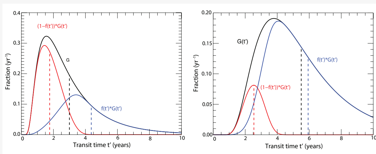
Box 1-4 Figure 1. Age spectra G (black line) for an inert tracer compared to the transit time distributions weighted with chemical loss (red and blue line) for a mean age of 3 years (a), and 5.5 years (b). The red line represents the transit time distribution for the remaining organic fraction of a source gas; the blue line represents the fraction which has been released and is thus in the inorganic form. The loss function has been approximated as a function of transit time in order to represent a tracer similar to CFC-11 (Engel et al., 2018). The first moments of the three functions differ substantially: the first moment of the red curve (representing the remaining organic fraction) is younger, and that of the blue curve (describing the inorganic halogen released from the source gas) is older than the mean age value. Note that this figure is purely for illustrative purposes, as the loss function has been approximated.
