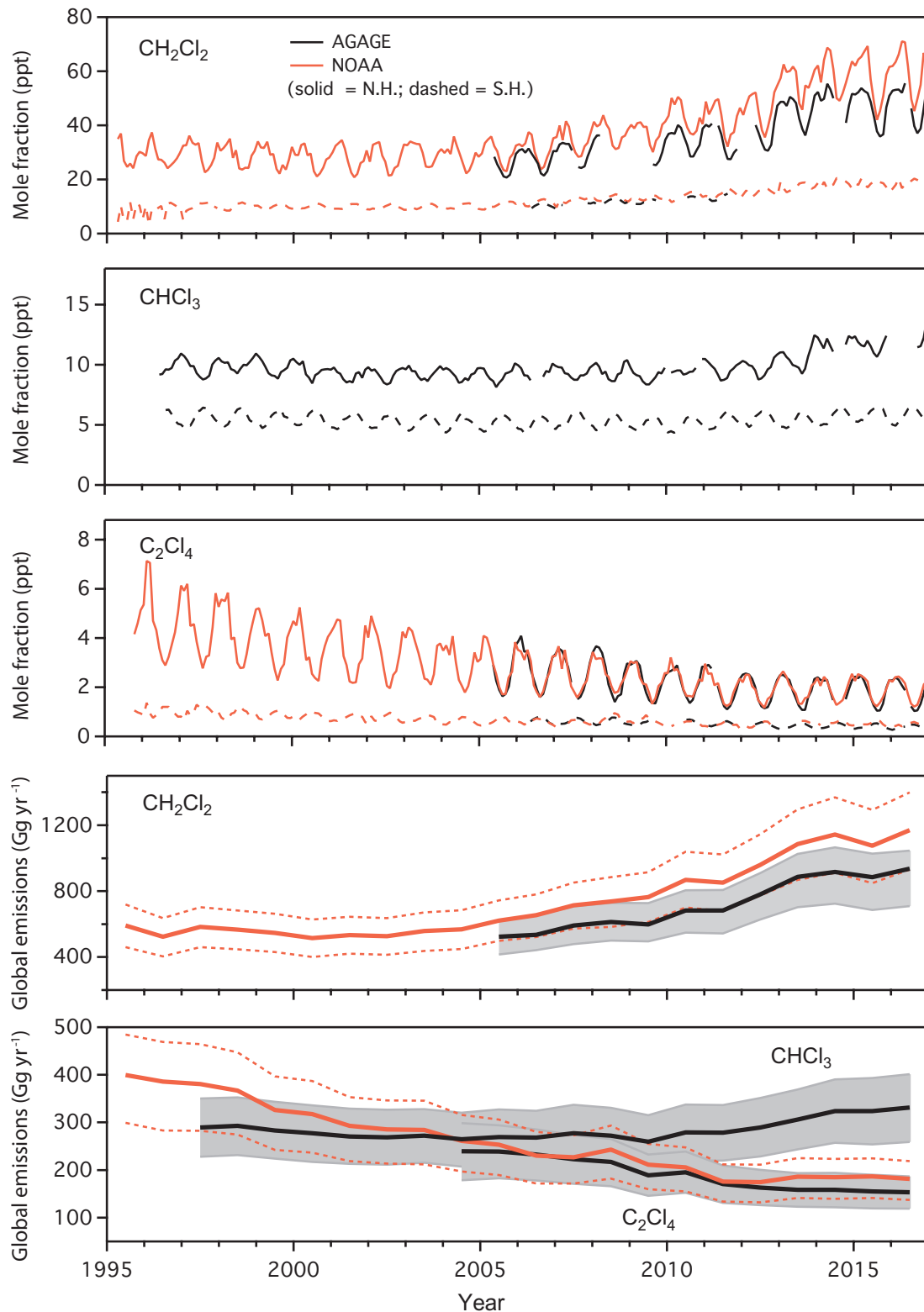
Figure 1-8. Upper three panels: Monthly hemispheric mean mole fractions of \text{CH}_2\text{Cl}_2 , \text{CHCl}_3 , and \text{C}_2\text{Cl}_4 derived from AGAGE (black) and NOAA (red) observations in the NH (solid lines) and SH (dashed lines). Lower two panels: Global emissions estimates ( \text{Gg yr}^{-1} ) calculated using a global 12-box model (using methods described in Box 1-1 and Figure 1-4), with 1-sigma uncertainties indicated by shading (AGAGE) or dotted lines (NOAA).
