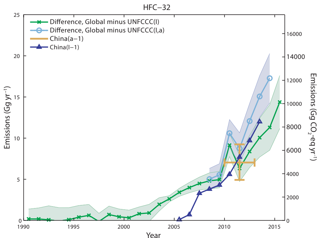
Figure 2-8. As in Figure 2-6 , but for HFC-32. Here Chinese emissions are from inventory-based (Fang et al., 2016; I-1, blue triangles) and atmosphere-based (Lunt et al., 2015, a-1, yellow) estimates.
