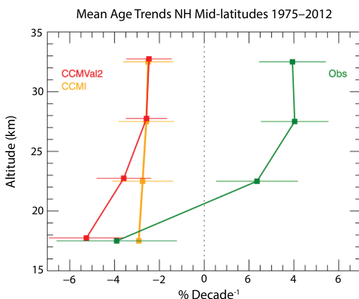
Figure 5-9. Profiles of trends in the Northern Hemisphere (NH) mid-latitude mean age of air (in percent per decade) from 1975 to 2012. Green symbols are trends derived from in situ tracer observations combined with a simple mechanistic model. Red symbols represent average trends from four ocean-coupled CCM-Val2 models. Orange symbols represent average trends from nine ocean-coupled CCMI models. Error bars represent the standard deviation of the mean of all model trends at each level and, for observations, the 1\sigma uncertainty on the trend estimate at each level. Update to Ray et al. (2014).
