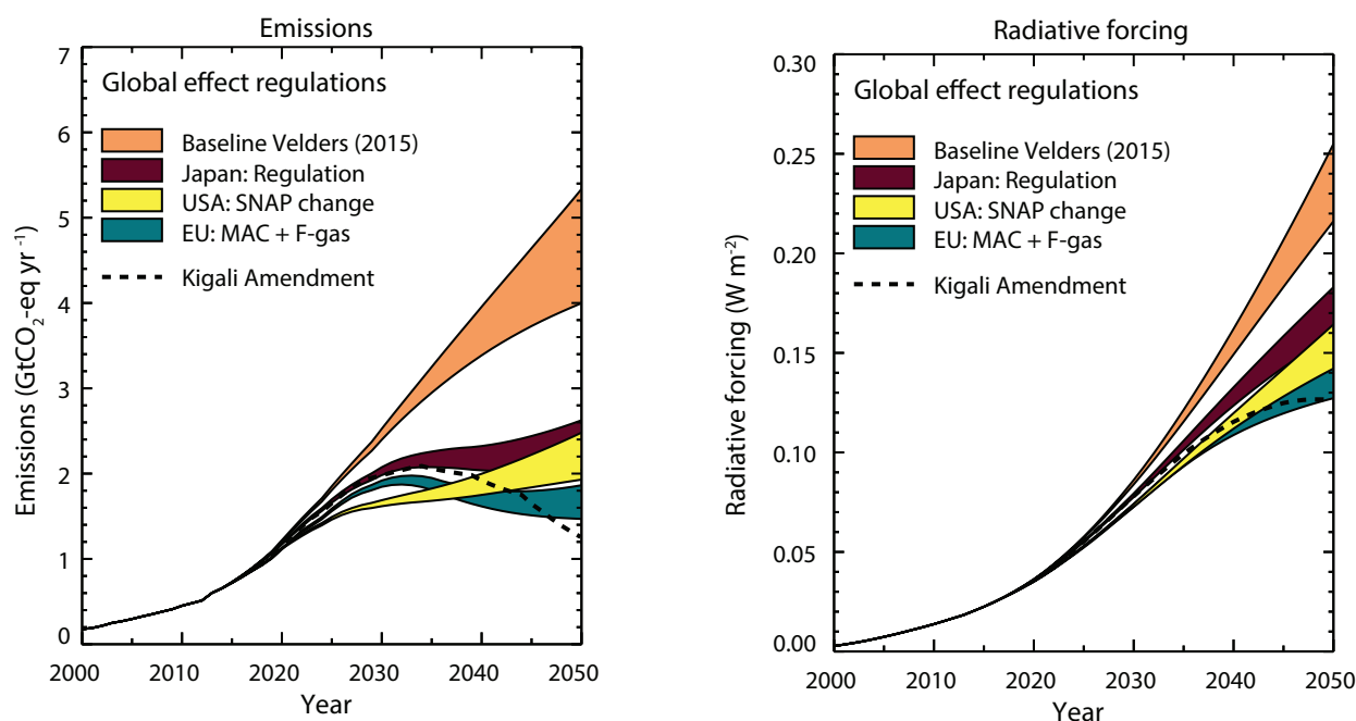
Figure 2-18. Response of global HFC emissions ( \text{GtCO}_2\text{-eq yr}^{-1} ) and global radiative forcing ( \text{W m}^{-2} ) in the baseline scenario of Velders et al. (2015) to global implementation of three national regulations and of the Kigali Amendment (HFC-23 not included). In each case, the national regulation is applied to all countries, with a 5-year delay of the regulations for developing countries. The emissions and radiative forcing shown here are based on the GWPs and radiative efficiencies used in Velders et al. (2015), which differ somewhat from those in Table 2-2. (Note: see Section 2.5.1.2 for the status of the HFC regulations under SNAP).
