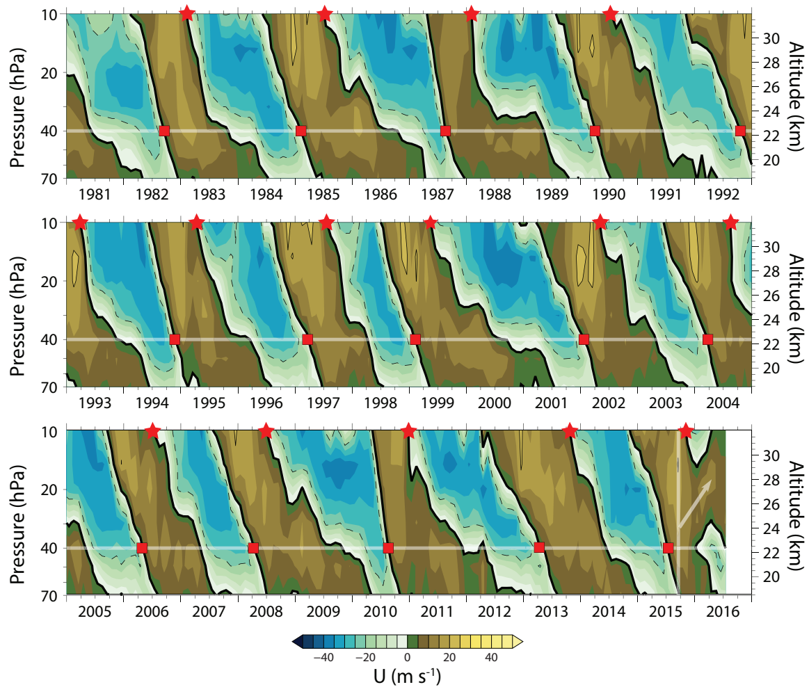
Figure 3-4. Monthly mean zonal wind U ( \text{m s}^{-1} ) derived from Singapore radiosondes ( 1^\circ\text{N} , 104^\circ\text{E} ) between 70 and 10 hPa for 1981 through July 2016. Easterlies are shown in cyan/blue, while westerlies are shown in green/brown. Contours are every 20 \text{ m s}^{-1} , with easterlies dashed and westerlies solid, and a thick black line for zero wind. The red squares show the dates of the 40 hPa easterly-to-westerly transition, while the red stars show the dates of the 10 hPa westerly-to-easterly transition. From Newman et al. (2016).
