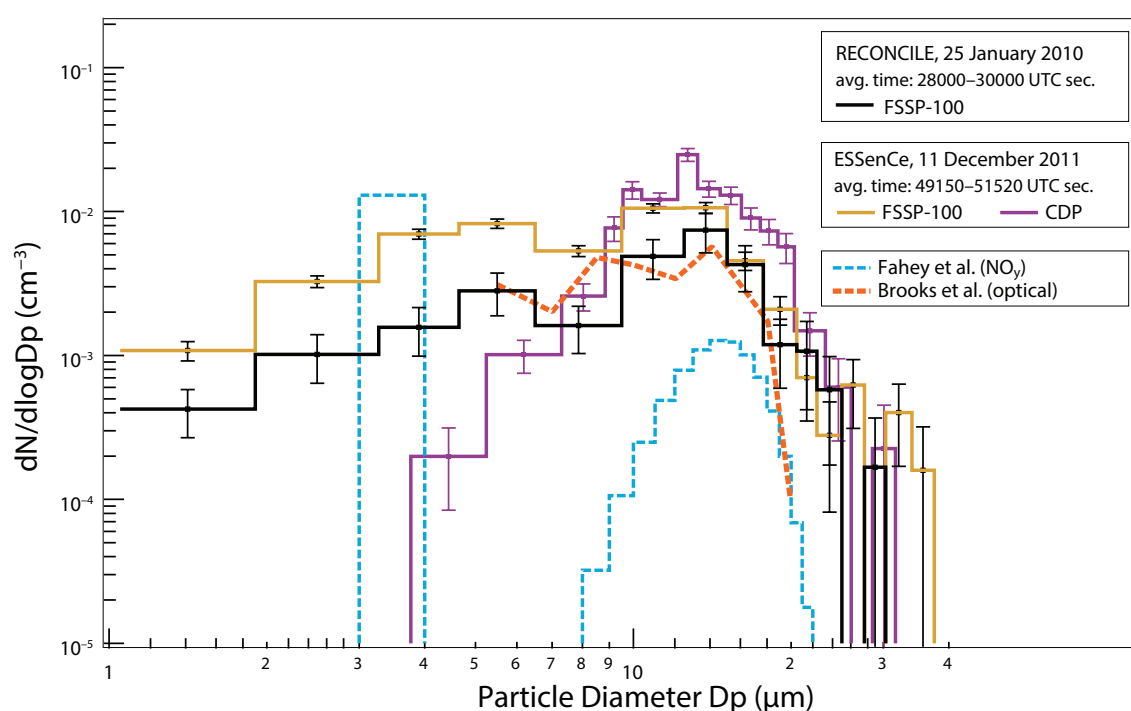
Figure 4-10. Size distributions of large \text{HNO}_3 -containing PSC particles with high number densities from in situ airborne measurements in 2010 and 2011. These measurements are compared to previous measurements by Fahey et al. (2001) (retrieved from total \text{NO}_y ) and Brooks et al. (2003) (optical measurements). Adapted from Molleker et al. (2014).
