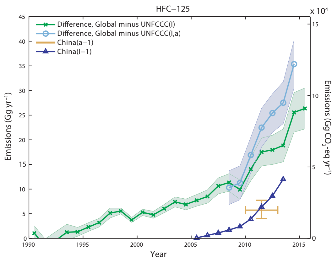
Figure 2-9. As in Figure 2-8, but for HFC-125.
