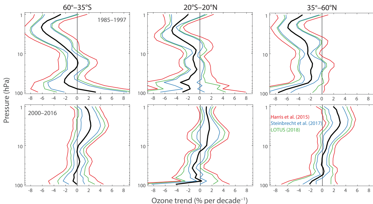
Figure 3-20. Combined trends of six satellite data records with 2\sigma uncertainties for the pre-1997 period (top row) and the post-2000 period (bottom row) from the LOTUS analysis for three latitude bands 35°–60°S (left column), 20°S–20°N (center column) and 35°–60°N (right column). Central trend estimates are identical for all methods (black lines). Green lines represent uncertainties calculated using the LOTUS method (Equation 5.1 in LOTUS, 2018); Blue lines represent the method of Steinbrecht et al. (2017) with the number of independent datasets estimated as 2 for pre-1997 and 3 for post-2000 trends; and red lines represent the J-distribution method used by Harris et al. (2015). Results shown here for the latter two methods were obtained using formulae that were modified to use an unbiased estimator of sample variance. Adapted from LOTUS (2018).
