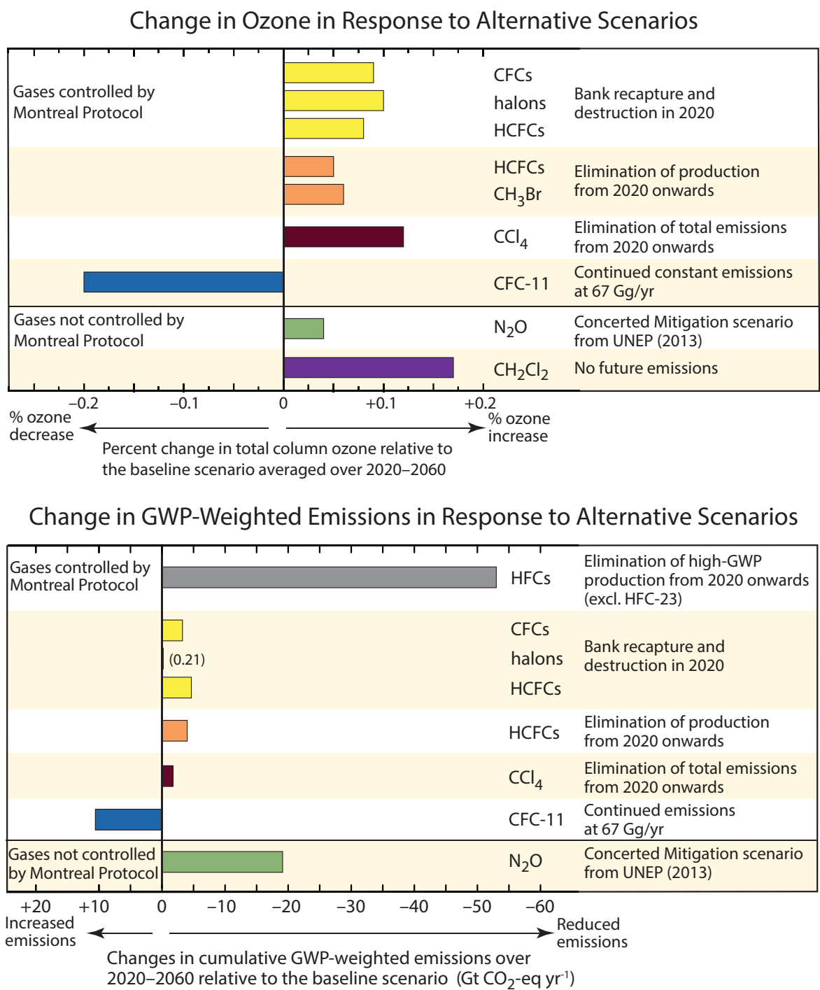
Figure 6-1. Ozone and climate-relevant impacts of alternative future scenarios compared with the baseline scenario. The climate-relevant metric is chosen to be the integrated GWP-weighted emission from 2020 to 2060, and the ozone-relevant metric is the percentage change in total column ozone averaged over 2020 to 2060. A decrease in total ozone and an increase in GWP-weighted emissions occur when future emissions are higher than in the baseline scenario for the compounds considered. Numerical values of these changes are shown in Table 6-5 .
