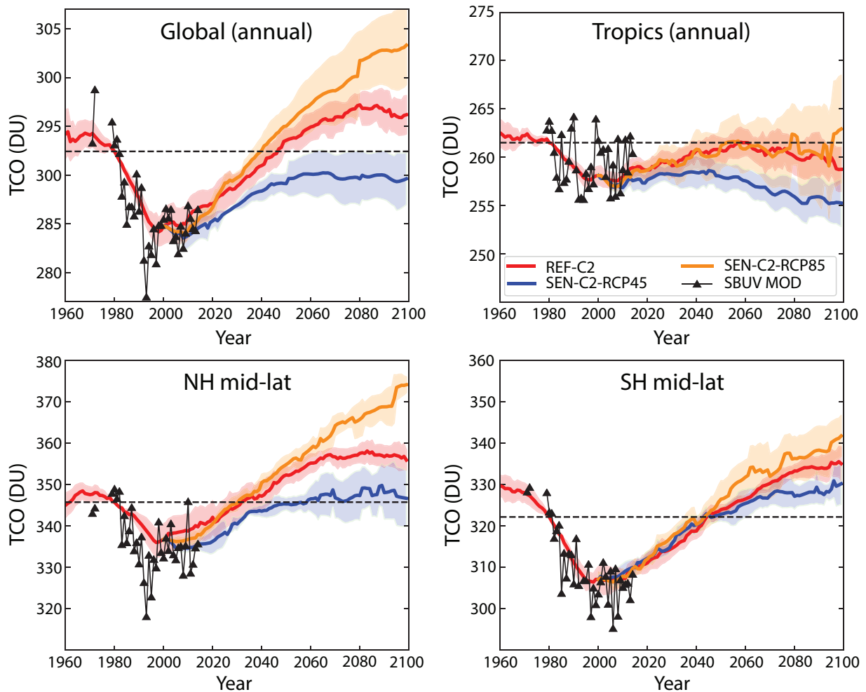
Figure 3-29. Adjusted and smoothed multi-model mean time series of annual mean TCO from observations (solid black lines and symbols) and for RCP scenarios from CCMI models: REF-C2=RCP-6.0 (red lines), SEN-C2-RCP45=RCP-4.5 (blue lines), and SEN-C2-RCP85=RCP-8.5 (orange lines). The black dashed lines represent 1980 values of TCO. From Dhomse et al. (2018).
