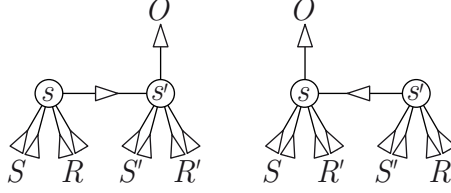
FIGURE 3. Two adjacent maximal \mathbf{B} -trees \mathsf{T} (left) and \mathsf{T}' (right).
