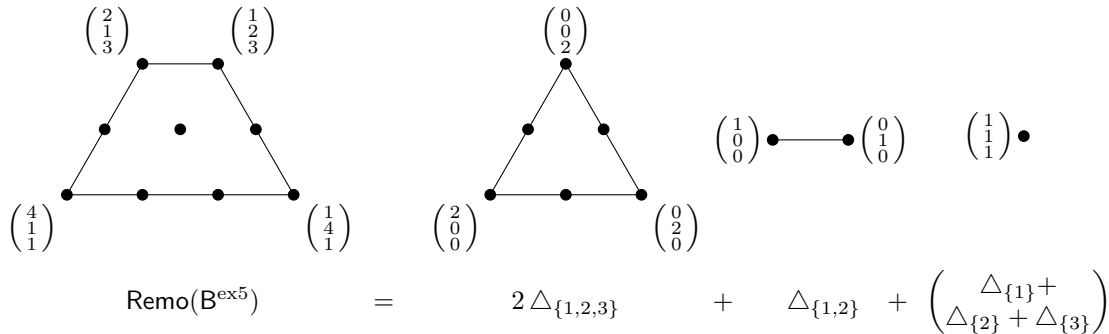
FIGURE 4. The Minkowski decomposition of the 2-dimensional removehedron \text{Remo}(\mathbf{B}^{\text{ex5}}) into faces of the standard simplex.
