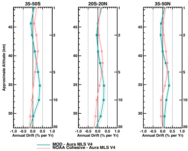
Figure 3.10: Drift (in % per year) of zonally averaged profile data from SBUV MOD (turquoise) and SBUV COH (red) relative to Aura MLS v4 for 50°S–35°S (left), 20°S–20°N (middle) and 35°N–50°N (right).
