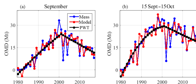
Figure 11. OMD (in Mt) computed from total columns of MSR-2 dataset lower than 220 DU and south of 60^\circ \text{S} for September (a) and 15 September–15 October (b). Regressed values by MLR analysis using GRAD, HF and PWT are also shown as well as the fitted PWT proxy.
