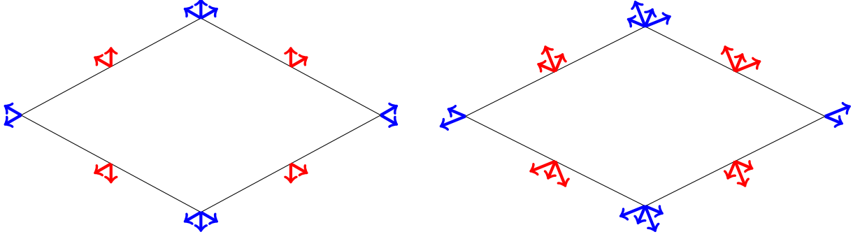
FIGURE 6. The sets R(F) for the faces F of the cube in type A_2 (left) and B_2 (right). Note that positive roots point downwards.
