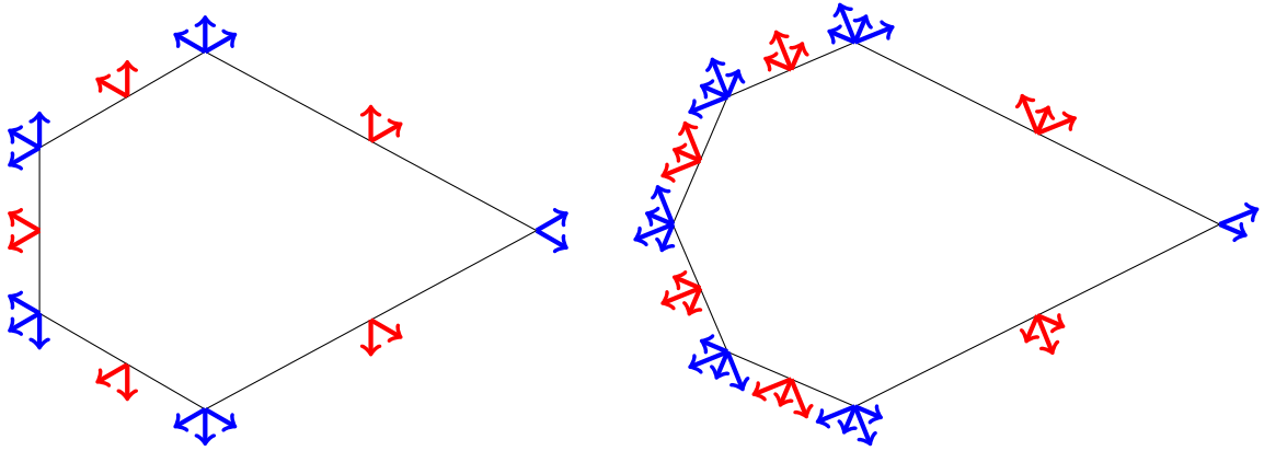
FIGURE 5. The sets R(F) for the faces F of the c -associatedhedron in type A_2 (left) and B_2 (right). Note that positive roots point downwards.
