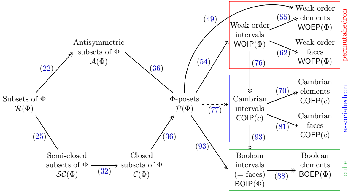
FIGURE 3. A roadmap through the different families of subsets of roots studied in this paper. An arrow \rightarrow indicates a subposet, while an arrow \dashrightarrow indicates a sublattice. The dashed arrow is a conjectural sublattice relation. The label on each arrow refers to the corresponding statement in the paper.
