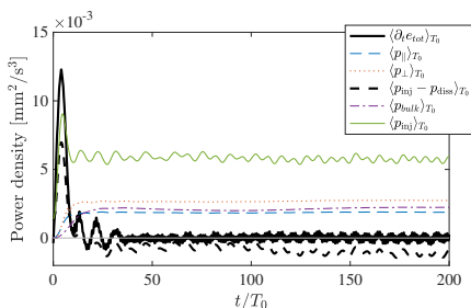
FIGURE 11. Evolution of the derivative of total energy, injected power and the different dissipative terms in time, for a linear experiment with forcing amplitude a_0 = 5 mm in the 3D tank. Note the 10^{-3} factor on the y -axis. The field had been filtered around the forcing frequency before computing these quantities.
