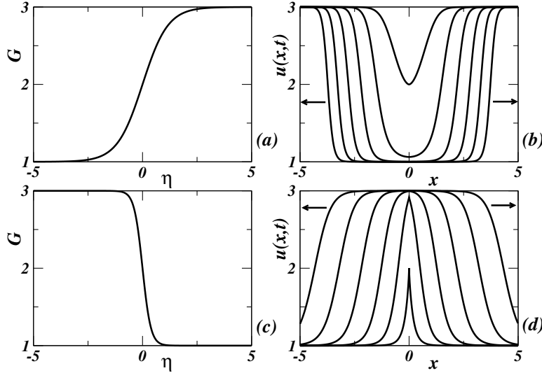
FIG. 1. Panels (a)-(b): s = 2.75 , with G(\eta) vs \eta in (a) and u(x, t) for different times t = 0, 2, 4, 6, 8, 10 . The values of A and |C - A| are 2 and 1, respectively. Panels (c)-(d): s = 1.75 , with G(\eta) vs \eta in (c) and u(x, t) for different times t = 0, 0.6, 1.2, 1.8, 2.4, 3 (again with A = 2 and |C - A| = 1 ). \chi and \gamma are constants of order unity.
