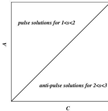
FIG. 2. Representation of the phase diagram in the (A, C) plane with: i ) for 1 < s < 2 anti-kink solutions for the G , the corresponding counterpart for the field u being pulse solutions; ii ) for 2 < s < 3 kink solutions for the G , corresponding to anti-pulse solutions for the field u .
