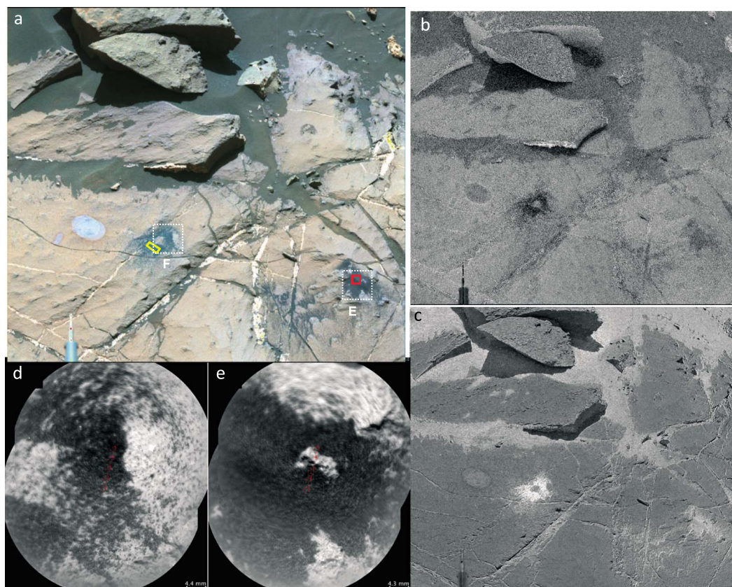
Figure 21. (a) False-color M34 image (751, 527, and 445 nm) of Dump piles E and F from Sol 1253 (mcam05852). Regions of interest from which Mastcam spectra were acquired (Figure 22) shown by boxes (red = Dump E; yellow = Dump F). Dotted white lines are approximate outlines of RMI mosaics. Bluish oval on bedrock to left of Dump F is brushed target “Kuisseb.” (b) 527 nm band depth mosaic. (c) 640/1012 nm ratio (using red Bayer filter and L6 filter). (d) RMI mosaic of Dump F. (e) RMI mosaic of Dump E. Dump F has a weak 527 nm band depth (dark tones) and strong 640/1012 nm ratio (light tone) compared to Dump E, consistent with its less ferric nature.
