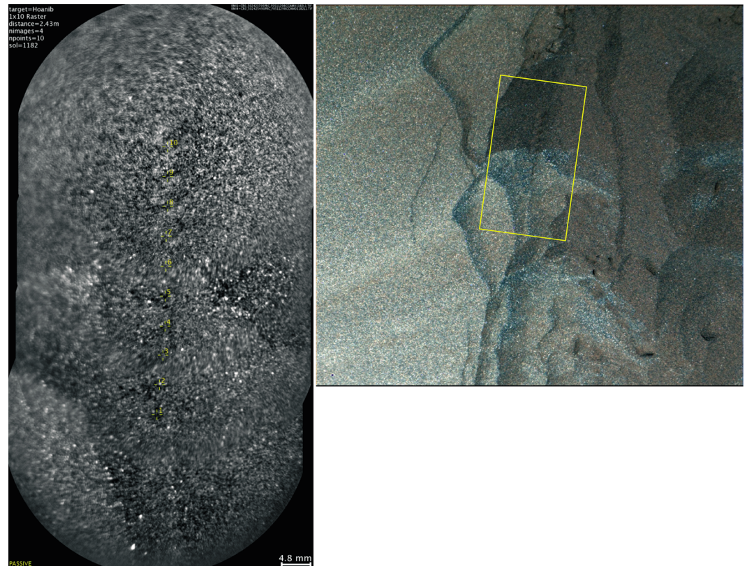
Figure 6. RMI mosaic of Hoanib (Sol 1182; ccam01182) showing 10 numbered locations of ChemCam observations and post-LIBS Mastcam M100 enhanced color image (Sol 1182, mcam05359); yellow box approximates extent of RMI mosaic.
