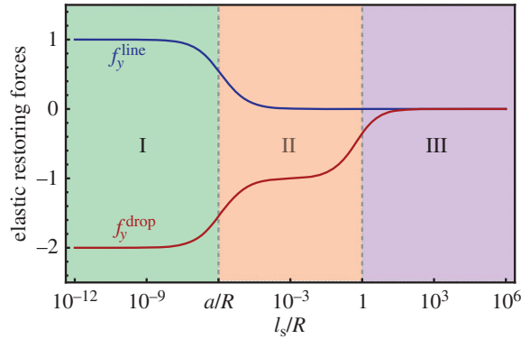
Figure 7. Total elastic force under the contact line ( f_y^{\text{line}} ) and under the rivulet ( f_y^{\text{drop}} ) as a function of the dimensionless parameter l_s/R . The elastic restoring forces are scaled by \gamma_{LV} \sin \theta_{LV} . The Neumann model is recovered in the limit l_s/R \rightarrow \infty . (Online version in colour.)
