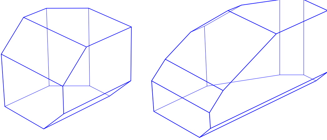
FIGURE 3. The associahedra \text{Asso}(\text{B}_o) for the type A_3 (left) and type C_3 (right) cyclic initial exchange matrices.
