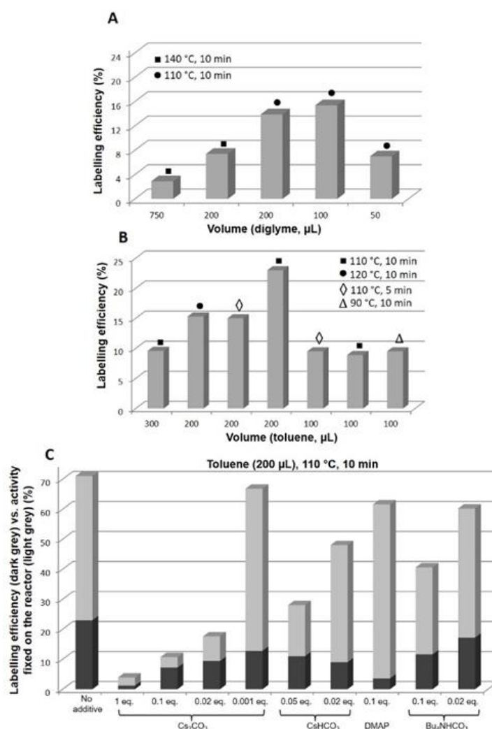
Figure 5. Influence of: (i) the temperature, concentration (13 \mu\text{mol} of 6b in various volumes of solvent) and reaction time on the radiolabelling efficiency in diglyme (A) or toluene (B) and (ii) the addition of traces of mineral or organic bases in the reactor (C), % were calculated based on the starting [^{18}\text{F}]\text{F}^- activity; purity of the eluted compound was controlled by radio-TLC (>98%).
