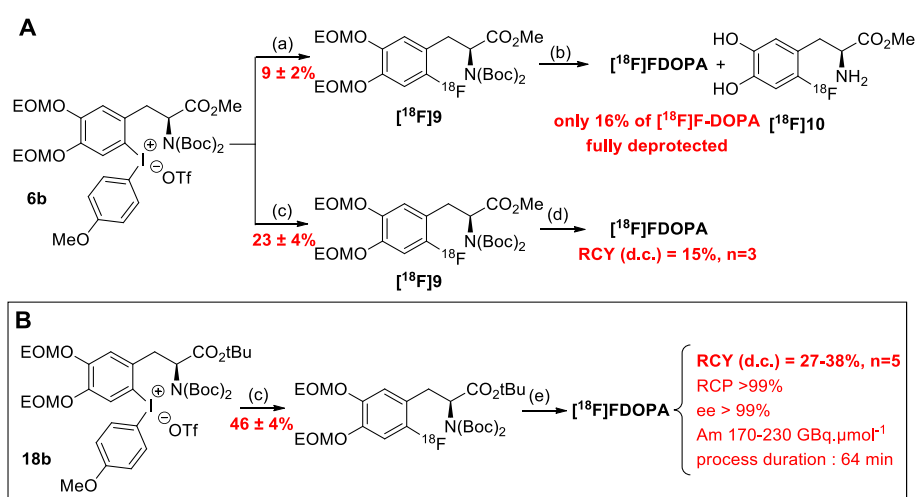
Scheme 3. A: In house preparation of [ 18 F]FDOPA from 6b following Kuik et al. [11] protocol compared to our radiosynthetic approach; B: Preparation of [ 18 F]FDOPA from tert -butyl ester precursor 18b with our optimized protocol. Reagents and conditions: (a) [ 18 F]KF-crypt-222-carbonate, diglyme, 140 °C, 5 min; (b) aq. H 2 SO 4 3 M, 140 °C, 5 min; (c) [ 18 F]F - , toluene, 105-110 °C, 10 min; (d) aq. HBr conc., 140 °C, 10 min; (e) aq. HCl conc., 120 °C, 7 min. EOM: ethoxymethyl.
