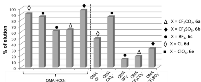
Figure 3. Percentages (%; ratio between values of activity measured in the eluate and initially loaded onto the QMA cartridge, n = 2 , except for QMA- \text{HCO}_3^- , X = \text{CF}_3\text{SO}_3^- : n = 41 ) of [^{18}\text{F}]\text{F}^- elution from QMA- \text{HCO}_3^- or QMA cartridges preconditioned with corresponding anions depending on the counterion of the iodonium salt used (13 \mu\text{mol} in 750 \mu\text{L} of methanol).
