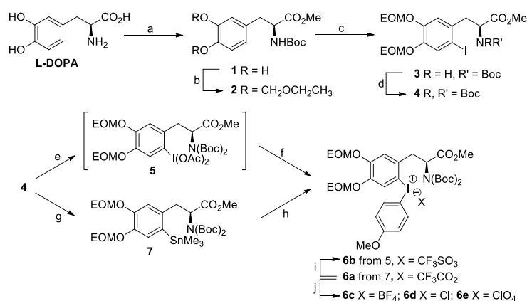
Scheme 1. Preparation of diaryliodonium salts 6a-e . Reagents and conditions: (a) i) MeOH, SOCl 2 , 0 °C then reflux, 16 h; ii) (Boc) 2 O, THF, sat. aq. NaHCO 3 , RT, 2 h, 95%; (b) C 2 H 5 OCH 2 Cl, DIPEA, THF, 0 °C then 40 °C, 15 h, 99%; (c) I 2 , K 2 CO 3 , Ph(OCOCF 3 ) 2 , CH 2 Cl 2 , RT, 2.5 h, 74%; (d) NEt 3 , DMAP, (Boc) 2 O, MeCN, RT, 29 h, 86%; (e) Selectfluor, TMSOAc, MeCN, RT, 6.5 h; (f) i) TMSOCOCF 3 , p -MeOPhBF 3 K, MeCN, RT, 10 min; ii) 0.5 M aq. NaOAc/AcOH buffer (pH 5); iii) aq. NaPF 6 , MeCN, RT; iv) IRA-400 (TfO - ) ion-exchange resin, 36%; (g) Sn 2 Me 6 , Pd(PPh 3 ) 4 , 1,4-dioxane, reflux, 1.5 h, 91%; (h) i) p -MeOPh(IOAc) 2 , CH 2 Cl 2 , -40 °C, 1 h; ii) TFA, -40 °C then RT, 5 h, 74%; (i) 1 M aq. NaOTf, CH 2 Cl 2 , RT, 85%; (j) 1 M aq. NaOTf, NaBF 4 , NaCl or NaClO 4 , CH 2 Cl 2 , RT, 87-95%. EOM: ethoxymethyl.
