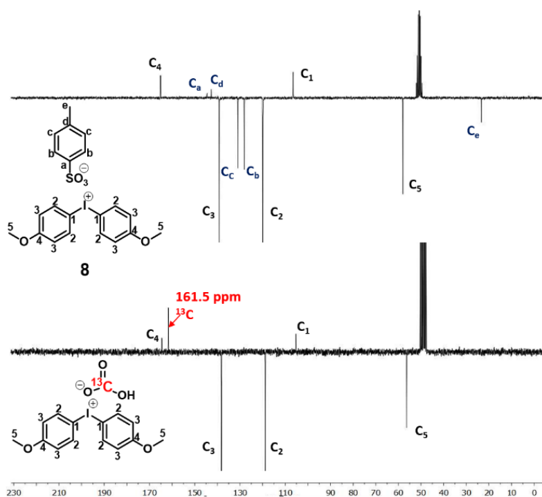
Figure 4. Comparison of 13 C NMR spectra of starting iodonium salt 8 and eluate obtained after elution of a 13 C-enriched QMA-HCO 3 - cartridge with 5 μmol of 8 showing the complete conversion of the tosylate derivative into its HCO 3 - analogue.
