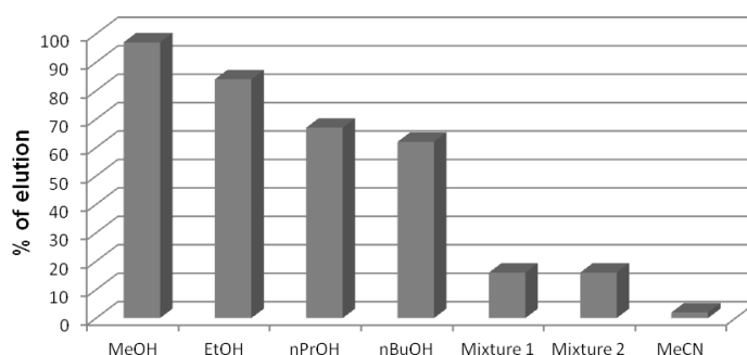
Figure 2. Percentages (% , ratio between values of activity measured in the eluate and initially loaded onto the QMA cartridge, n = 2 except for MeOH: n = 41 ) of [^{18}\text{F}]\text{F}^- elution from QMA- \text{HCO}_3^- cartridges depending on the solvent used for dissolution of the iodonium salt 6b (13 \mu\text{mol} in 750 \mu\text{L} ); Mixture 1: MeCN/3-methylpentan-3-ol, 25/75, v/v; Mixture 2: MeCN/ \text{H}_2\text{O} , 90/10, v/v.
