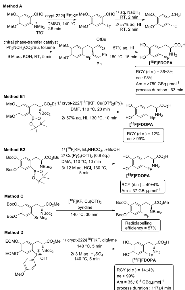
Figure 1. n.c.a. radiosyntheses of [ 18 F]FDOPA according to Lemaire et al. [7] (method A), Tredwell et al. [6a] (method B1), Zischler et al. [6b] (method B2), Makavarage et al. [10] (method C) and Kuik et al. [11] (method D).
