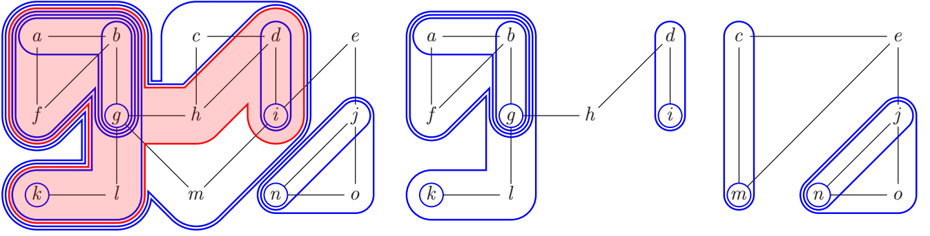
FIGURE 20. The red tube \mathfrak{t}_{\text{ex}}^\circ = \{a, b, d, f, g, h, i, k, l\} in the maximal tubing \mathbb{T}^\circ (left) yields a maximal tubing \mathbb{T}_{\text{ex}}^\circ[\mathfrak{t}_{\text{ex}}^\circ] on the restriction G_{\text{ex}}[\mathfrak{t}_{\text{ex}}^\circ] (middle) and a maximal tubing \mathbb{T}_{\text{ex}}^\circ \star \mathfrak{t}_{\text{ex}}^\circ on the reconnected complement G_{\text{ex}} \star \mathfrak{t}_{\text{ex}}^\circ (right).
