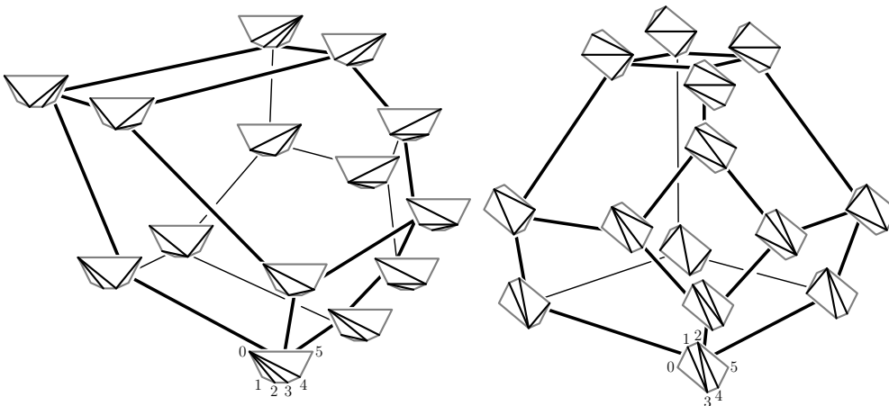
FIGURE 1. Two polytopal realizations of the 3-dimensional associahedron with vertices labeled by triangulations of convex hexagons described in [HL07].
