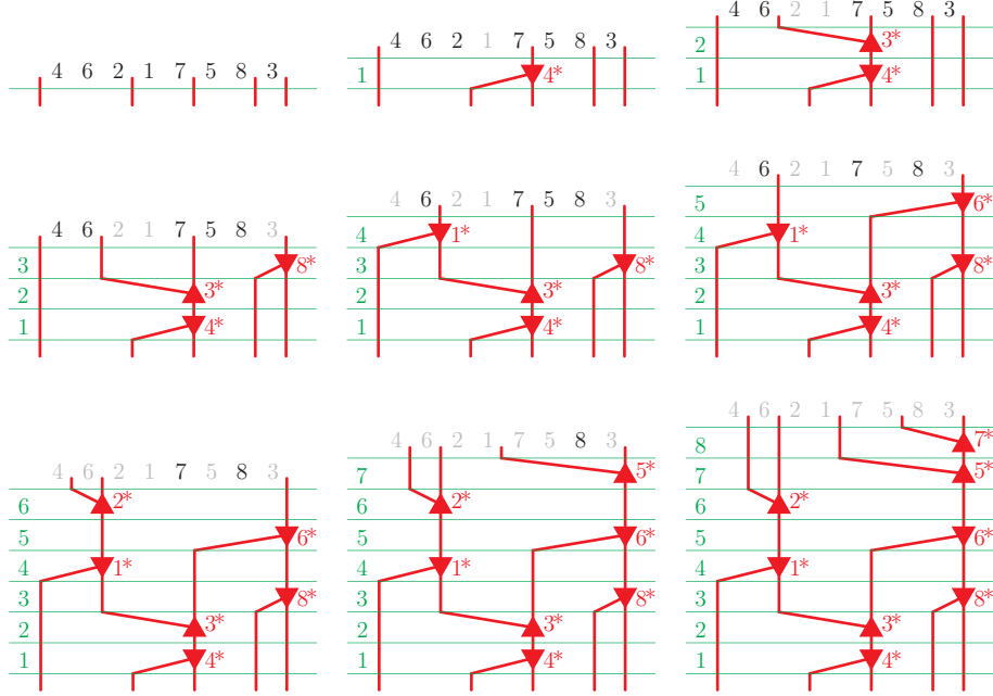
FIGURE 8. The construction of the leveled spine \kappa(\sigma^{\text{ex}})^{\circledast} for \sigma^{\text{ex}} = [4, 6, 2, 1, 7, 5, 8, 3] .
