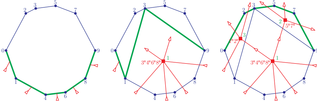
FIGURE 9. The sequence of paths \pi_0(\tau^{\text{ex}}), \pi_1(\tau^{\text{ex}}), \pi_2(\tau^{\text{ex}}) for \tau^{\text{ex}} = [2, 2, 1, 1, 2, 1, 2, 1] .
