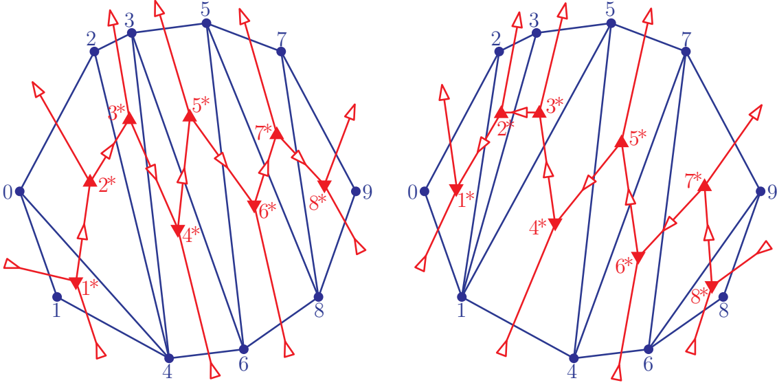
FIGURE 6. The source \underline{T}(\mathbf{P}^{\text{ex}}) and the sink \overline{T}(\mathbf{P}^{\text{ex}}) of the slope increasing flip graph \mathcal{G}(\mathbf{P}^{\text{ex}}) .
