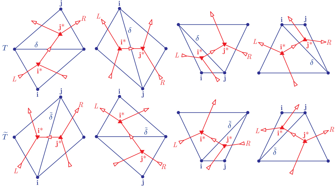
FIGURE 5. The four possible configurations of a square. Triangulations in the same column relate by a flip.
