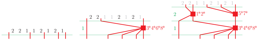
FIGURE 10. The construction of the leveled spine \kappa(\tau^{\text{ex}})^{\otimes} for \tau^{\text{ex}} = [2, 2, 1, 1, 2, 1, 2, 1] .
