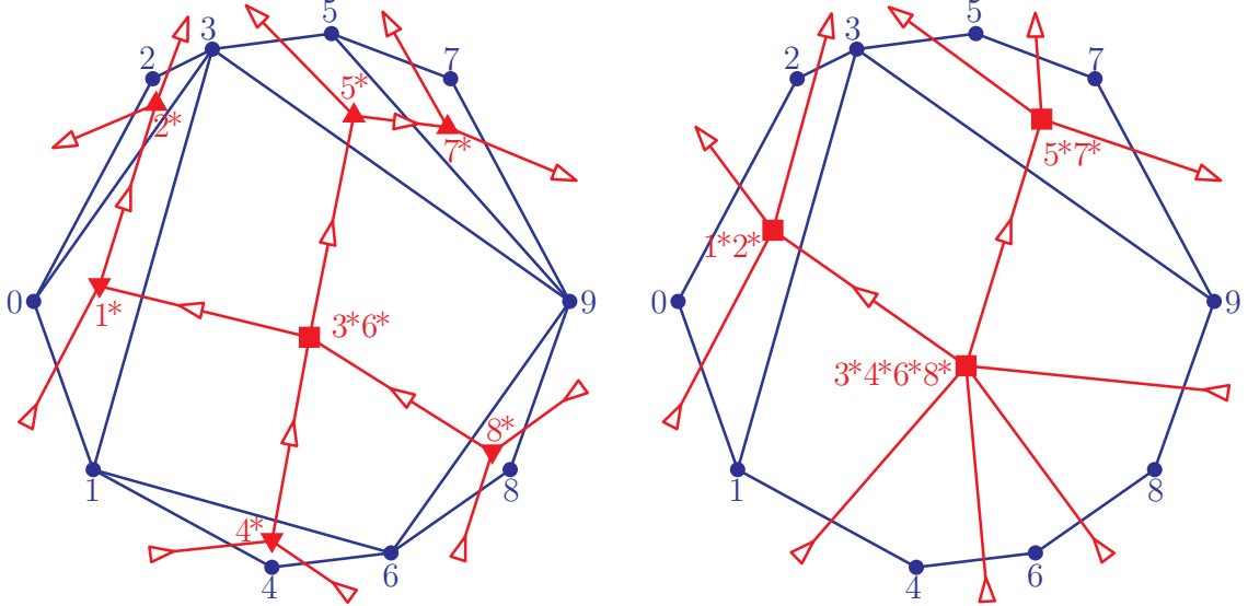
FIGURE 4. Two dissections W^{\text{ex}} and \widetilde{W}^{\text{ex}} of the polygon \mathbf{P}^{\text{ex}} and their spines.
