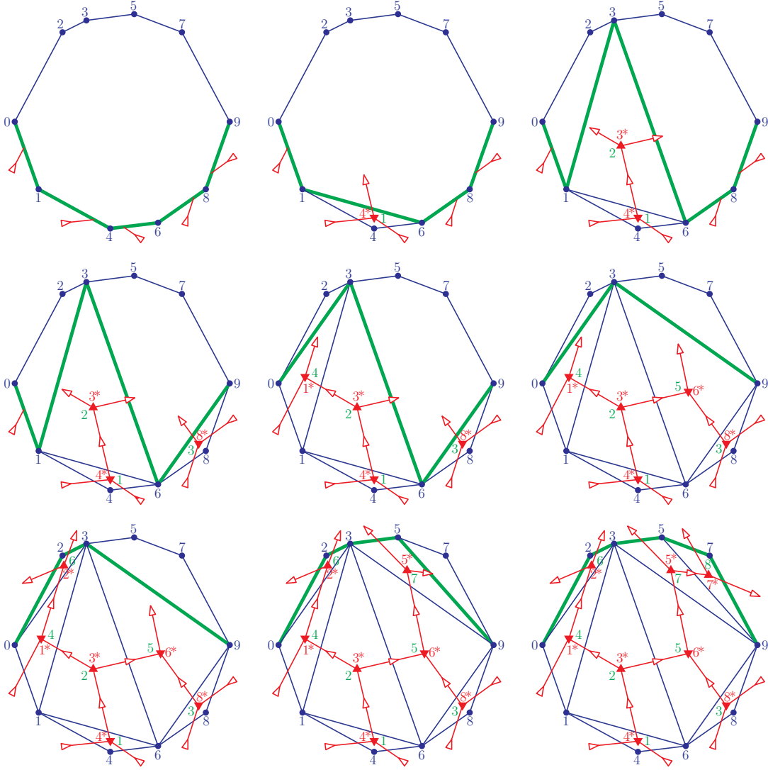
FIGURE 7. The sequence of paths \pi_0(\sigma^{\text{ex}}), \pi_1(\sigma^{\text{ex}}), \dots, \pi_8(\sigma^{\text{ex}}) for \sigma^{\text{ex}} = [4, 6, 2, 1, 7, 5, 8, 3] .
