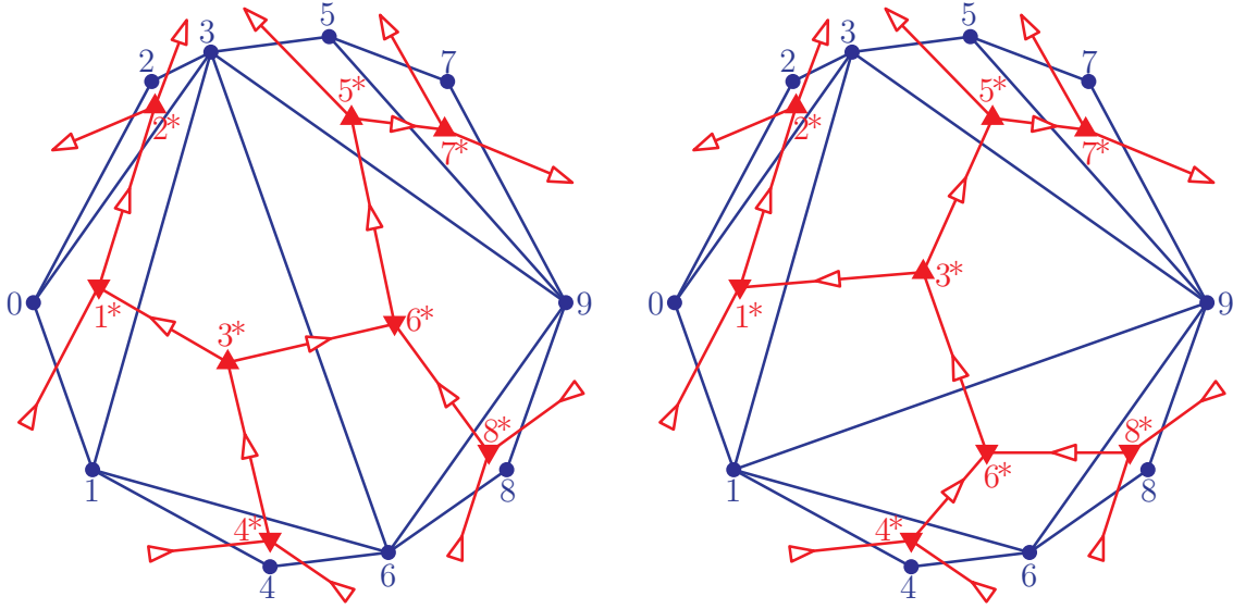
FIGURE 2. Two triangulations T^{\text{ex}} and \tilde{T}^{\text{ex}} of the polygon \mathbf{P}^{\text{ex}} and their spines.
