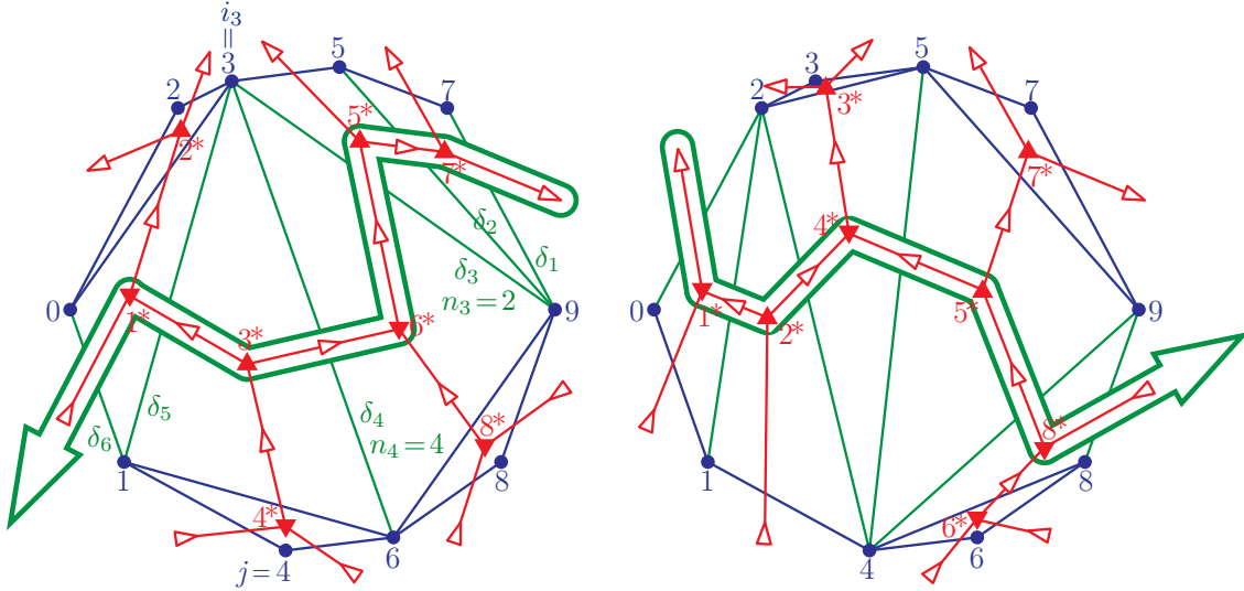
FIGURE 11. A maximal path \pi in the spine of the triangulation T^{\text{ex}} of Figure 2 (left). Considering the down label j = 4 , we have k = 3 and i_k = 3 is to the right of \pi . Therefore, the combinatorial rotation of the triangulation T^{\text{ex}} which sends vertex 3 to vertex 4 sends \pi to a path with two incoming arcs at 4^* .
