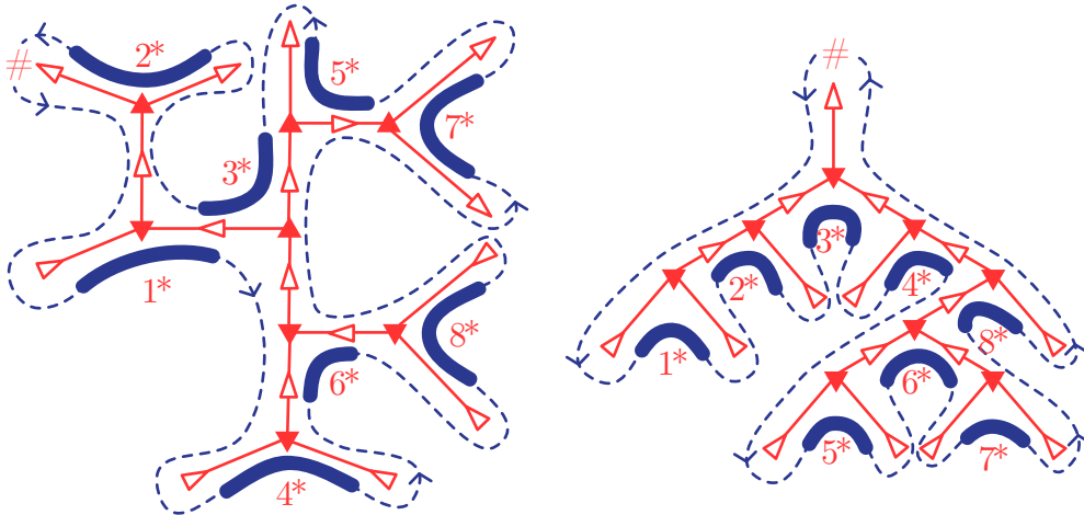
FIGURE 3. Traverse in counter-clockwise direction around the unlabeled tree of spine \tilde{T}^{\text{ex}} starting at blossom \# to reconstruct the inner node labels (left). The procedure specializes to inorder search labeling of binary trees (right).
